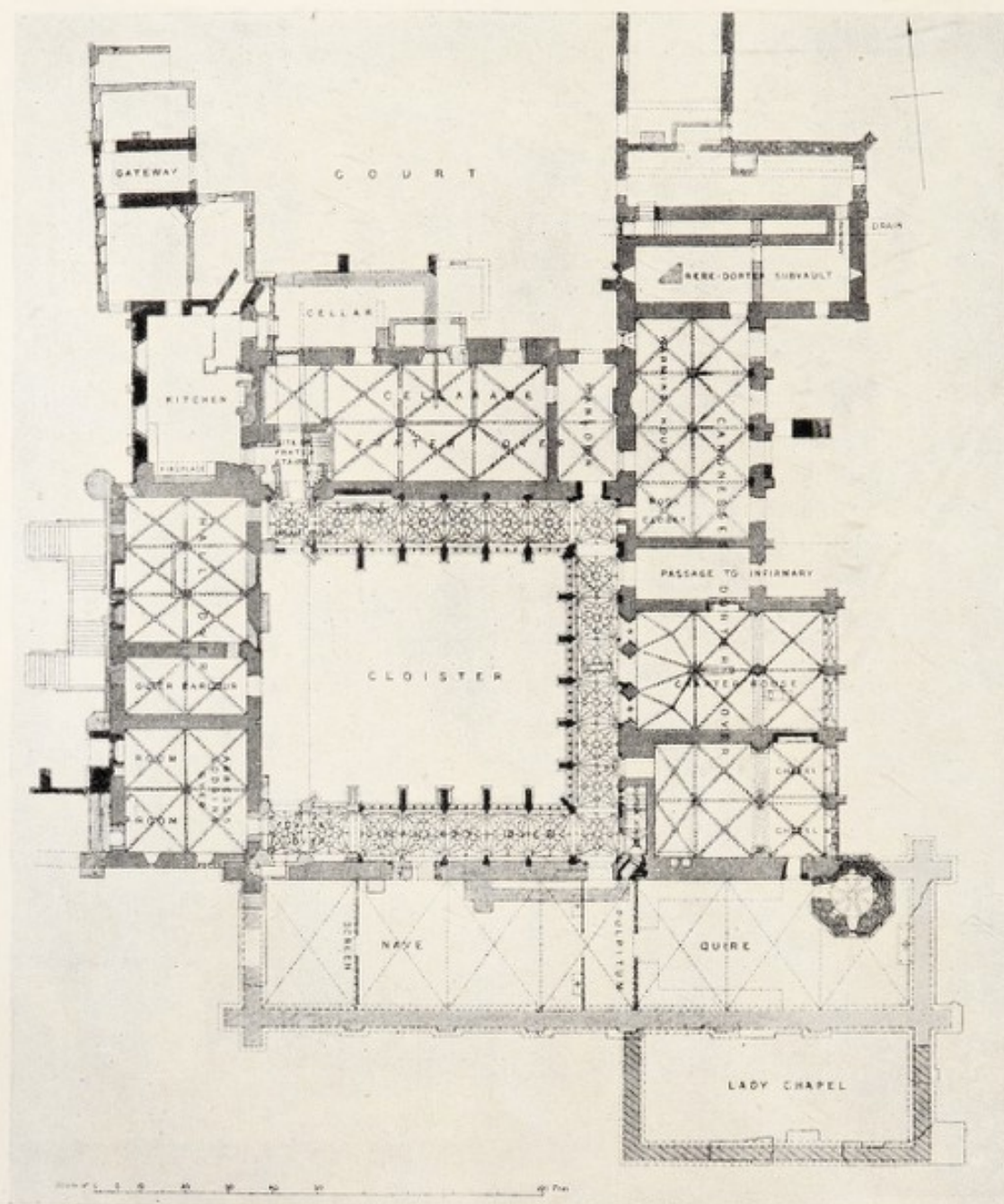
PLAN OF LACOCK ABBEY
