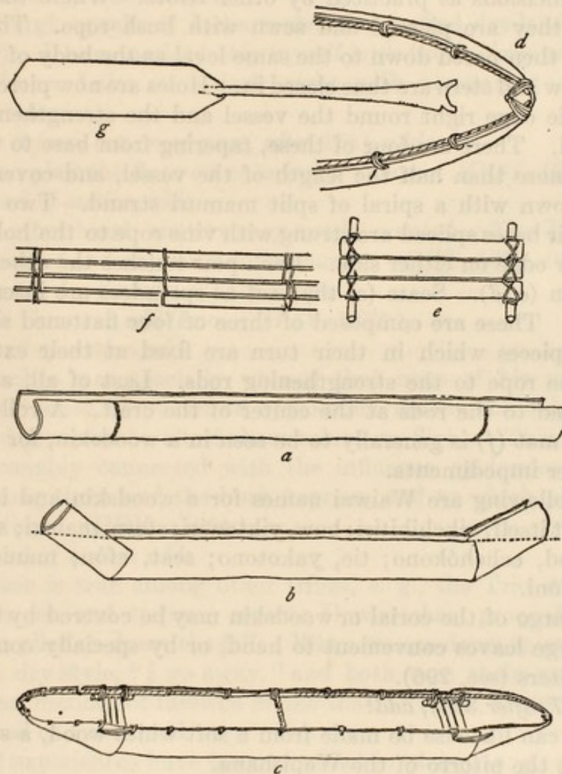
FIGURE 90.—Manufacture of the Waiwai woodskin. (Sec. 798 A)
