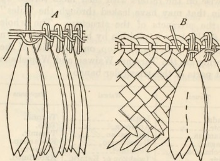
FIGURE 15.—Rain shelters for protecting boat cargoes. (Sec. 296.) A, Dalibanna leaves on two turu-palm laths (Wapishana, Taruma). B, Dalibanna leaves on plaited spinous-palm leaves (Taruma, Waiwai)
