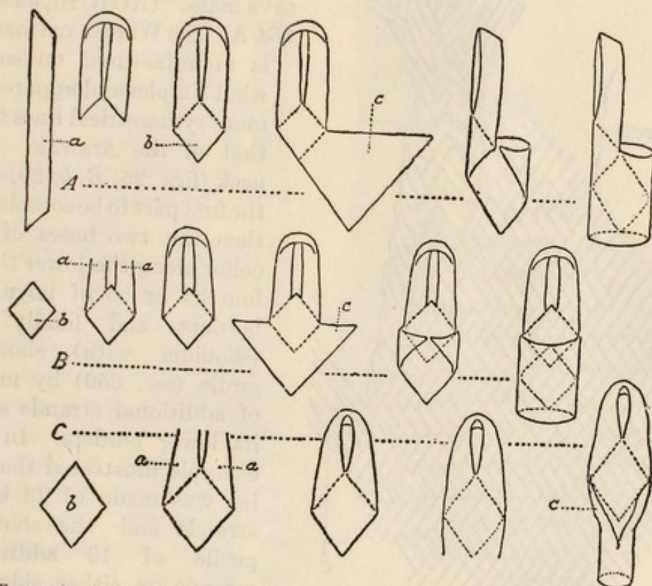
FIGURE 25.—Diagram to show variations in the commencing stages of the manufacture of a cassava squeezer. (Sec. 354 A.) A, Arawak; B, Wapishana; C, Taruma, Waiwai. a, Collar; b, neck; c, shoulder
