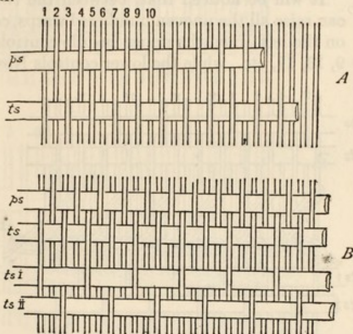
FIGURE 61.—Manufacture of a 6-weft Atorai hammock. (Sec. 473 A.) A, The first two wooden slips ( ps , ts ) picking up strings 2, 4, 6, 8, 10, etc., and 1, 3, 5, 7, 9, etc., respectively. B, The second two wooden slips ( ts I , ts II ) picking up strings 1, 5, 9, 13, 17, etc., and 3, 7, 11, 15, 19, etc., respectively
