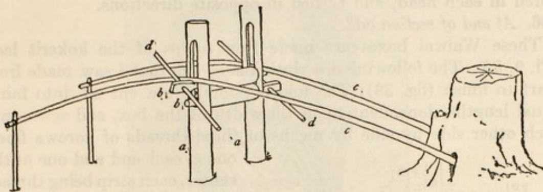
FIGURE 32.—Roller press for squeezing sugar cane, upper Barama River. (Sec. 383.) a, a, Upright posts with slits in which to rest the two rollers b, b. These are pressed together by the saplings c, c, and turned in opposite directions by the handles d, d
