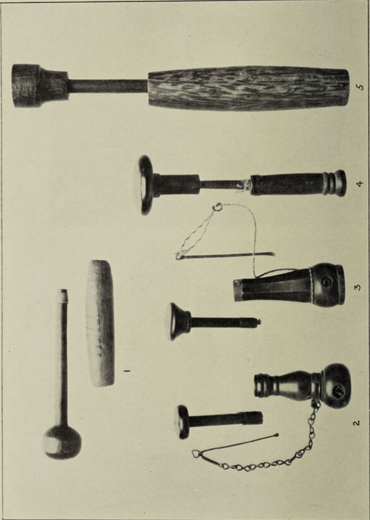
FIRE PISTONS FOR IGNITING TINDER BY AIR COMPRESSION 1, Siam; 2, Lower Siam; 3, Philippine Islands; 4, Philippine Islands; 5, Java
