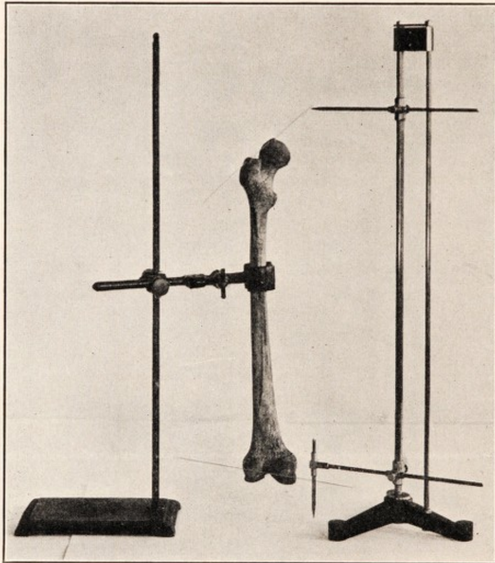
FIG. 11.—Parallelograph of Martin. ( Manufactured by Hermann; Zürich. )
