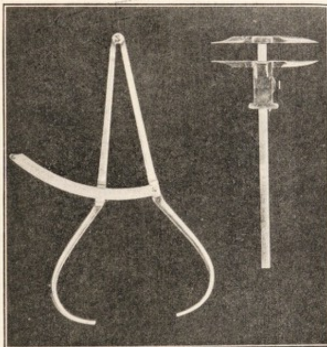
FIG. 1.—Two common instruments. ( Made by Hermann, Zürich. ) (The one on the left) Calipers [Fr. compas d'épaisseur ; Ger. Tasterzirkel .] (The one on the right) Slide compass [Fr. compas glissière ; Ger. Gleitzirkel .]
