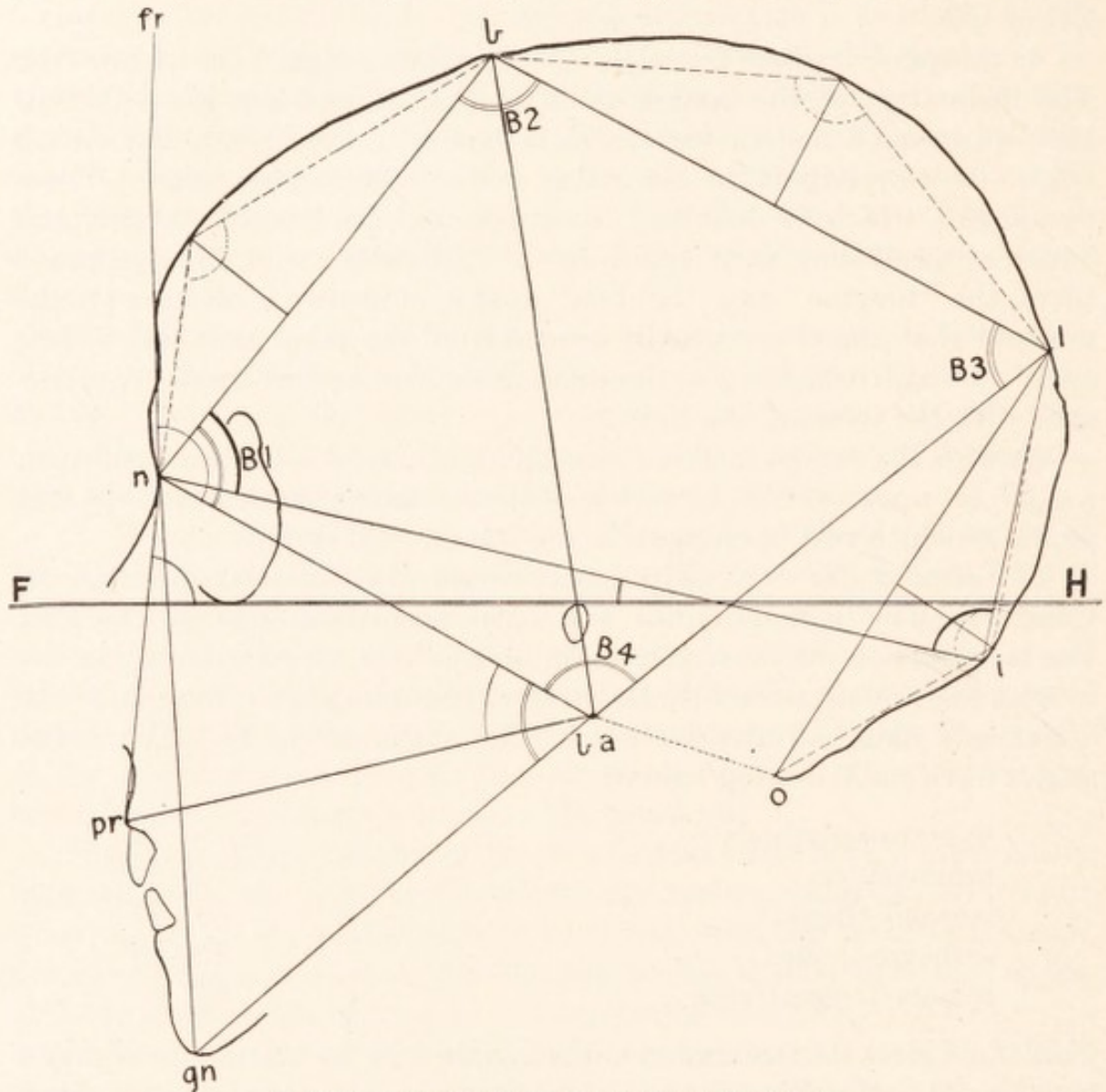
FIG. 27.—Diagram illustrating cranial angles.
