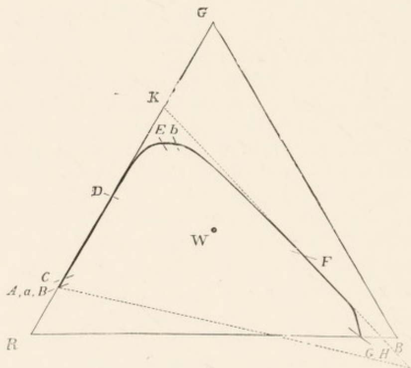
FIG. 3.—Spectrum Curve in the Colour Triangle.
