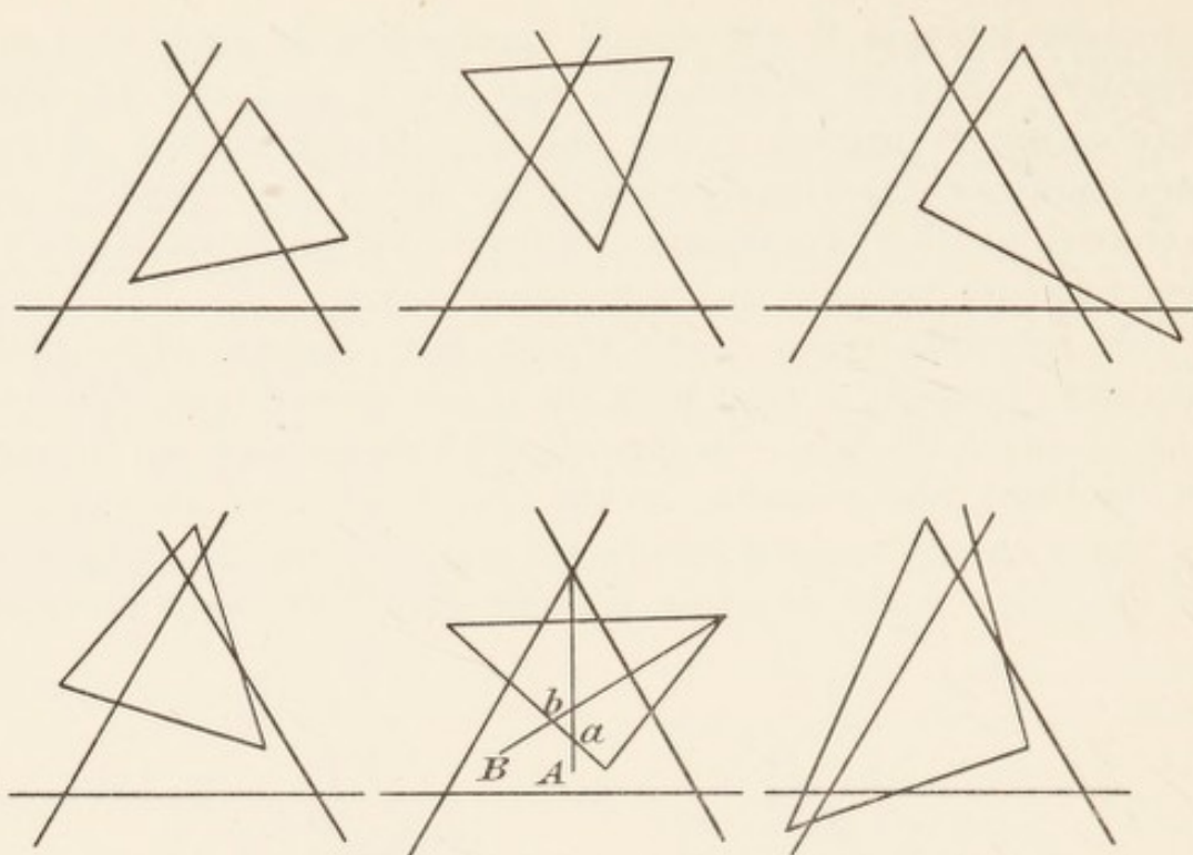
FIG. 6.—Derived Colour Triangles. Class III.
