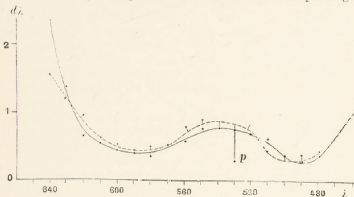
FIG. 20.—Helmholtz's Differential Sensitivity Curve.
