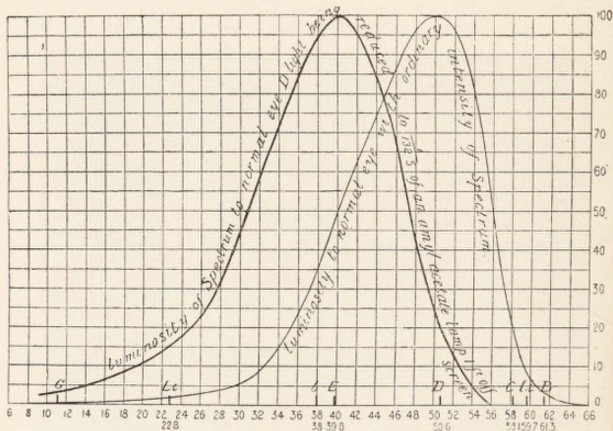
FIG. 17.—Curves of Strong and Weak Luminosity.
