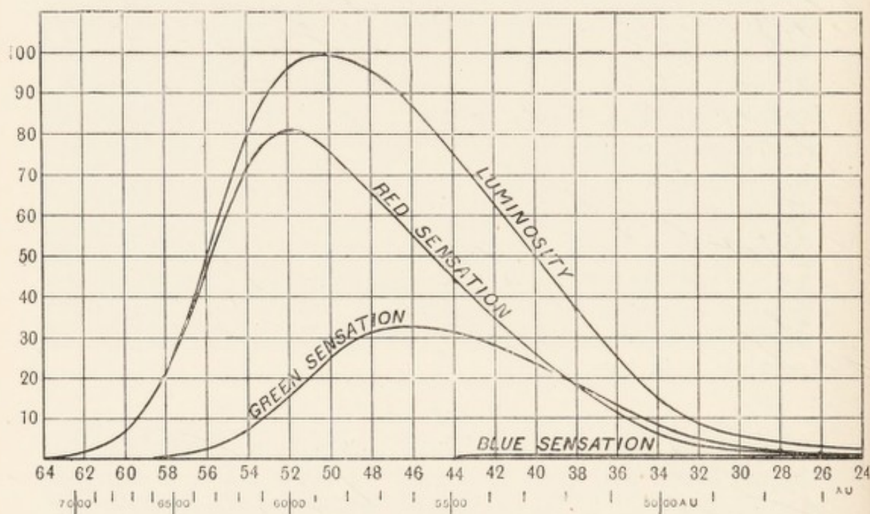
FIG. 14.—Sensation Curves (by Luminosity).
