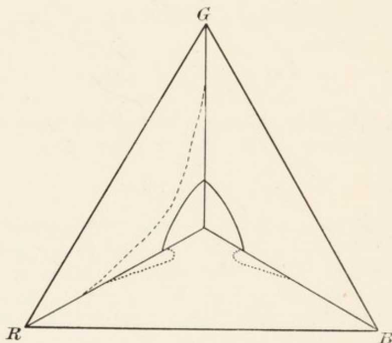
FIG. 24.—The Spectrum Curve in the Colour Diagram.
