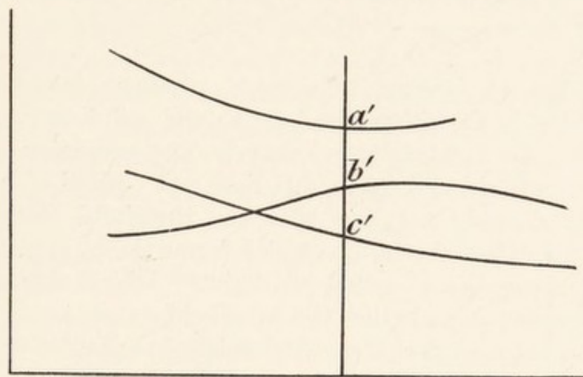
FIG. 19.—Test for Colour Sensitivity.
