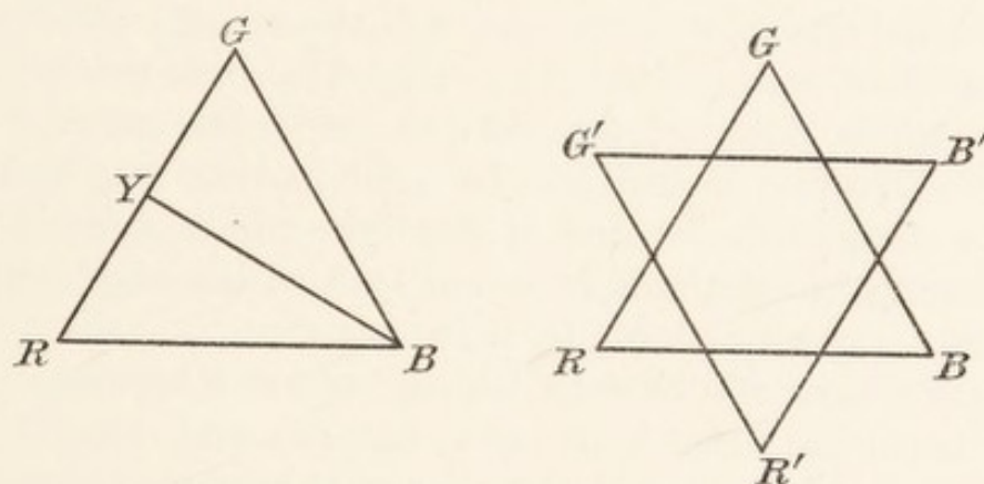
FIG. 9.—Special Derived Colour Triangles.
