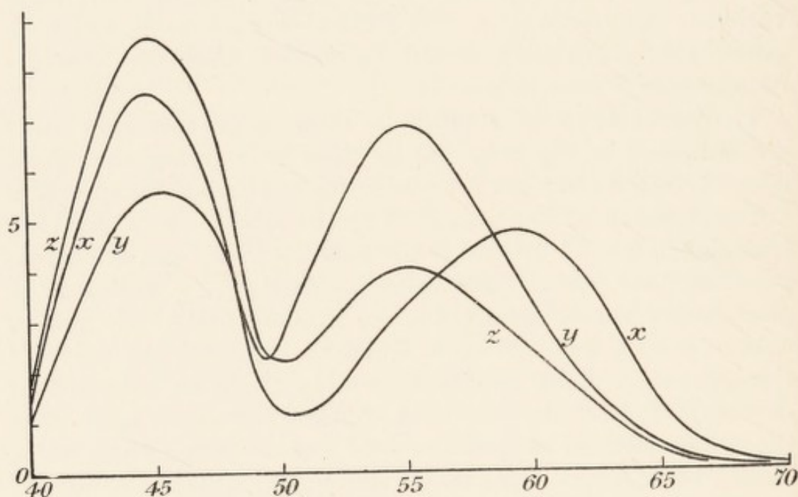
FIG. 8.—Spectrum Stimuli in Helmholtz's Absolute Triangle.
