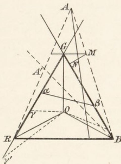
FIG. 11.—The Dichromatic Colour Triangle.
