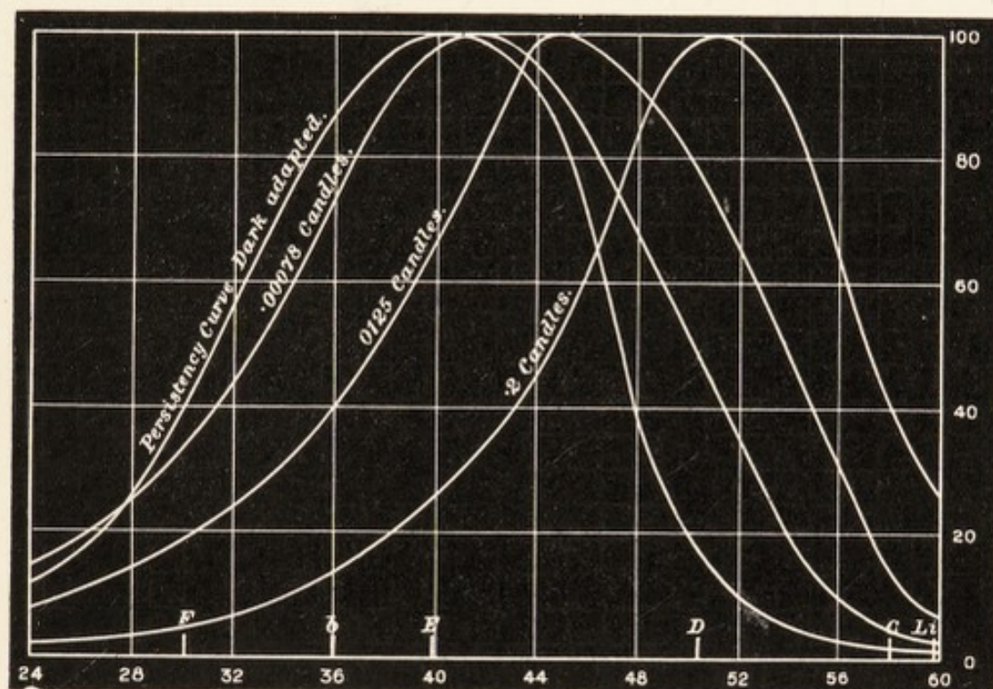
FIG. 16.—Persistency Curves.
