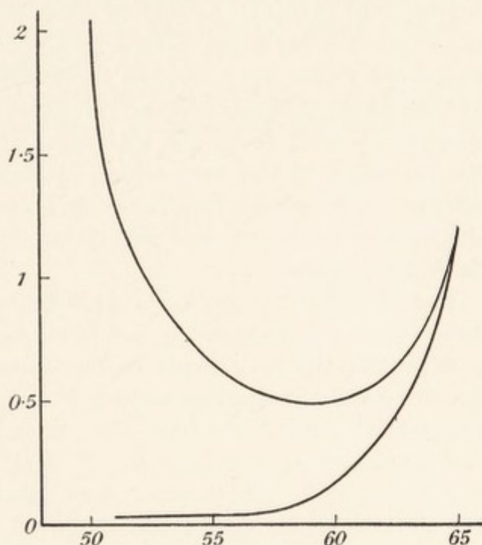
FIG. 26.—Threshold Values deduced from Ives' Curves.
