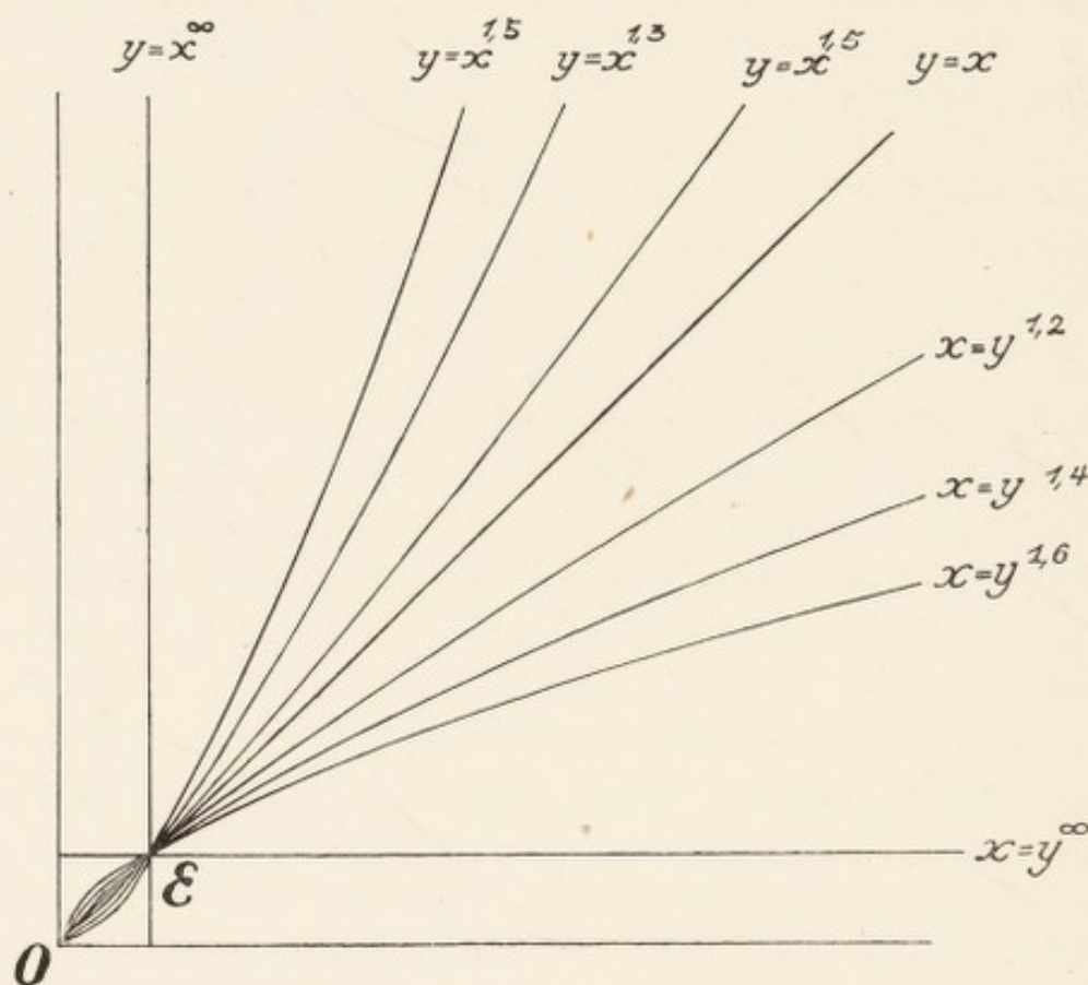
FIG. 10.—Shortest Colour Lines.
