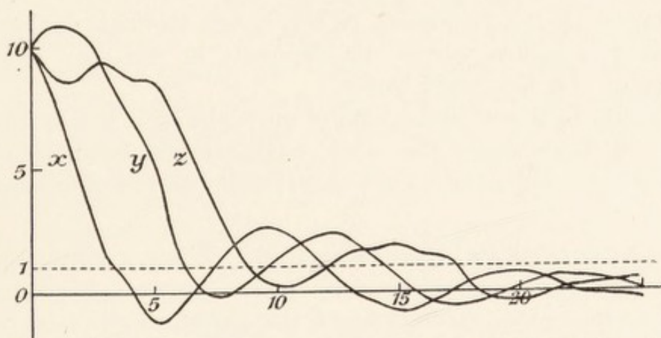
FIG. 29.—Oscillating After Images with Initial White Sensation.
