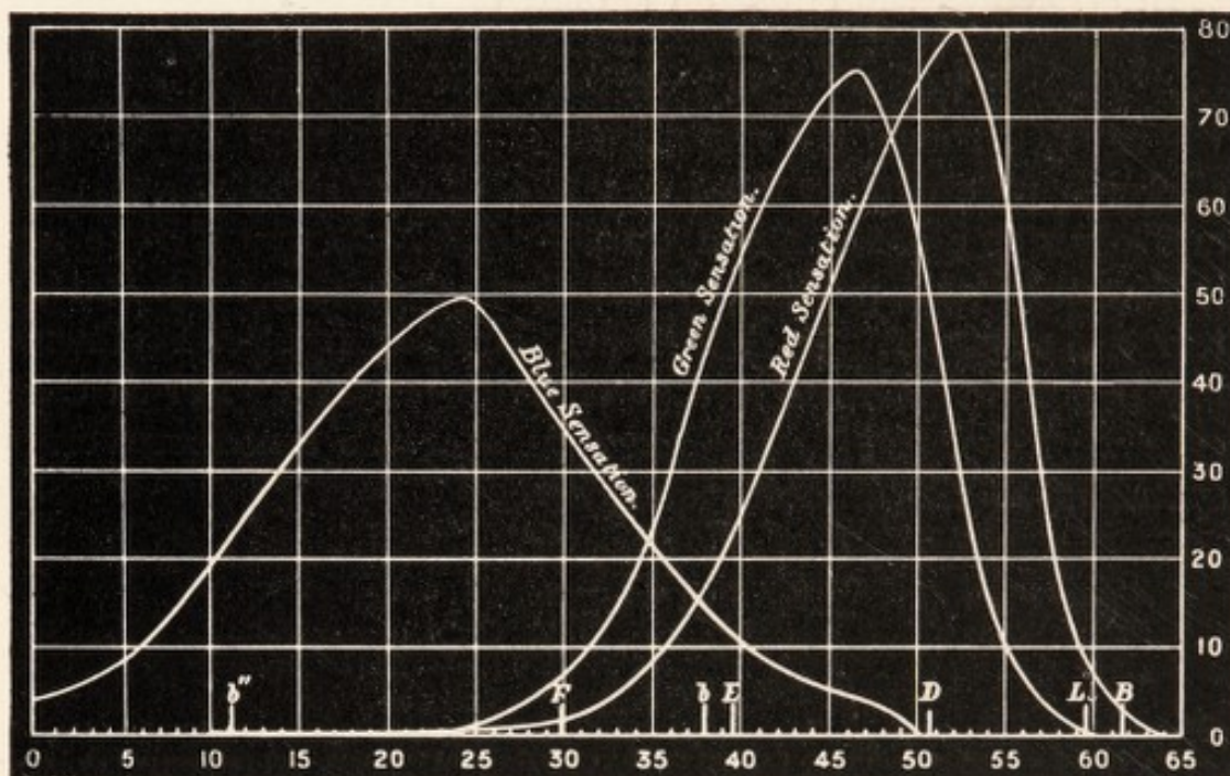
FIG. 13.—Sensation Curves (Equal Area).
