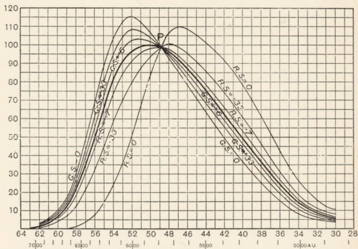
FIG. 15.—Theoretical Luminosity Curves.
