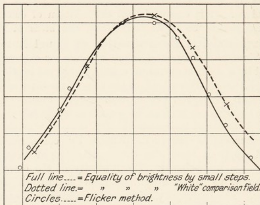
FIG. 12.—Luminosity Curves.
