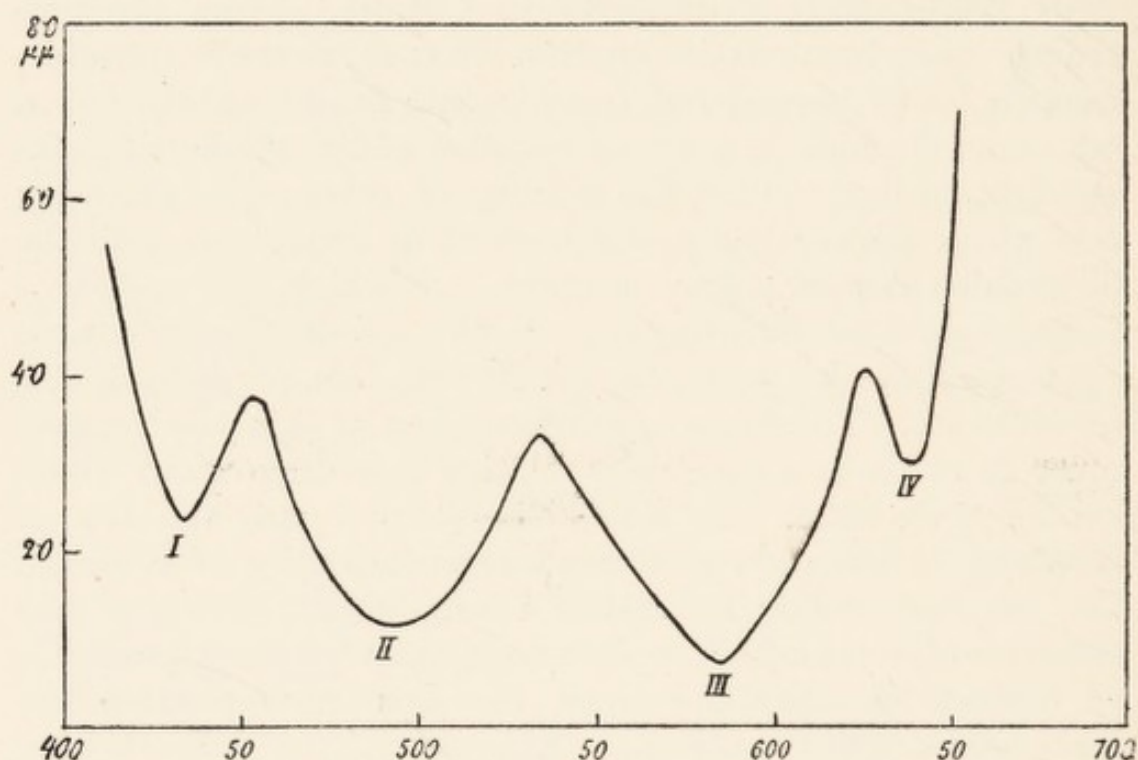
FIG. 18.—Curve of Differential Sensitivity.
