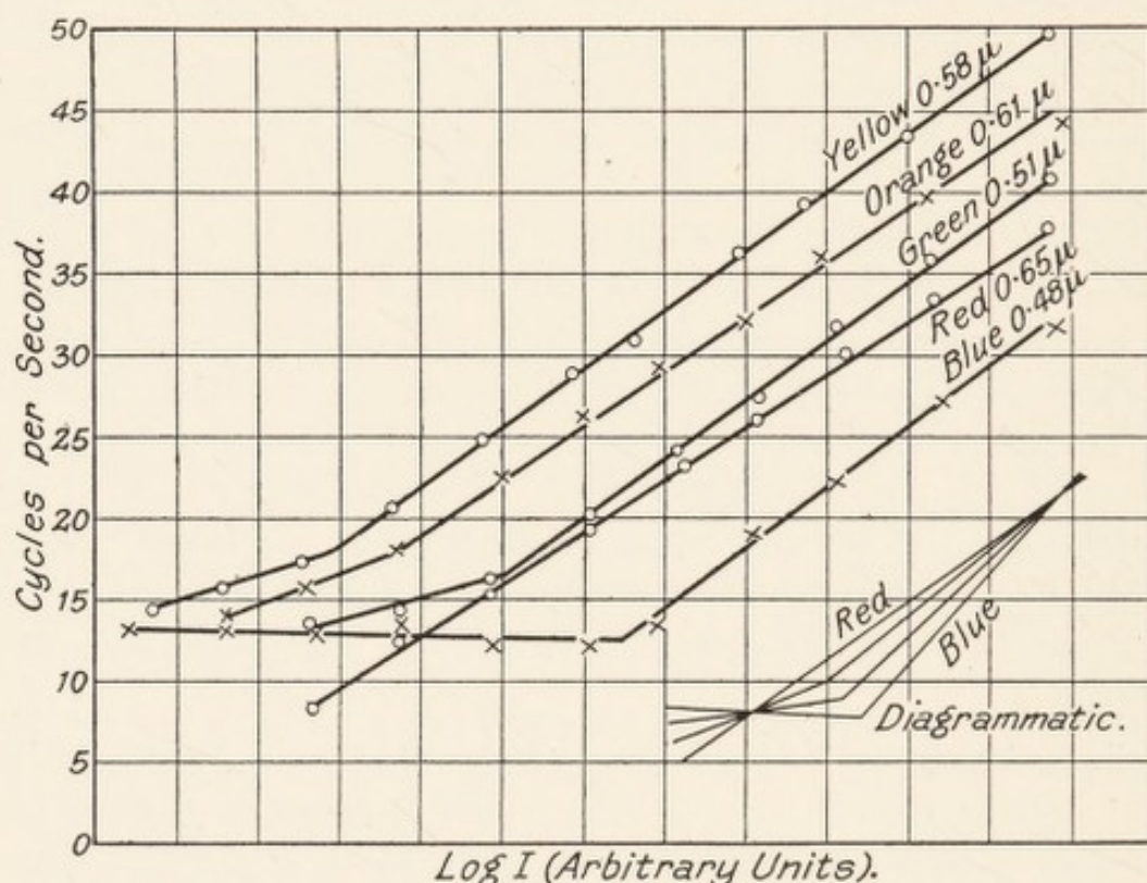
FIG. 25.—Curves of Critical Flicker Frequency and Intensity.
