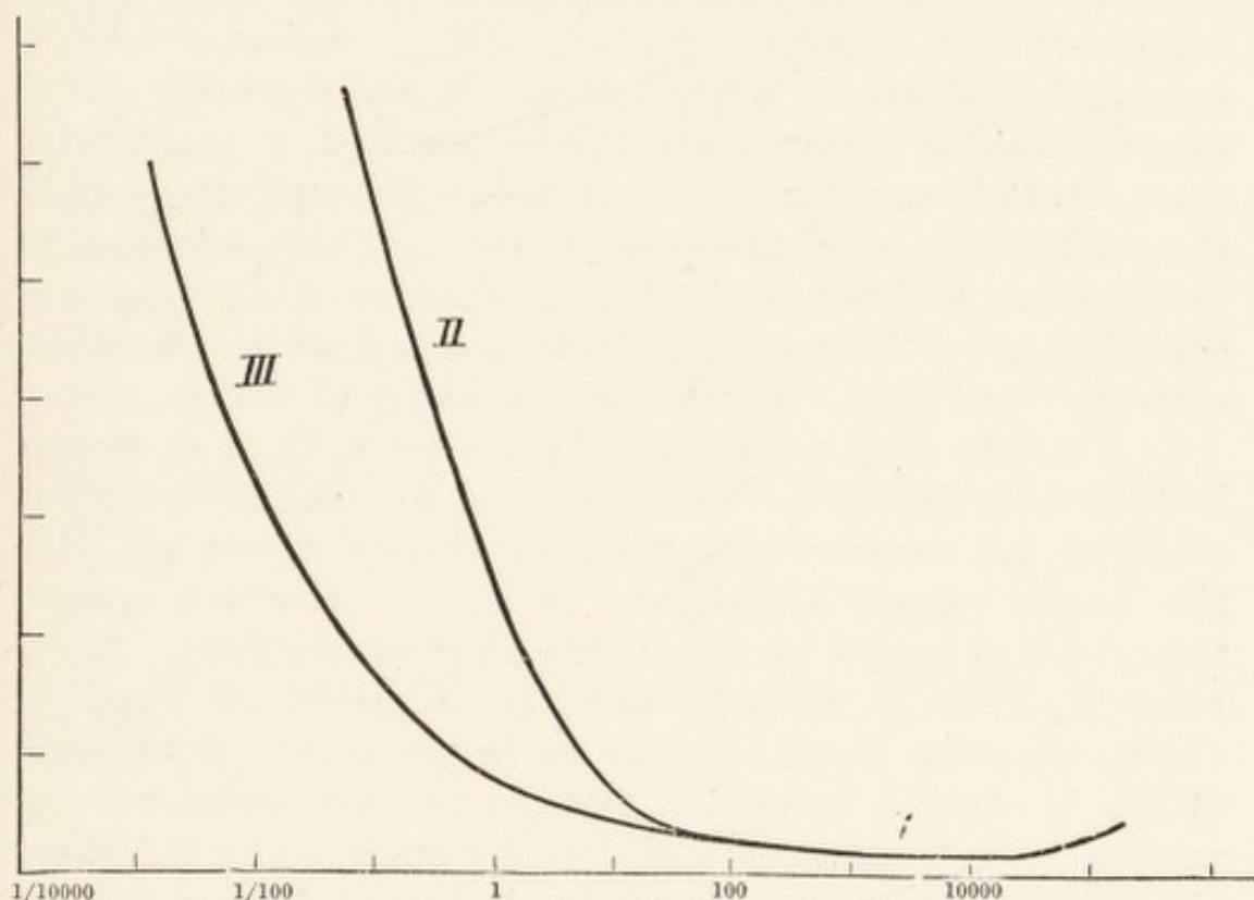
FIG. 1.—Change of Sensation with Intensity of Illumination.
