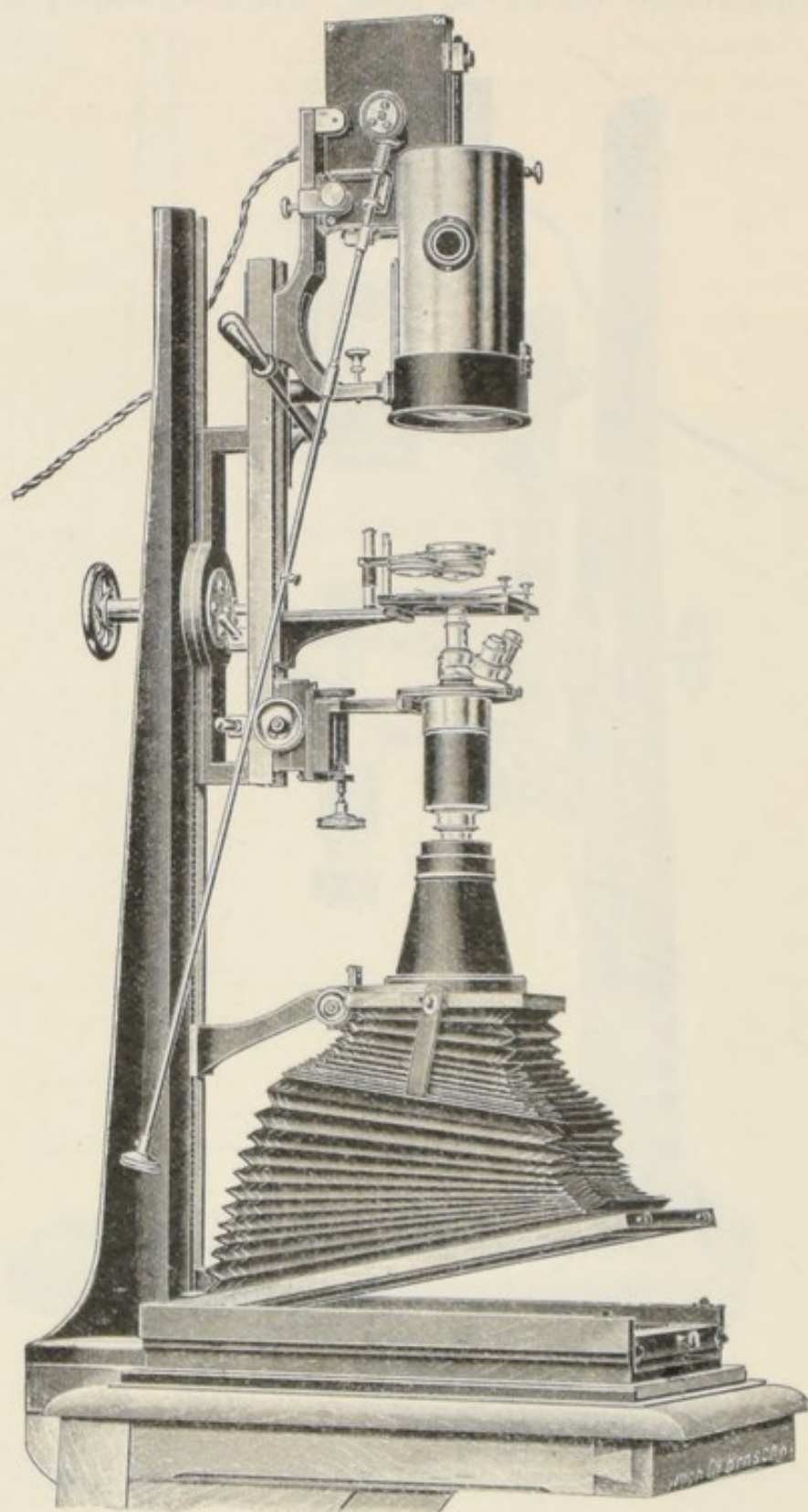
FIG. 236.—Edinger's drawing apparatus with attachment for photo-micrography.
