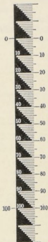
FIG. 208.— Scale of step micrometer.
