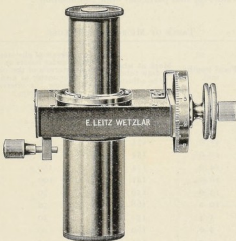
FIG. 207.—Screw micrometer eyepiece (Filar micrometer).
