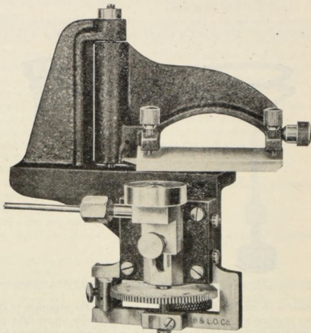
FIG. 232.—Clinic microtome with freezing attachment.
