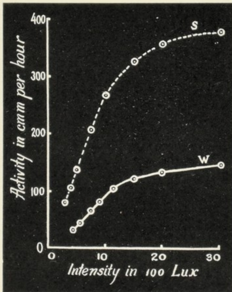
FIG. 7. Photosynthetic Curves under Increasing Intensity of Light, for Spring-specimen s, and for Winter-specimen w
