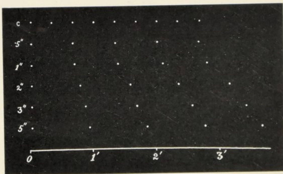
FIG. 27. The Effect of Intermittent Light on Photosynthetic Activity
