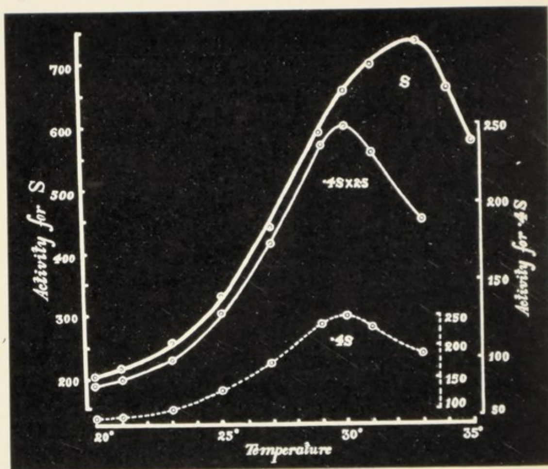
FIG. 60. Photosynthetic Curves under Variation of Temperature carried through a Cycle at Intensity of Light S (upper curve), and at Intensity 0.4 S (dotted curve). The middle curve is obtained by multiplying the activities under 0.4 S by 2.5 , which is the ratio of the two intensities S and 0.4 S (see text).
