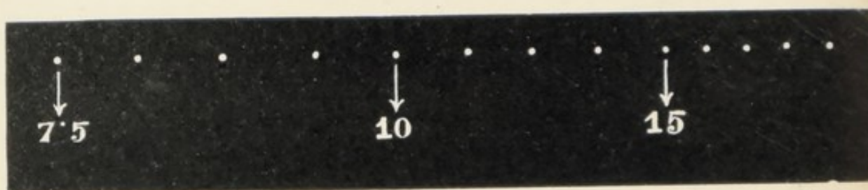
FIG. 6. Records showing the periods of physiological adjustment under rapid change from 750 to 1000, and then to 1500 lux (7.5, 10 and 15 units)
