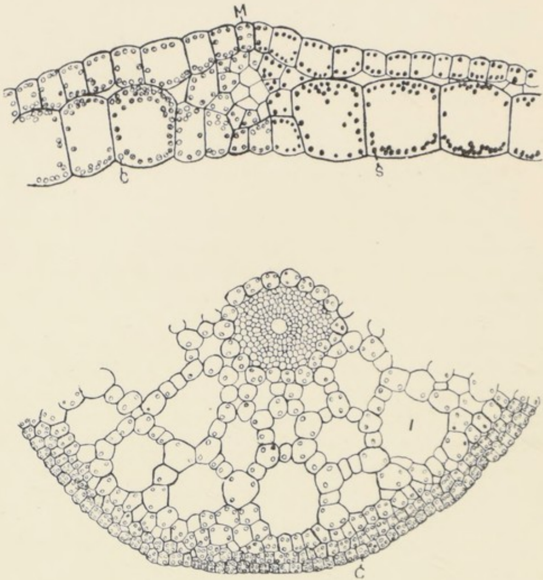
FIG. 1. Transverse Section of the Leaf (upper figure), and of the Stem (lower figure) of Hydrilla verticillata
