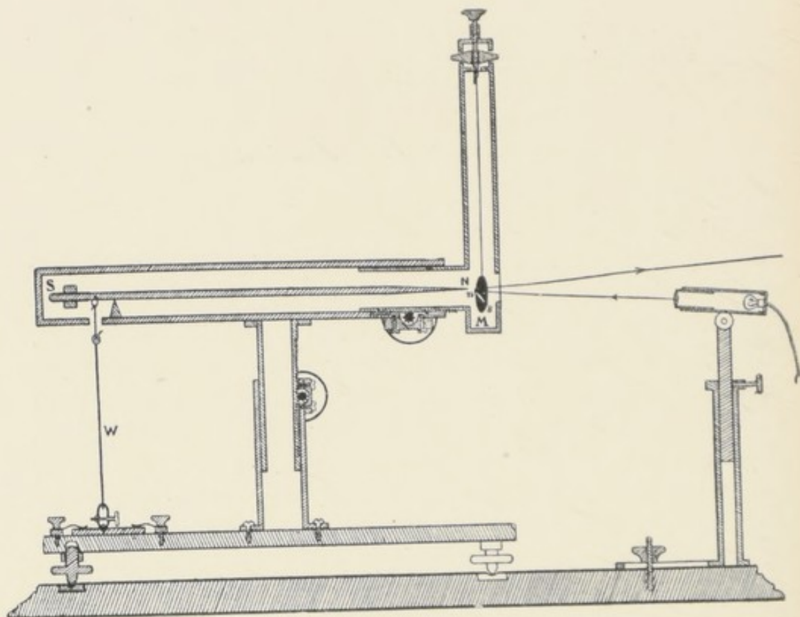
FIG. 49. The Magnetic Radiometer
