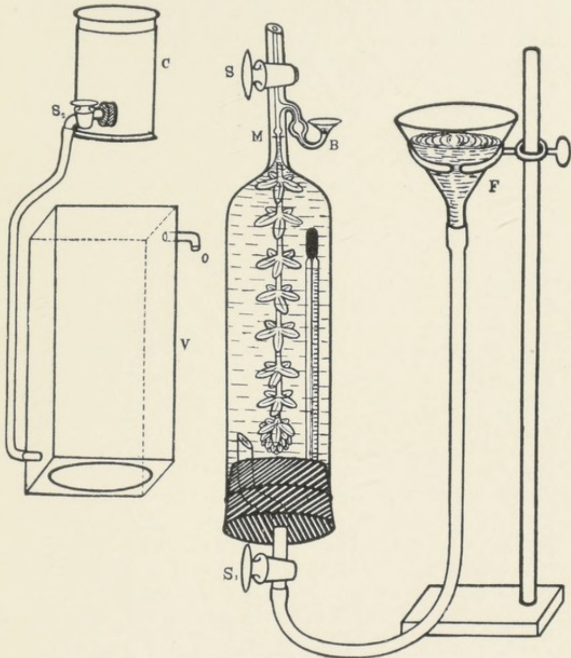
FIG. 37. Arrangement for Variation of Temperature. The Plant-vessel with Bubbler seen to the right; outer enclosing Vessel v seen to the left
