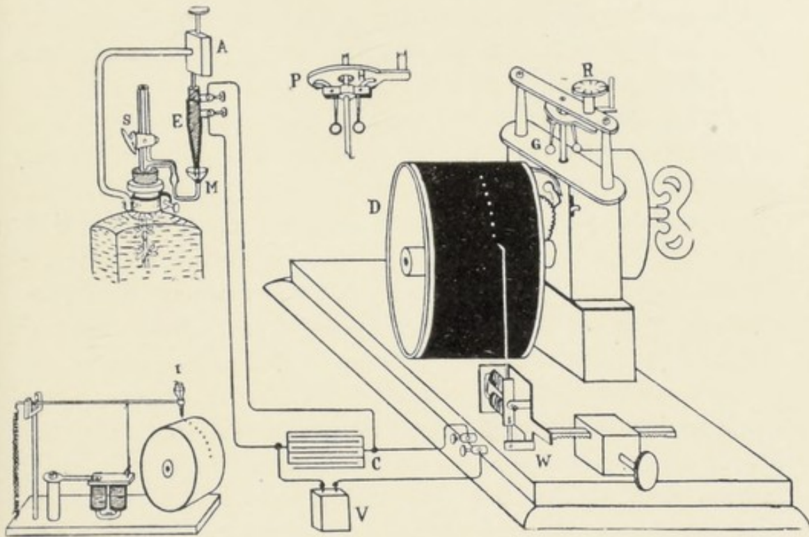
FIG. 3. The Automatic Recorder for Photosynthesis
