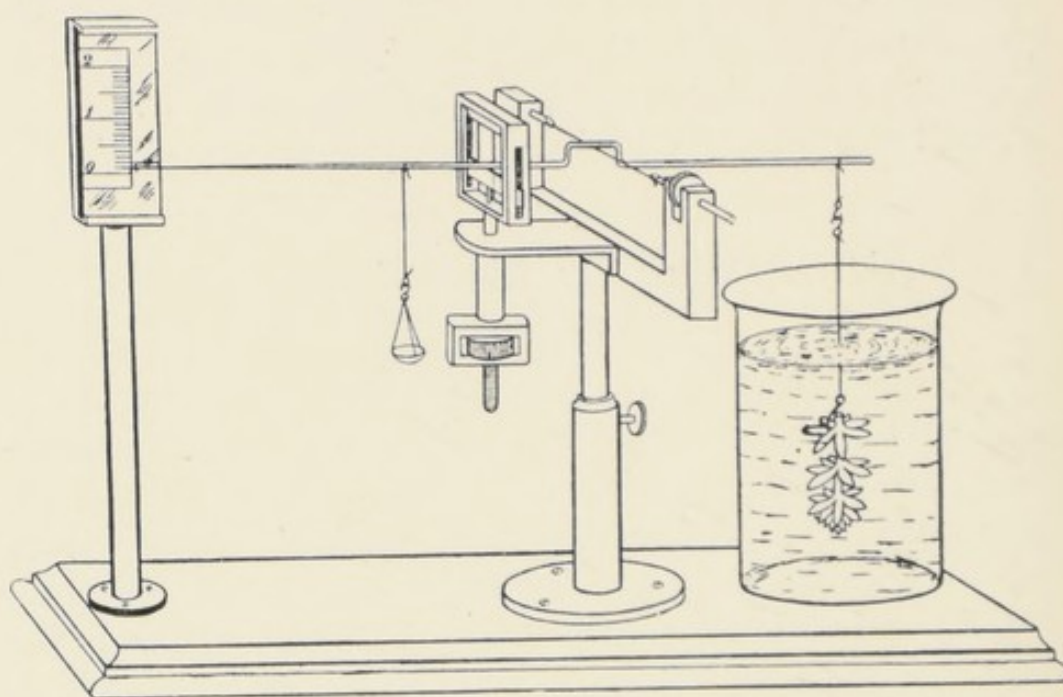
FIG. 52. The Torsion Balance for Measurement of Increase of Weight of the Living Plant during Photosynthesis
