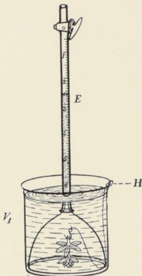
FIG. 54. Eudiometer E for collection of Oxygen evolved under Light v_1 , second vessel ; H , suspending hook.
