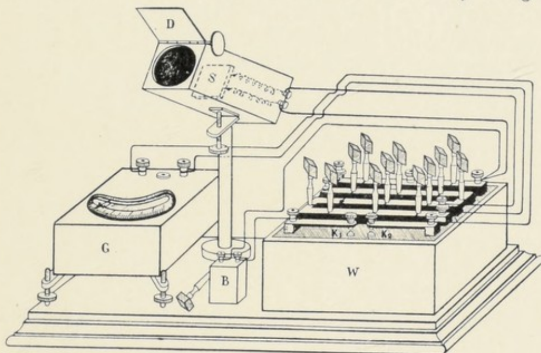
FIG. 32. The Portable Electric Photometer
