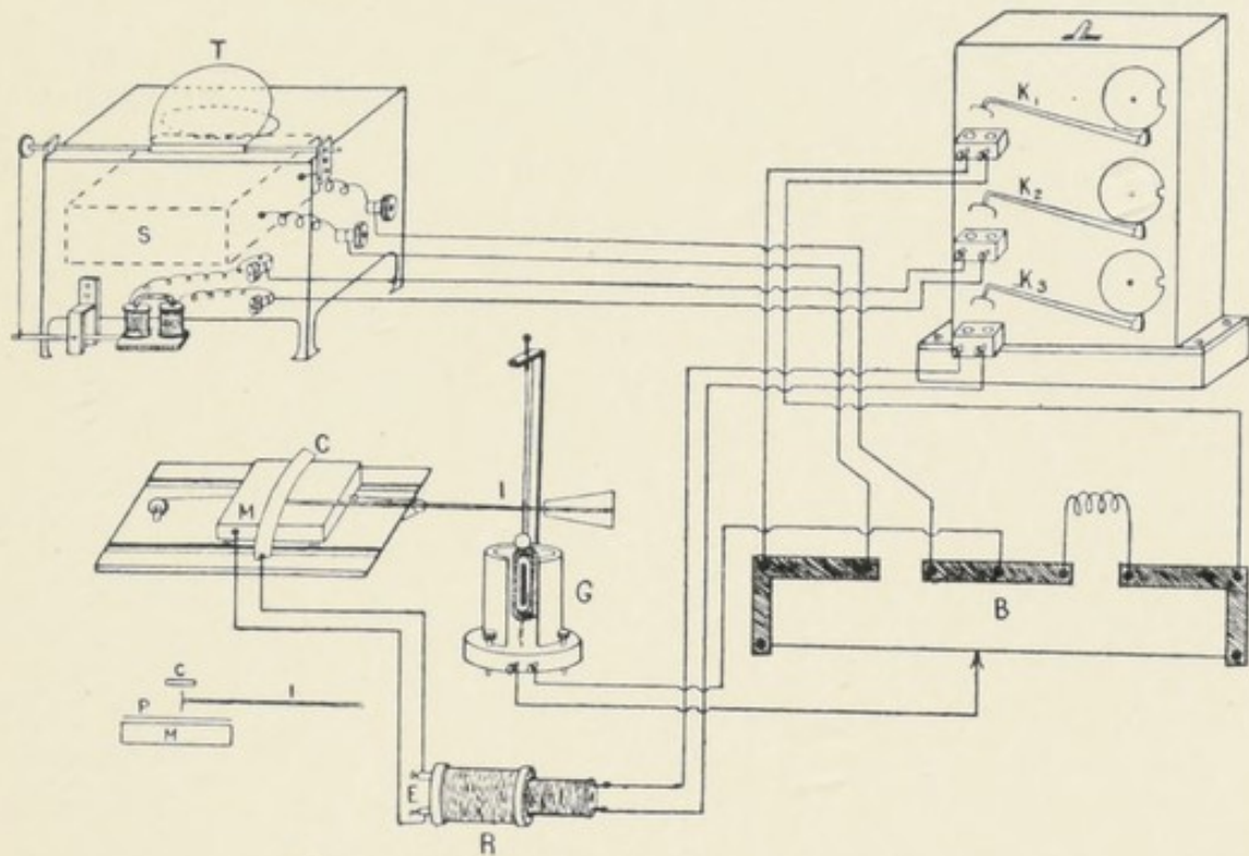
FIG. 29. The Self-recording Radiograph
