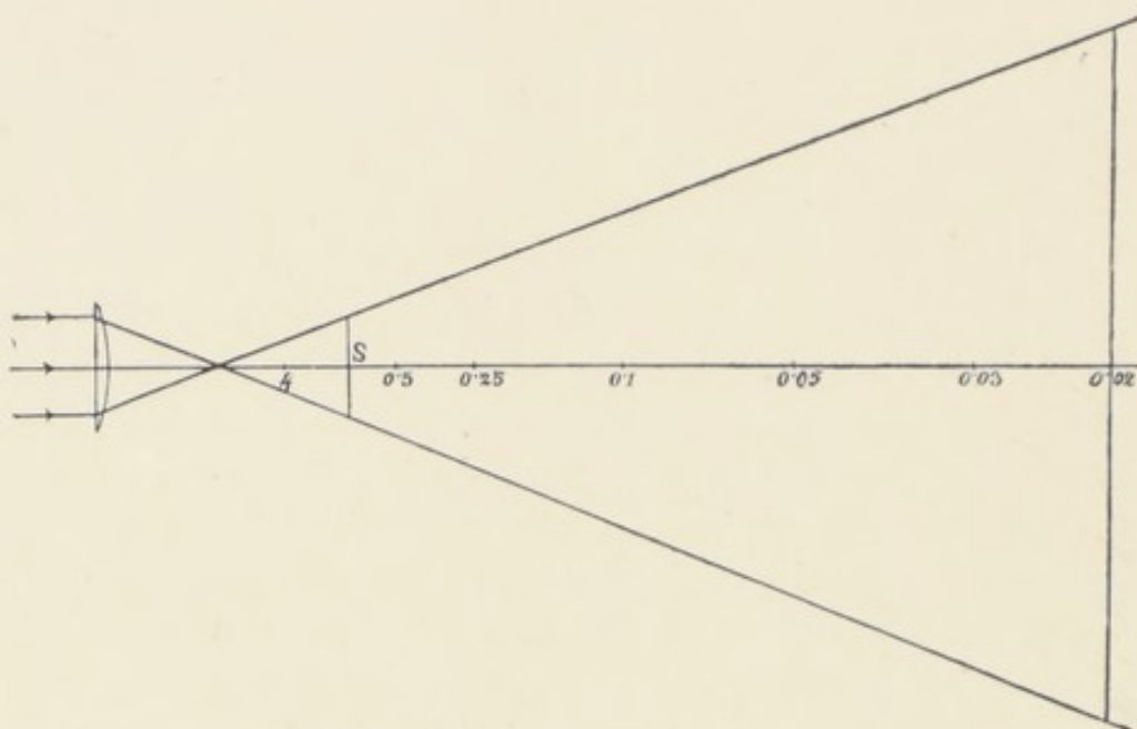
FIG. 5. Diagrammatic Representation of Arrangement for securing different intensities of Light
