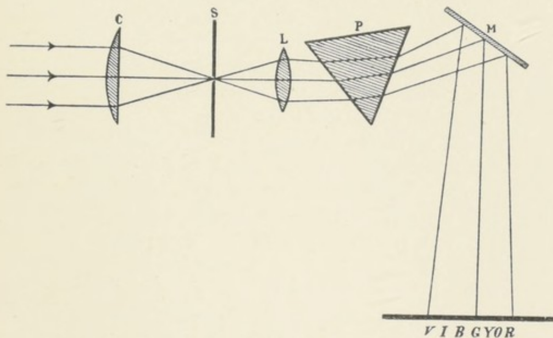
FIG. 48. Arrangement for obtaining a Pure Solar Spectrum
