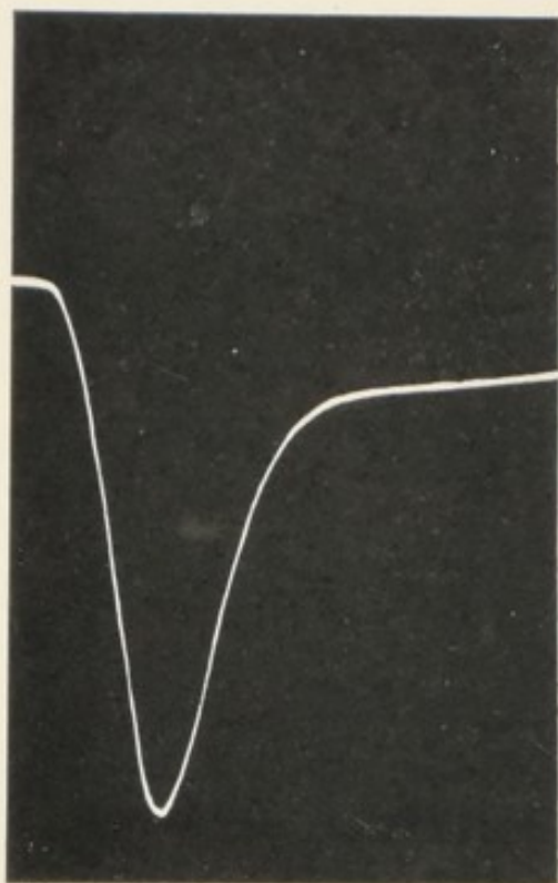
FIG. 21. The Positive Electric Response of Hydrilla
