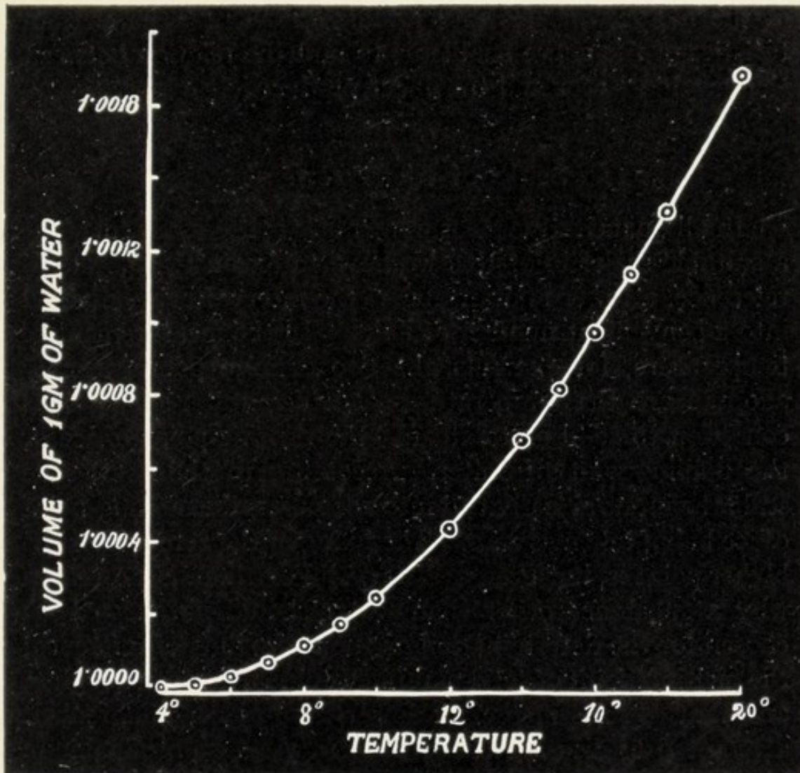
FIG. 56. Curve showing the Change of Volume of 1 Grm. of Water at different temperatures
