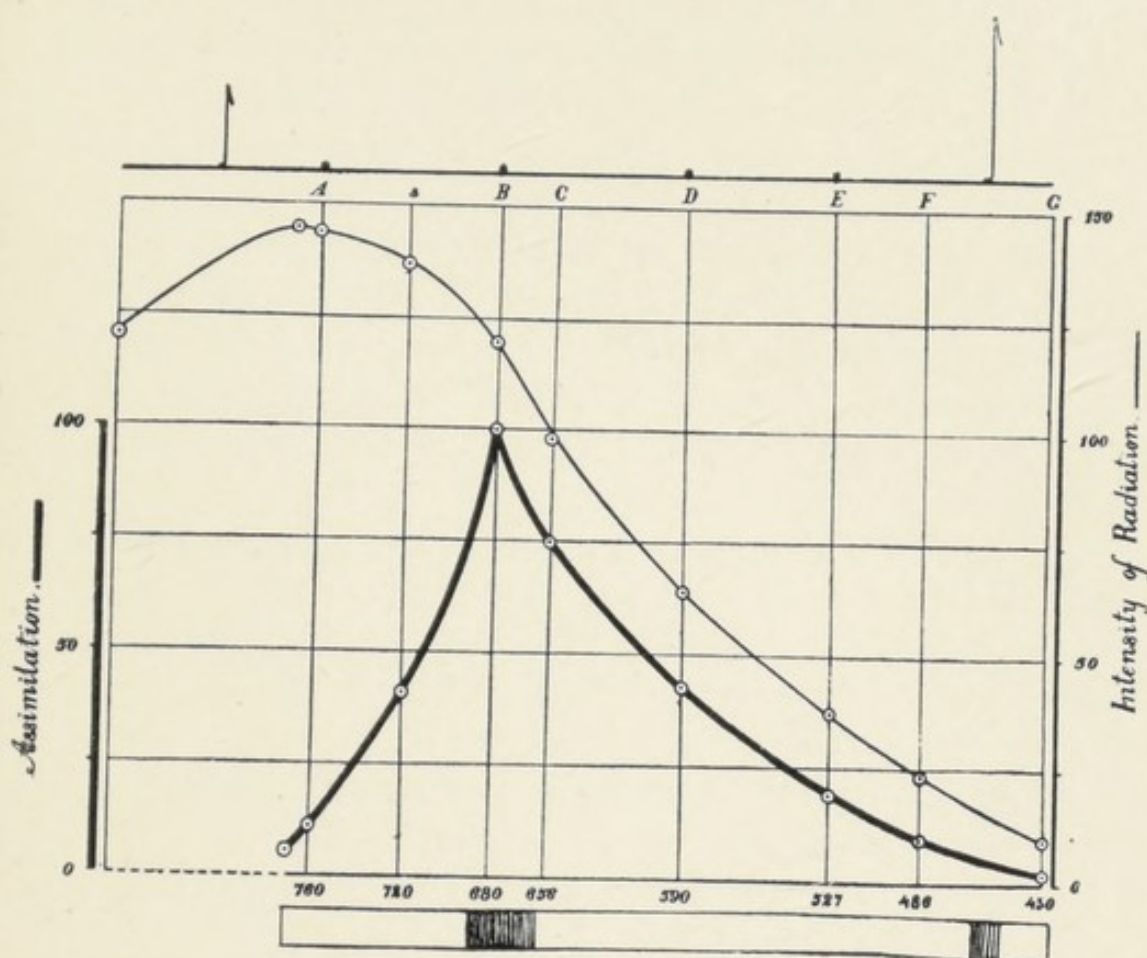
FIG. 51. Curves showing Distribution of Energy in the Spectrum (thin line) and corresponding Photosynthesis (thick line)
