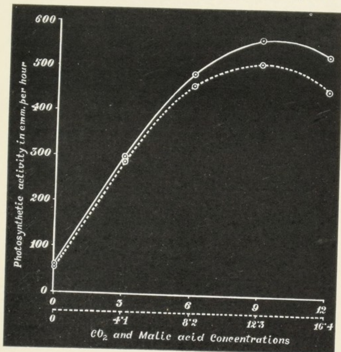
FIG. 36. Photosynthetic Curves under Increasing Concentration of \text{CO}_2 (upper curve) and of Malic Acid Solution (lower curve)
