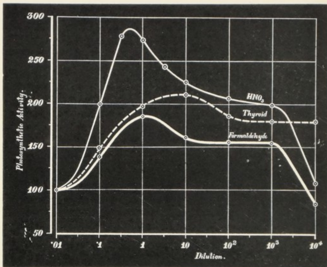
FIG. 17. Curves exhibiting the effect of infinitesimal traces of HNO 3 , of Thyroid Gland, and of Formaldehyde, on Photosynthetic Activity of Hydrilla
