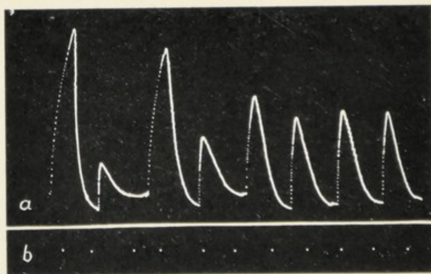
FIG. 11. (a) Alternating Response of Mimosa (upper record), and (b) of Photosynthesis (lower record)
