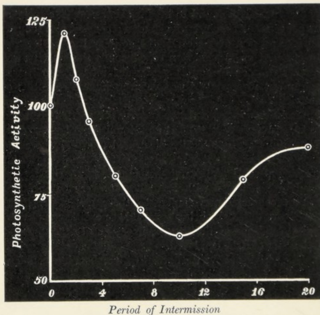
FIG. 28. Curve showing Variation of Photosynthetic Efficiency at various rates of Intermission of Light
