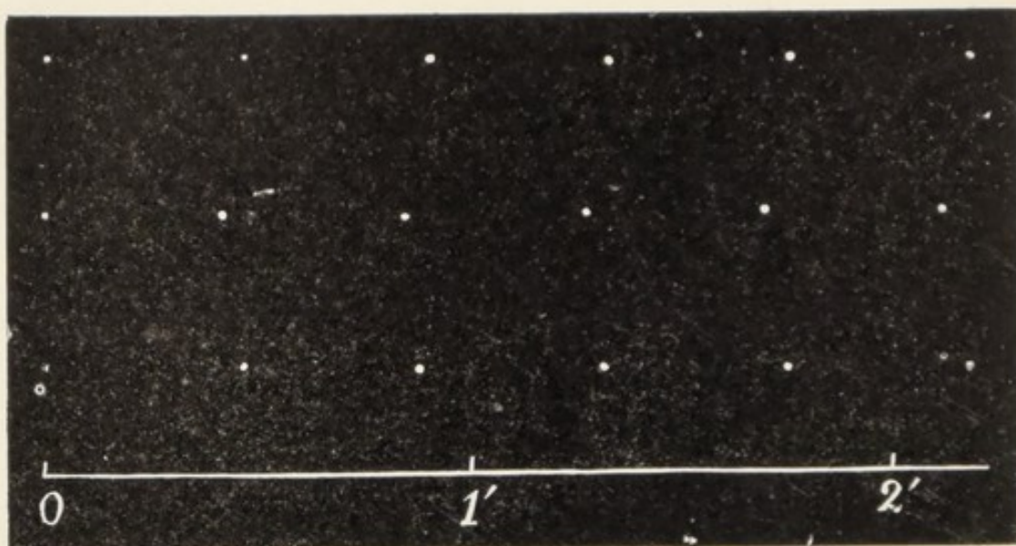
FIG. 4. Records of successive evolution of equal volumes of Oxygen under Constant Light
