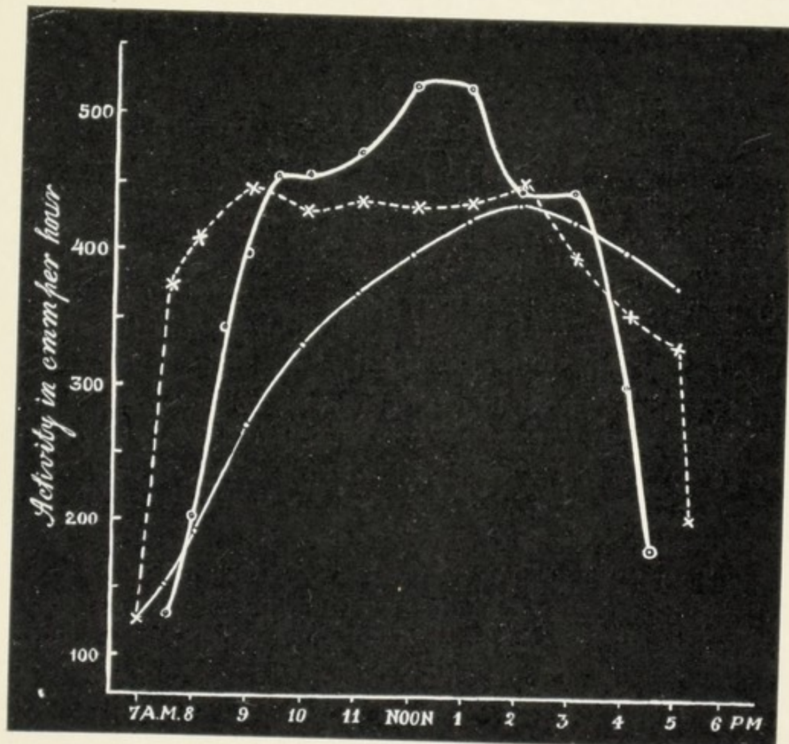
FIG. 45. The Curves for Light (dotted line), Temperature (thin line), and Resultant Photosynthetic Activity (thick line)
