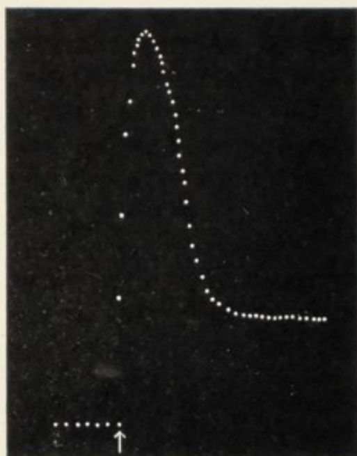
FIG. 12. Direct and After Effect of Light on Growth-elongation of Kysoor
