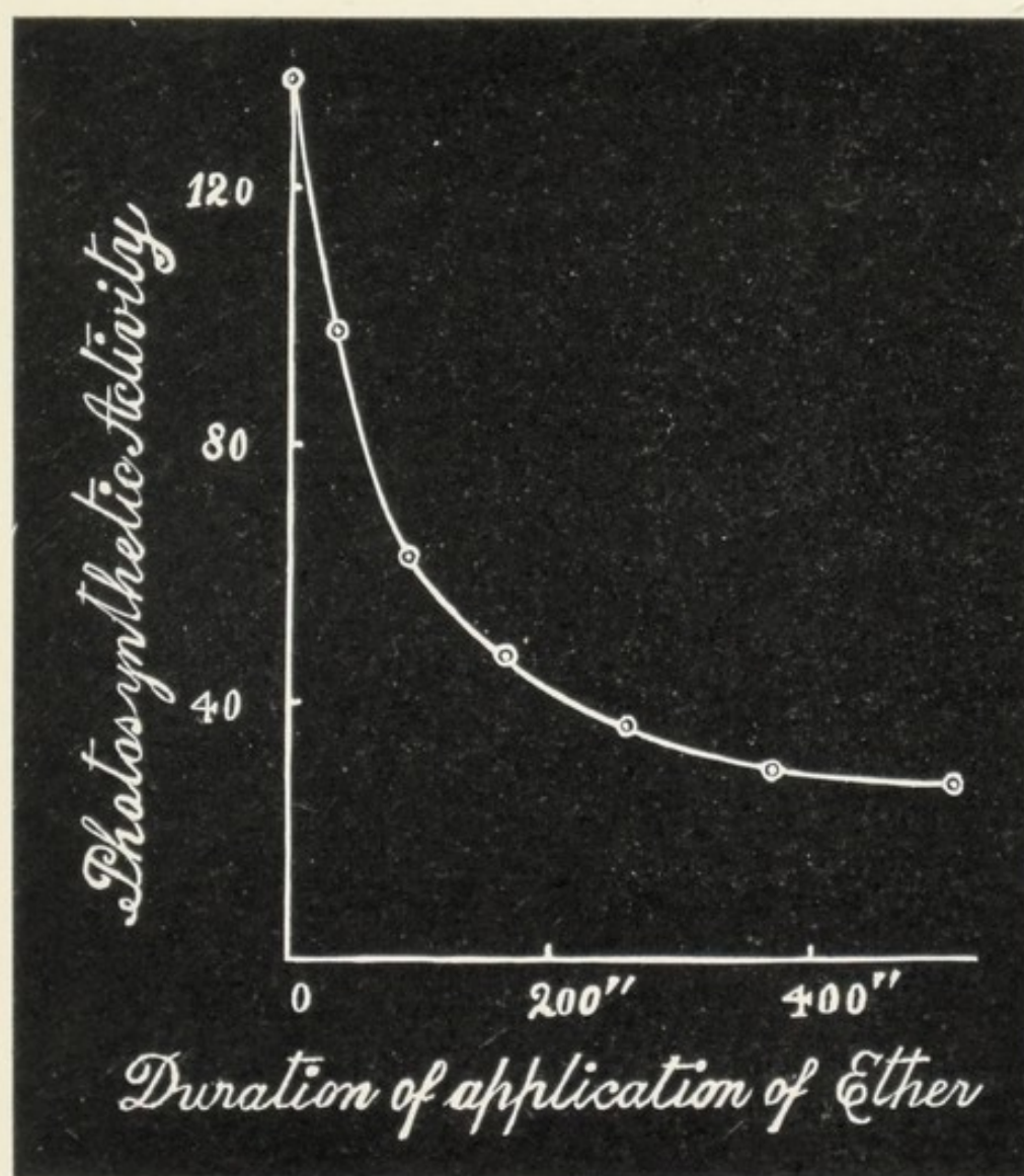
FIG. 15. Curve showing the effect on Photosynthesis of application of 1 per cent. Ether Solution
