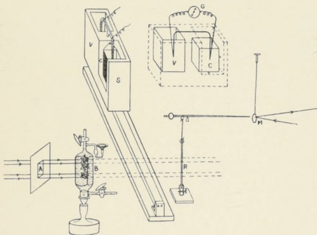
FIG. 55. Apparatus for Determination of Photosynthetic Efficiency
