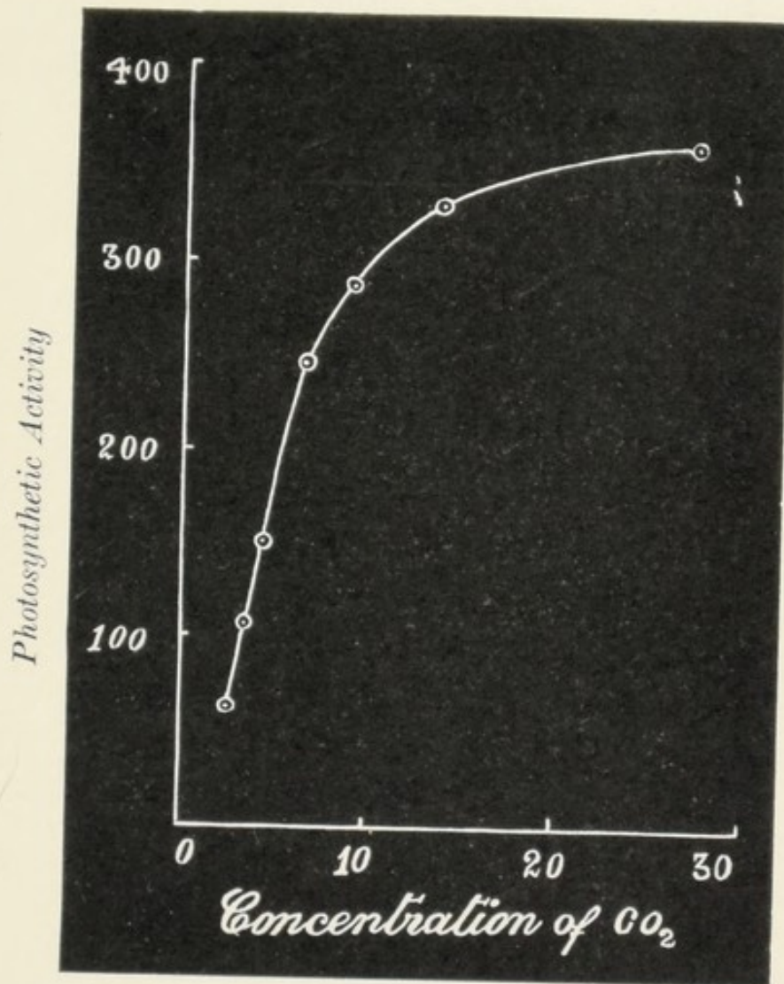
FIG. 33. The Photosynthetic Curve under Variation of \text{CO}_2 -concentration in mg. per 100 c.c.
