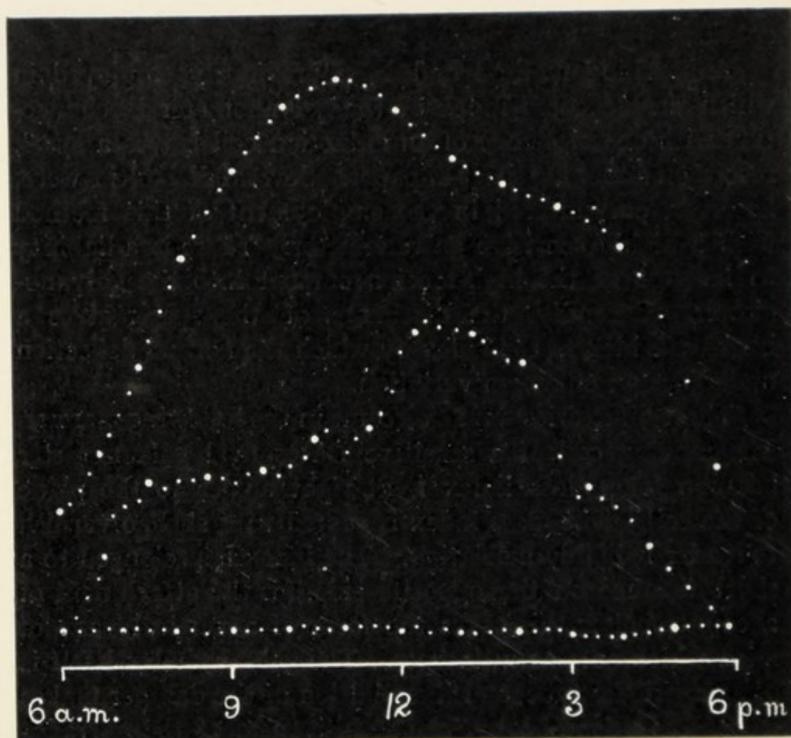
FIG. 30. Radiogram of Variation of Intensity of Light from the sky during 12 hours in winter
