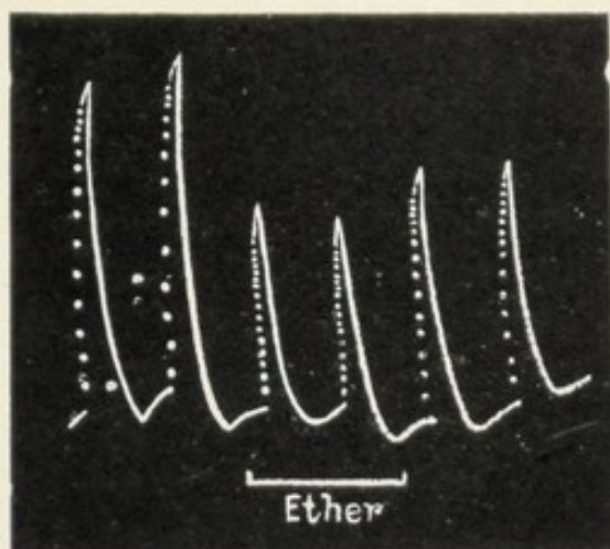
FIG. 13. Depression of Mechanical Response of Mimosa under Ether, and Gradual Recovery on Removal of the Anæsthetic
