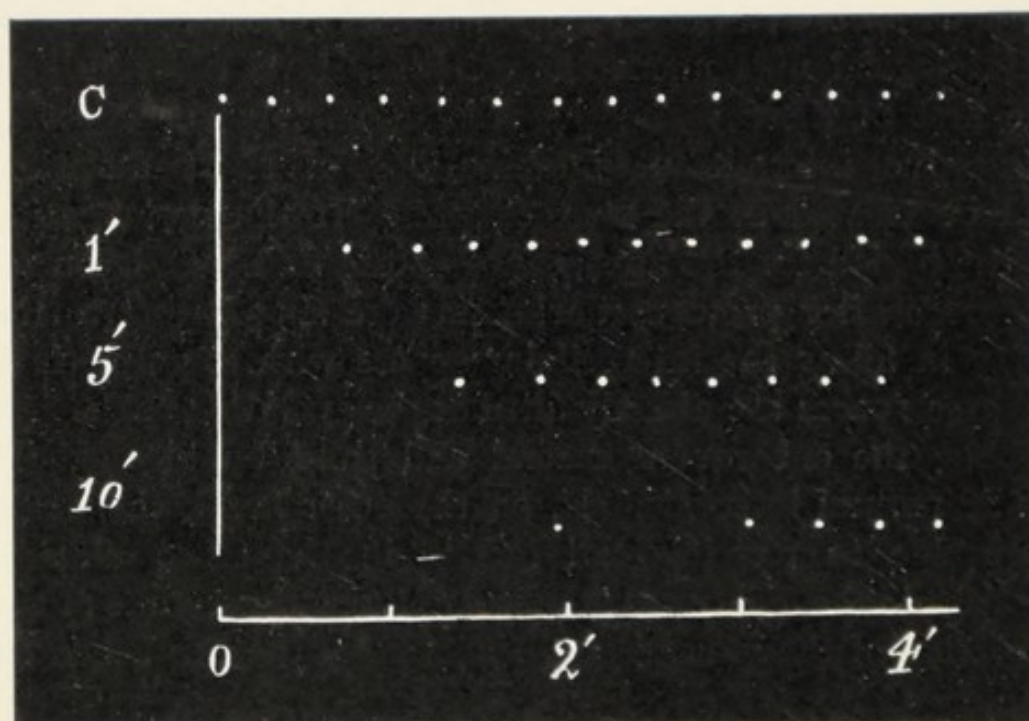
FIG. 26. Successive Records showing Increasing Induction-periods with Increasing Duration of Previous Darkness
