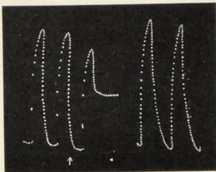
FIG. 23. Arrest of Desmodium pulsation under excess of \text{CO}_2 at arrow, and renewal on removal of the Gas
