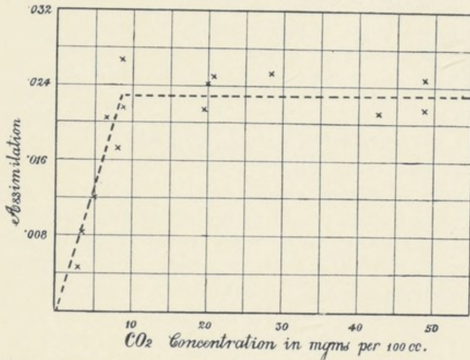
FIG. 34. Curve of Photosynthesis of Elodea under Variation of CO 2 concentration (after Blackman)
