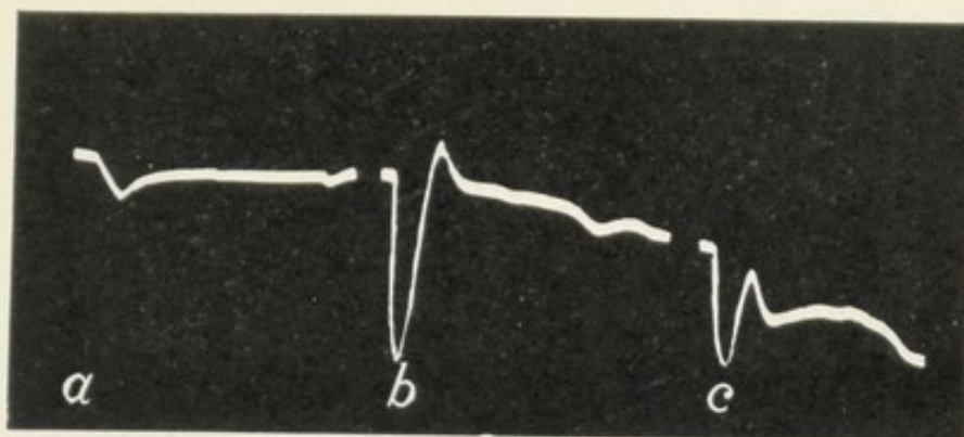
FIG. 22. Effect of Variation of Temperature on Electric Response of Hydrilla
