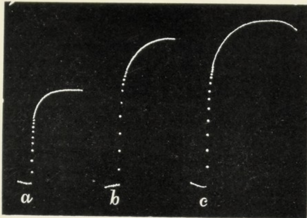
FIG. 10. Maximum Response of Mimosa under Increasing Intensity of Electric Stimulus
