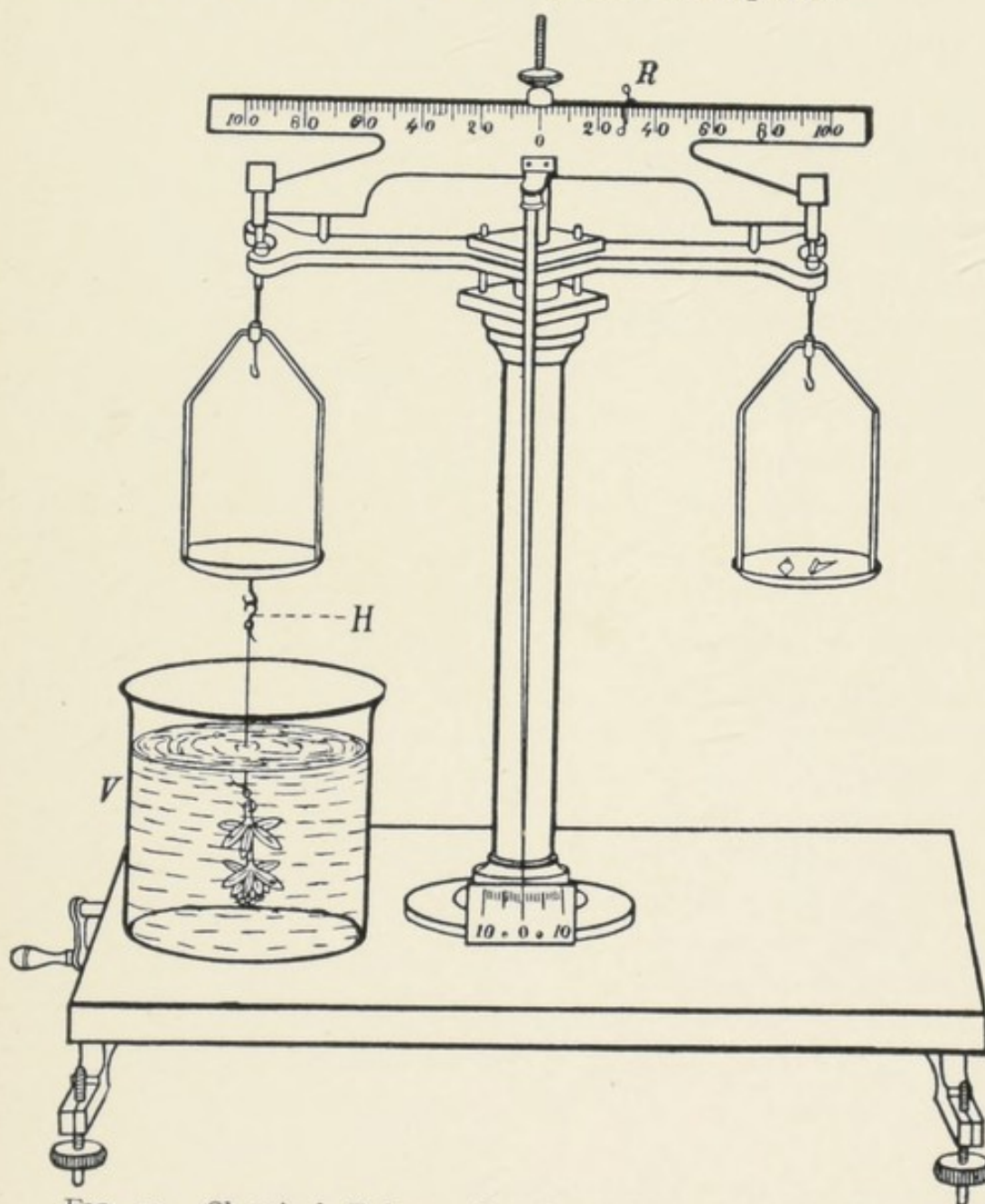
FIG. 53. Chemical Balance for determination of increase of weight of Hydrilla after exposure to Light Vessel v always kept on the Balance.
