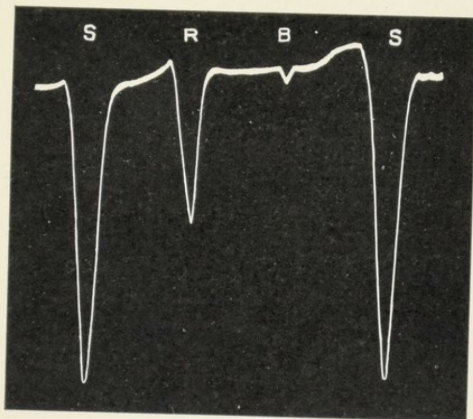
FIG. 35. Electric Response of Cicer arietinum
