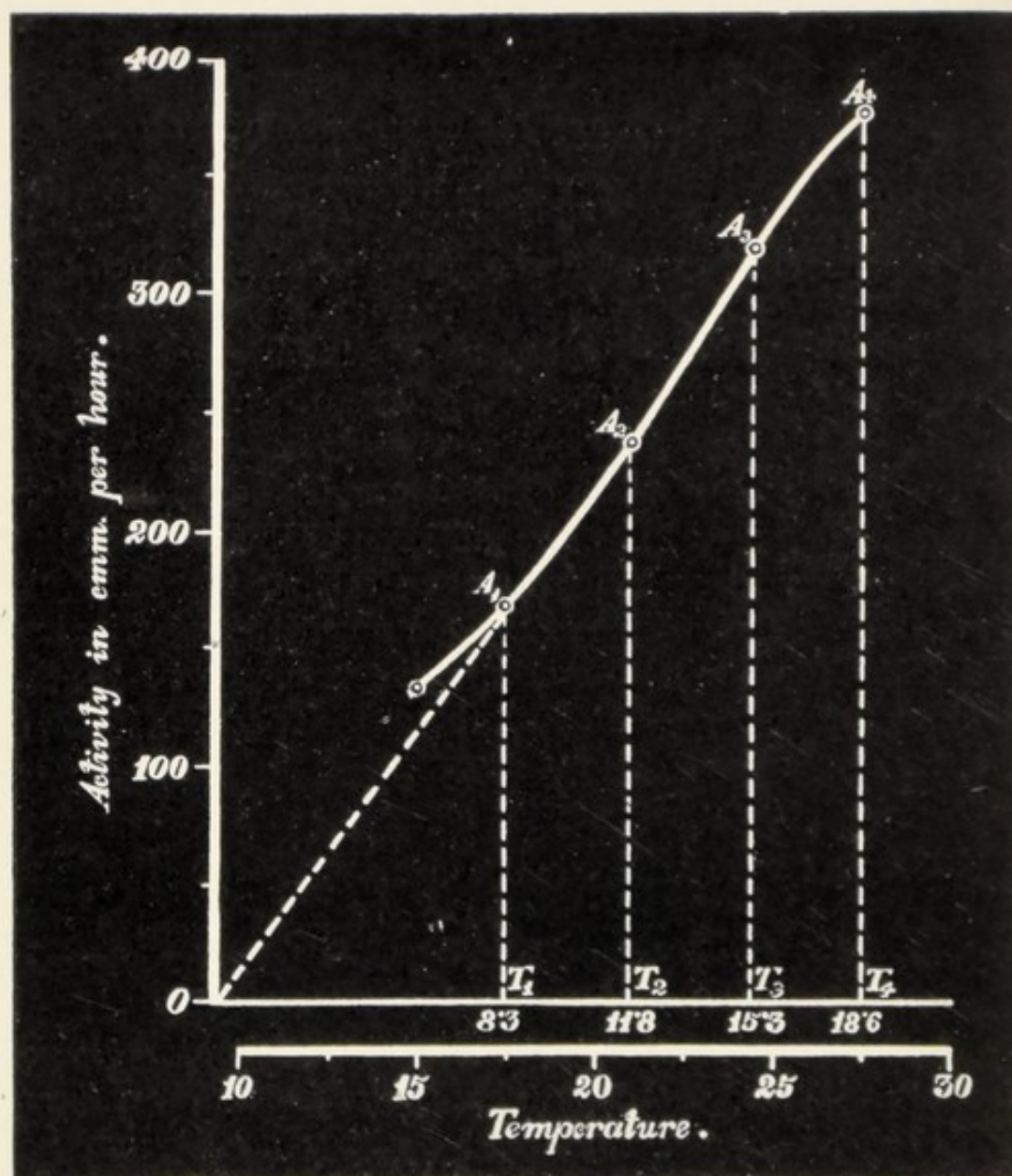
FIG. 57. Photosynthetic Curve under Variation of Temperature Curve produced backwards cuts abscissa at 9^{\circ}.2 , which is the physiological zero. The temperatures T_1 , T_2 , T_3 , T_4 on the physiological scale are given in the upper and on the centigrade scale in the lower line.
