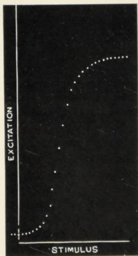
FIG. 9. The Tropic Curve under the Action of Light ( Erythrina indica )
