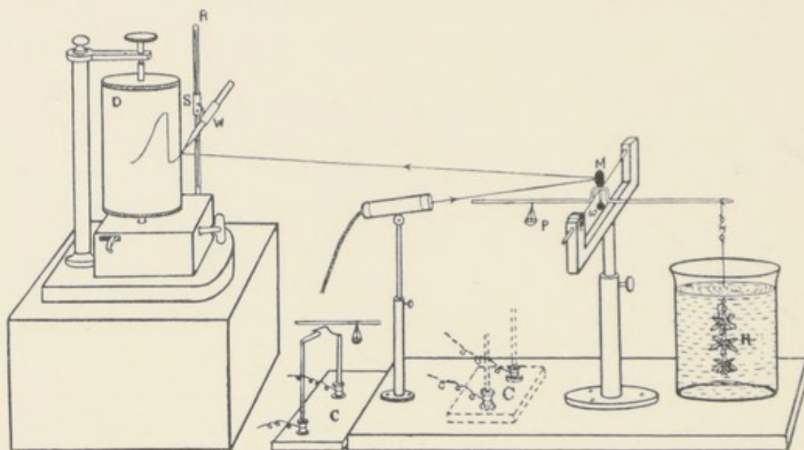
FIG. 46. Record of Photosynthetic Activity under Different Coloured Lights by the Method of Flotation
