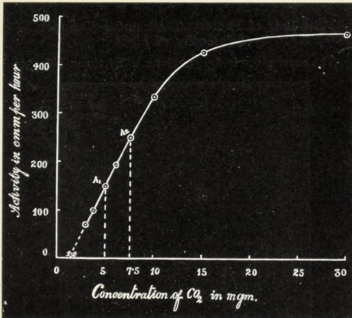
FIG. 58. Photosynthetic Curve under Variation of \text{CO}_2 -Concentration Physiological zero at 1.2 mg.
