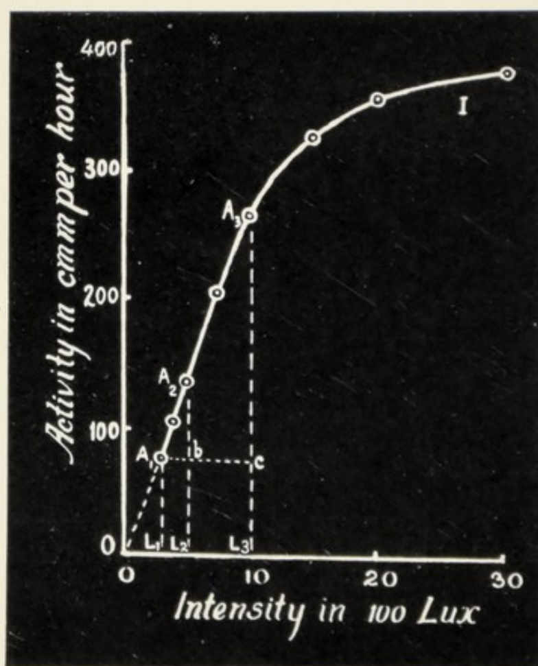
FIG. 59. Photosynthetic Curve under Variation of Intensity of Light
