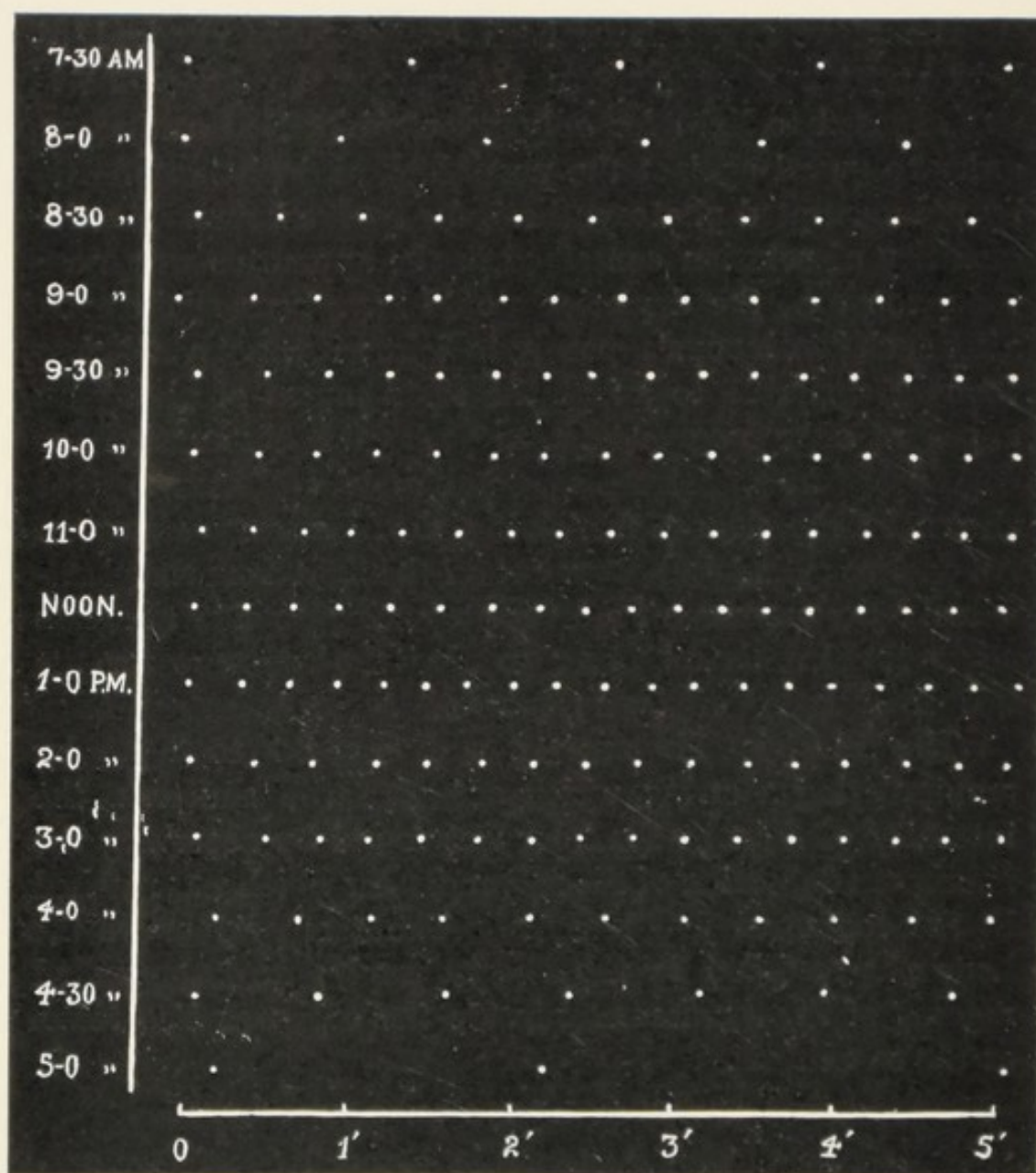
FIG. 44. Automatic Records of successive Bubbblings for five minutes during different periods of the Day
