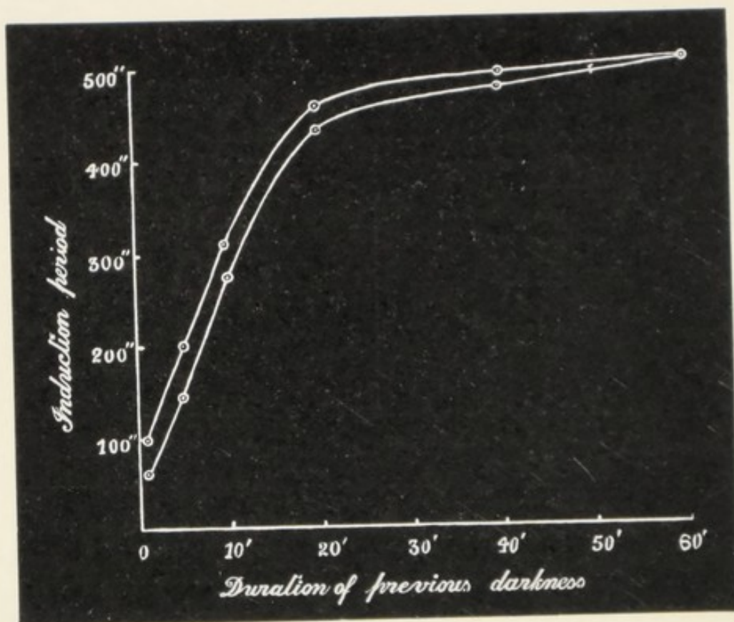
FIG. 25. Cyclic Curve showing effect of Increasing (lower curve) and Decreasing (upper curve) Periods of Darkness on Induction-period
