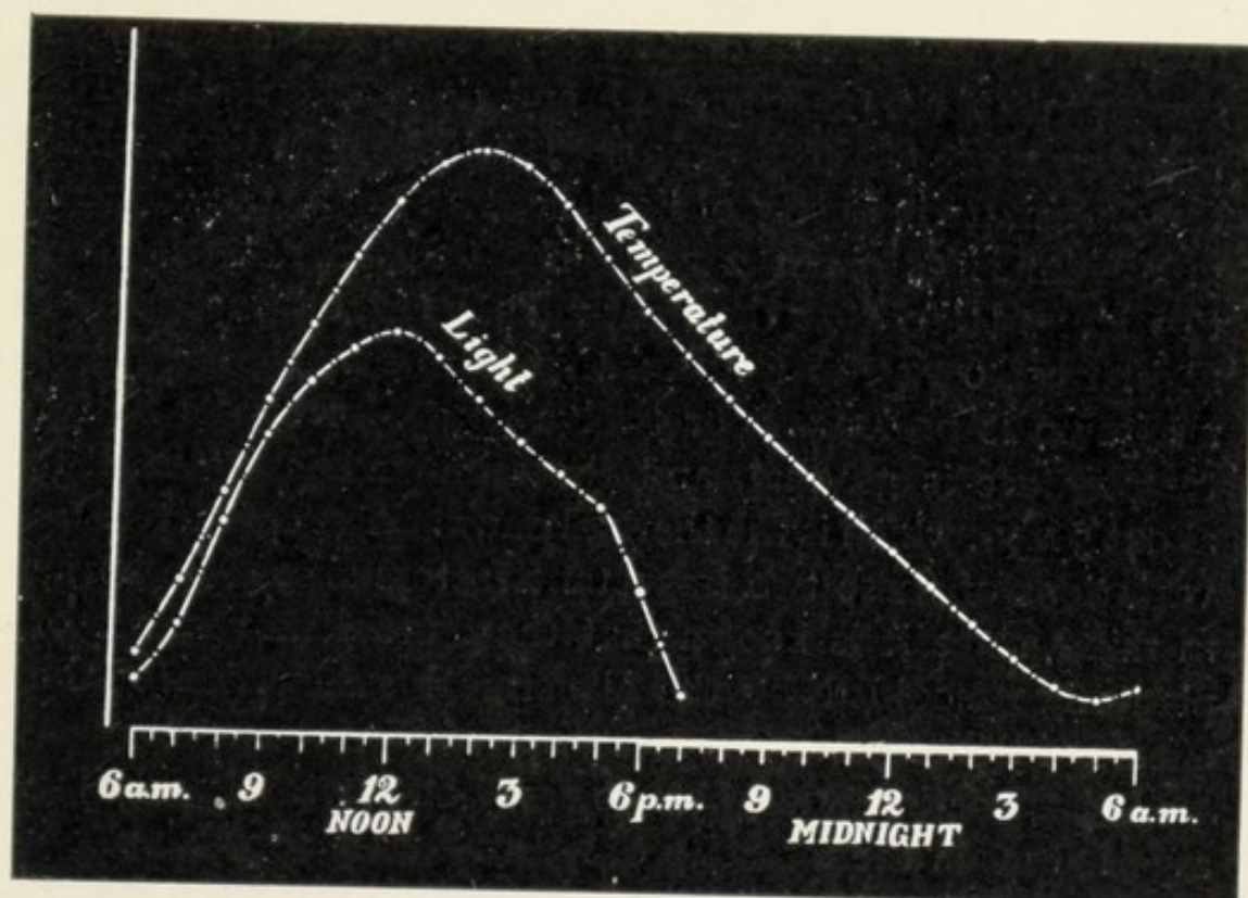
FIG. 31. Record of Diurnal Variation of Light and of Temperature in Summer
