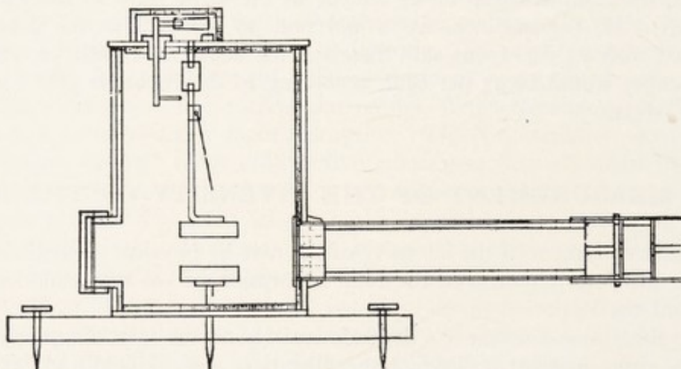
FIG. 143.—BACHEM'S ELECTROSCOPE.
