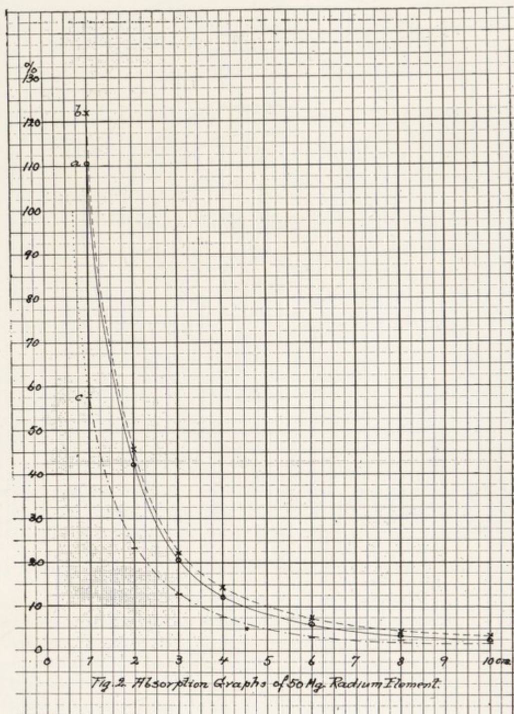
FIG. 149.—ABSORPTION GRAPHS OF 50 MG. RADIUM ELEMENT ARRANGED AS SHOWN IN FIG. 148, MEASURED IN WATER.
