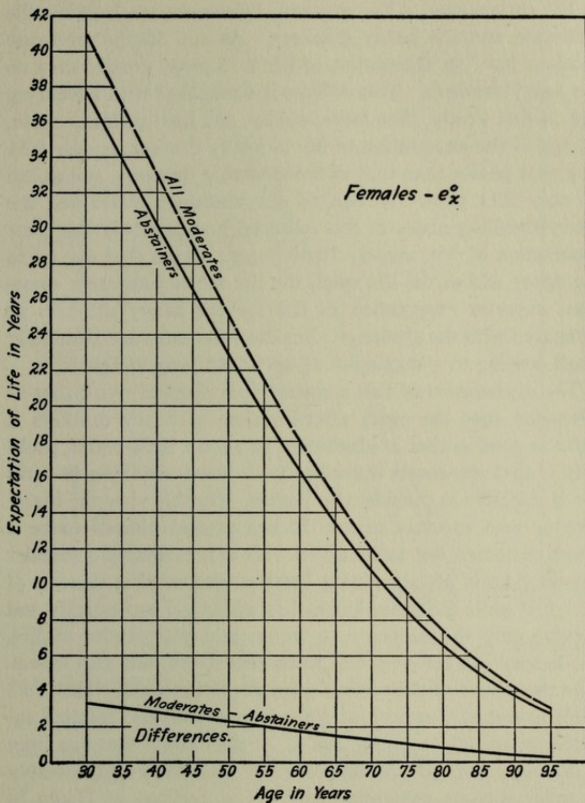
FIG. 11. The expectation of life ( e_x^o ), in years, for females falling in the two categories (a) abstainers (solid line), and moderate drinkers (dash line). At the bottom of the diagram are plotted the differences, in years, between moderate drinkers and abstainers (solid line). Data from Table XXIV.
