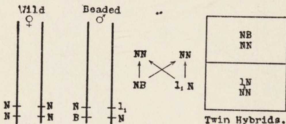
FIG. 116.—Diagram illustrating balanced lethals and twin hybrids.
