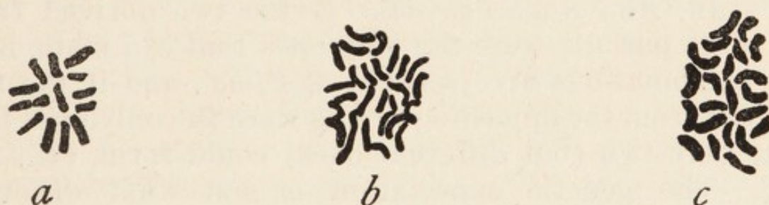
FIG. 58.—Chromosome group of Oenothera lamarckiana , a ; chromosome group of O. gigas , b ; triploid group, c .
