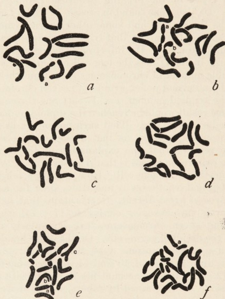
FIG. 62.—Somatic chromosomes groups of Oenothera scintillans , showing variable numbers of chromosomes. (After Hanse.)
