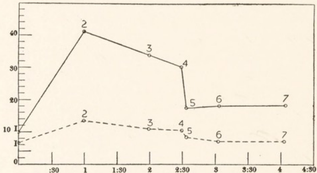
FIG. 20.—A record plotted from the data of one experiment. The time intervals in hours and minutes are registered on the abscissa; the values of the threshold in units are registered on the ordinate. The continuous line is the record of the muscle, the broken line that of the nerve-muscle. The record of the nerve-muscle is magnified ten times; that of the muscle is normal.
