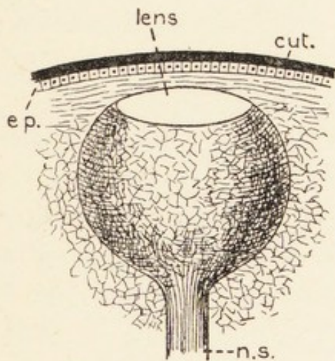
FIG. 26.—The “third” eye, or pineal eye, of the Green Lizard, exposed by dissection. cut. , cuticle; ep. , cellular epiderm; lens , the lens forming the top of the eyeball; n.s. , the nerve stalk, or optic nerve.
