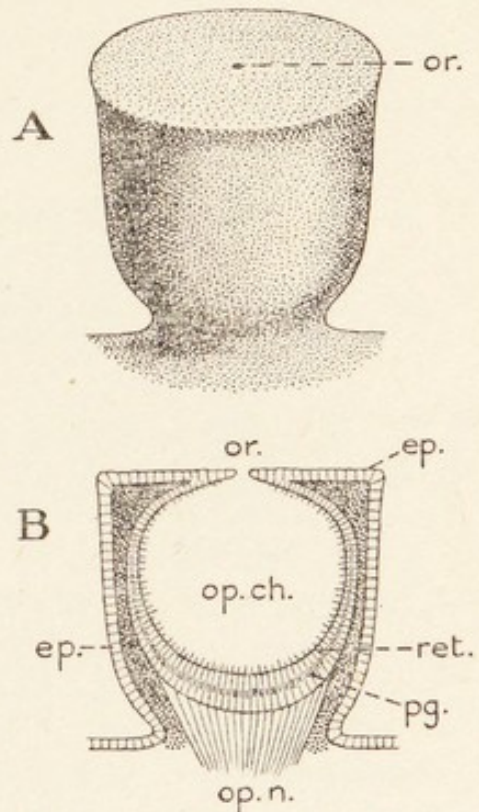
FIG. 33.—Eye of the Pearly Nautilus.
