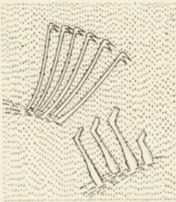
FIG. 22.—The uncleft "Genital" Bristles of an adult Chætogaster Limnææ , growing close to the first pair of abdominal bristle-bundles, and indicating the formation here of a new segment, the genital segment shown in Fig. 20, A, and not present in the fissiparous immature worms drawn in Fig. 20, B.
