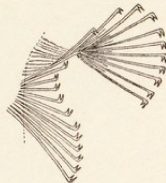
FIG. 21.—[Fan-like Bundle of Bristles, twenty-two in number, from the head-region of the adult or sexually mature Chætogaster Limnææ .
