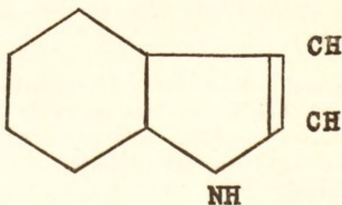
(Indole)
