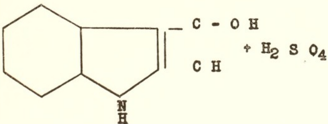
(indoxyl)
