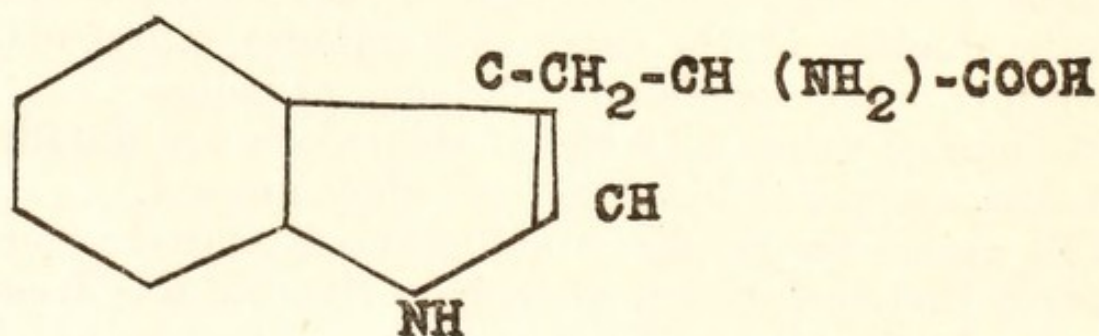
(Tryptophane)
