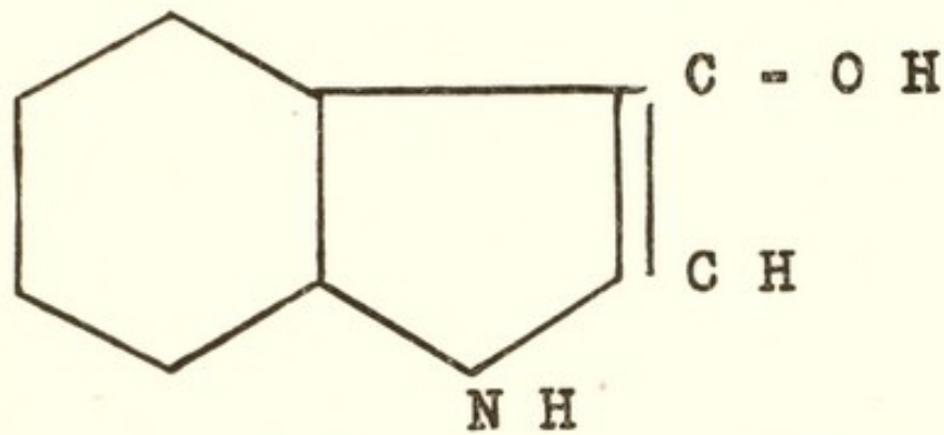
(Indoxyl)
