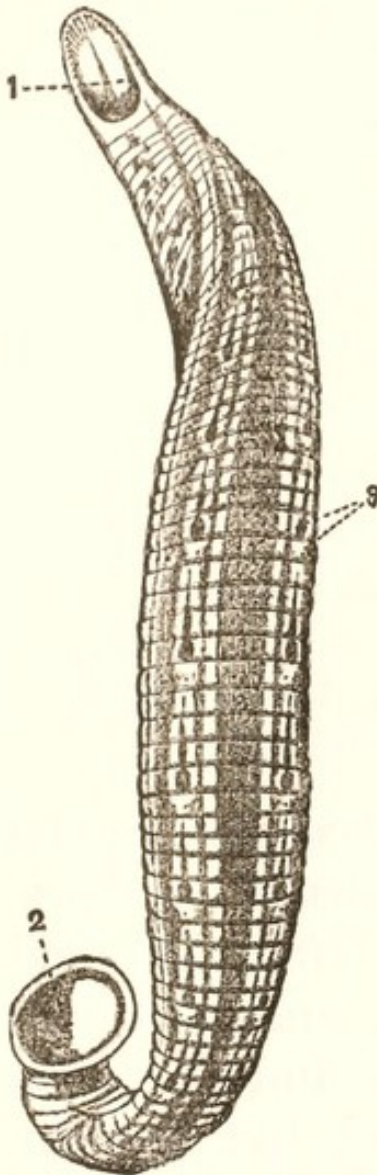
FIG. 48. — Hirudo medicinalis ; about life size. 1, Mouth; 2, posterior sucker; 3, sensory papillae on the anterior annulus of each segment. The remaining four annuli which make up each true segment are indicated by the markings on the dorsal surface.
