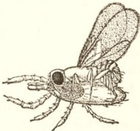
FIG. 47.— Ixodiphagus caurtei laying eggs in the nymph of Ixodes ricinus . \times 20 . (After Brumpt.)
