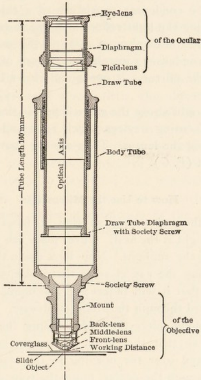
Fig. 3 (b).—Internal structure of the microscope.
