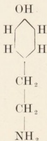
Para-hydroxy-phenylethylamine
