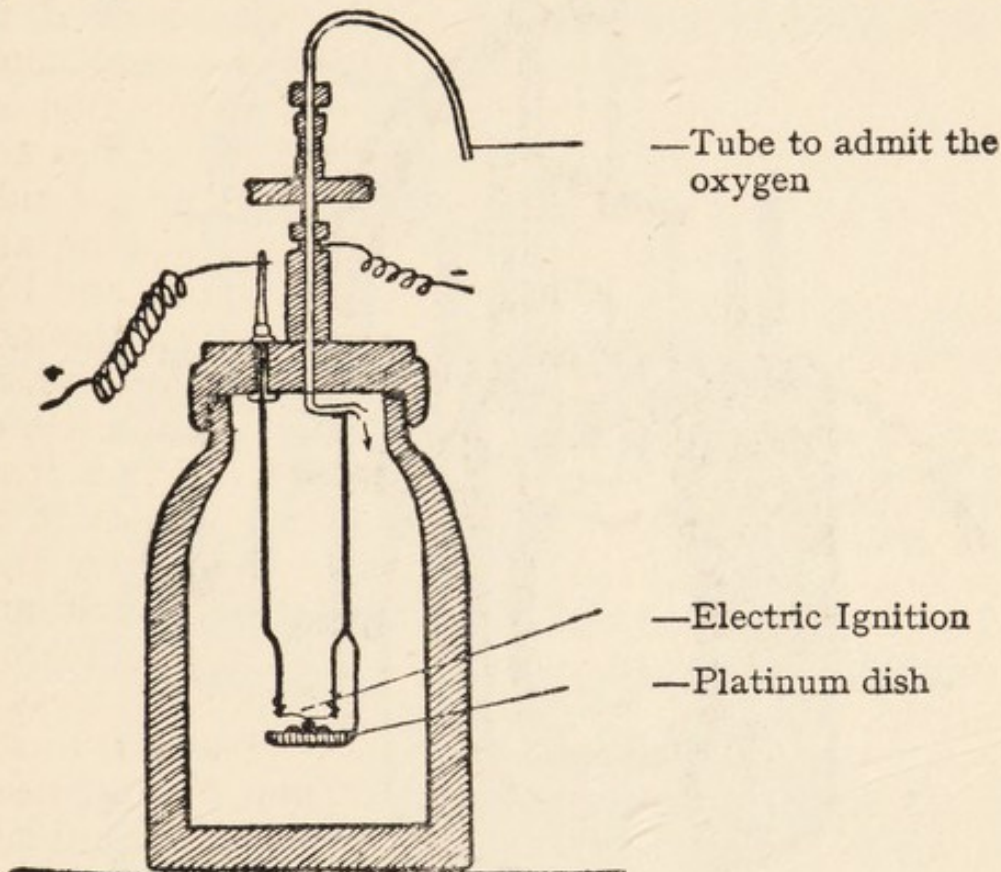
FIG. 1. Berthelot's Bomb
