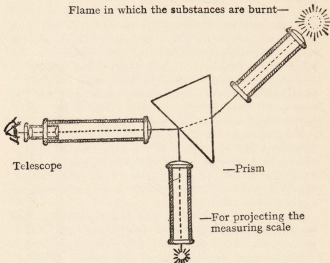
FIG. 4. Spectroscope
