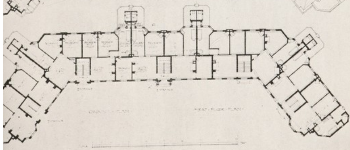
Design No. 2 (detail plans and elevations).
