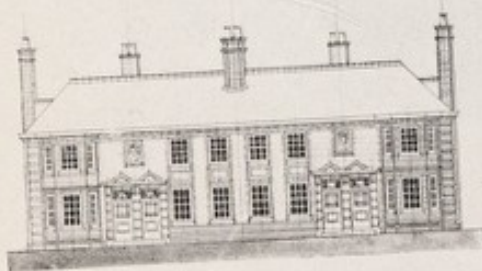
FRONT ELEVATION TO EASTBURY ST.
