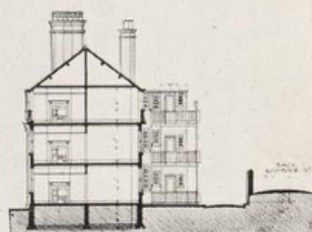
CROSS SECTION A - D
