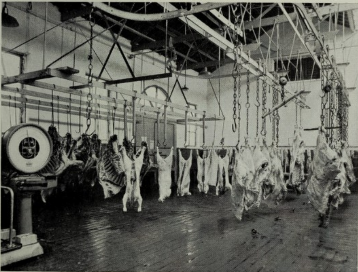
PART OF MAIN SLAUGHTERING HALL
