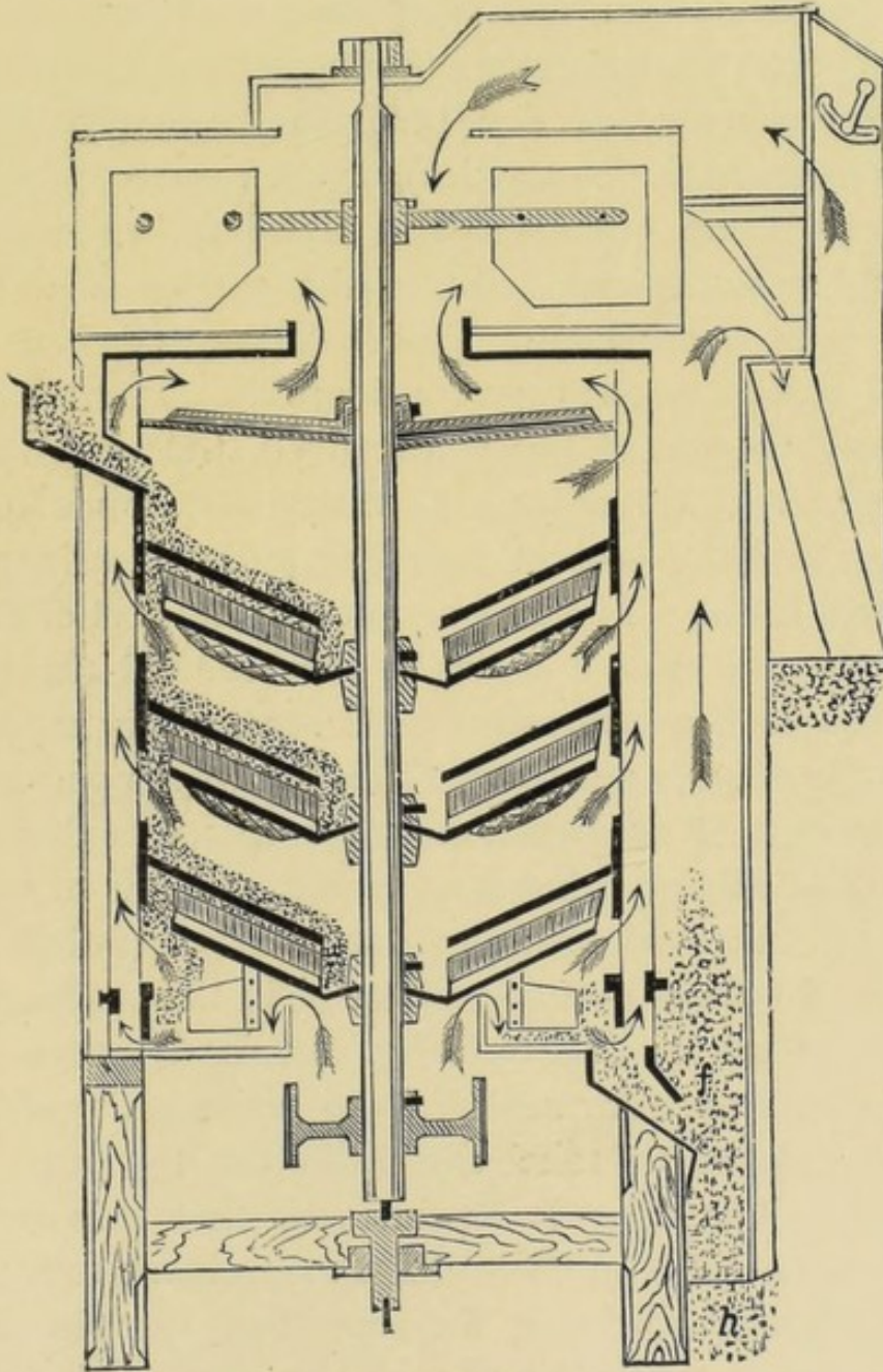
FIG. III.— Double Brush Scourer and Polisher.
