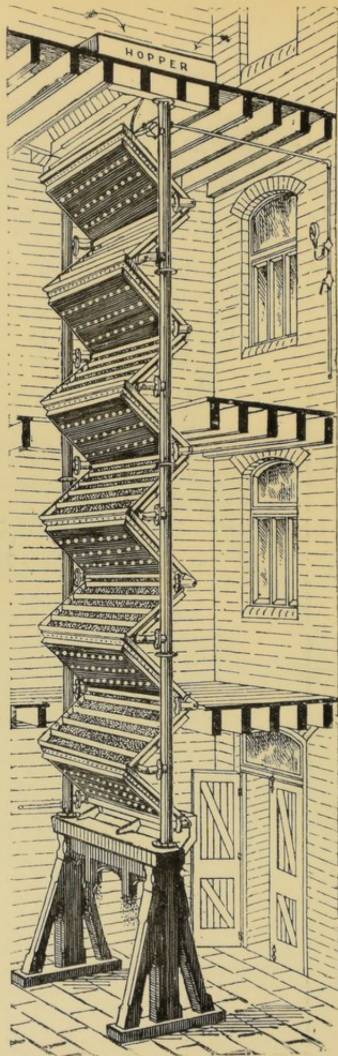
FIG. II.—Automatic Grain Drier and Conditioner.
