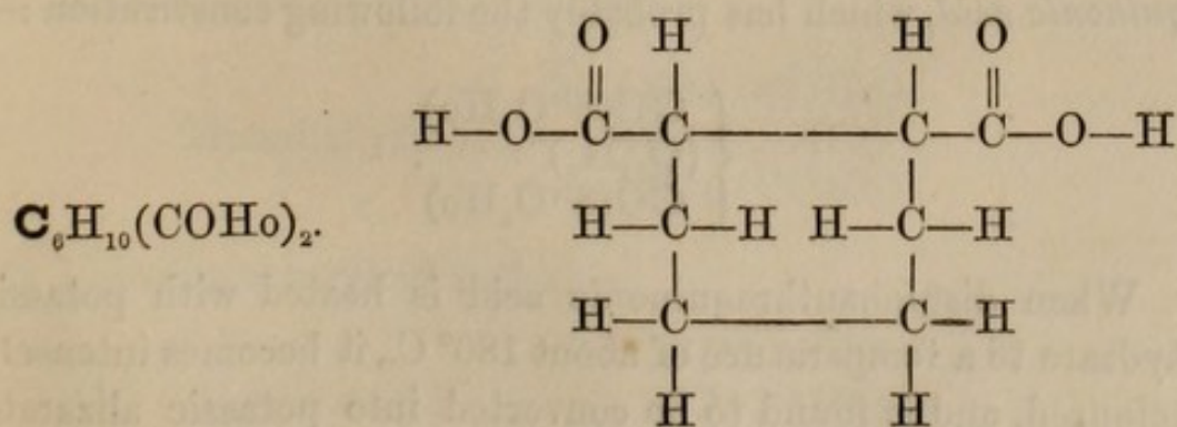
Hexahydrophthalic acid (Hexacarbon-succinic series).
