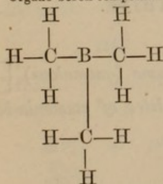
Boric methide.
