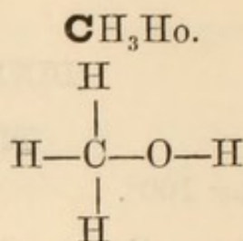
Methylic alcohol.
