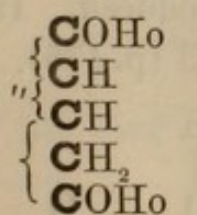
Itaconic acid.
