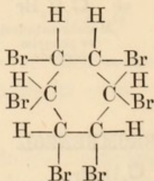
Tribrombenzol hydrobromate.
