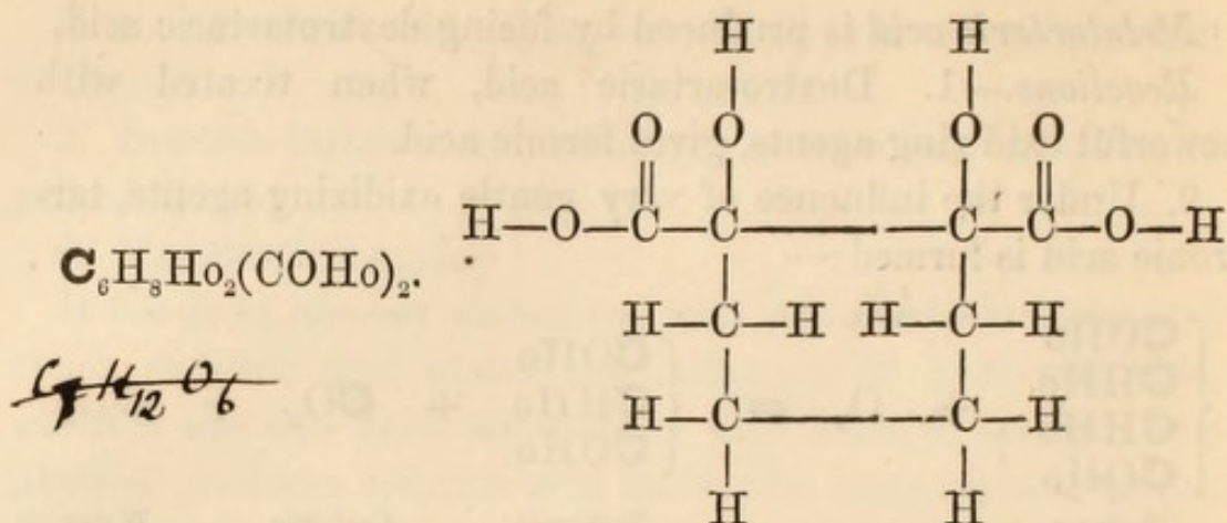
Tartrophthalic acid (Hexacarbon-tartaric series).
