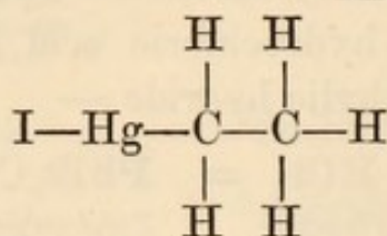
Mercuric iodethide.
