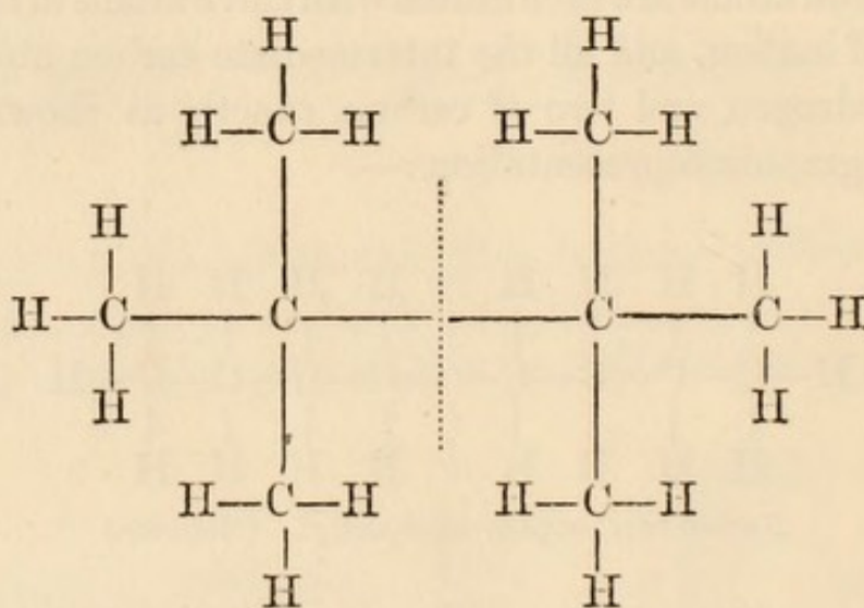
Trimethylated methyl. (Molecule.)
