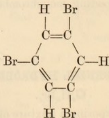
Tribrombenzol.
