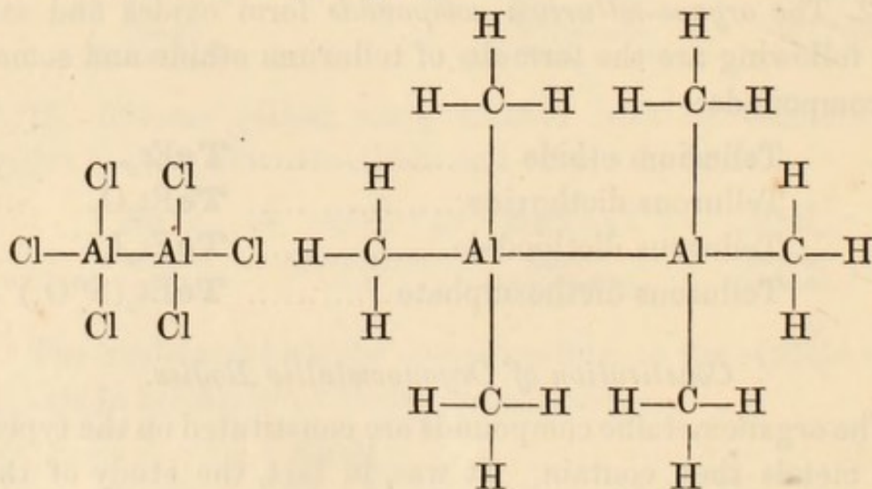
Aluminic chloride.
