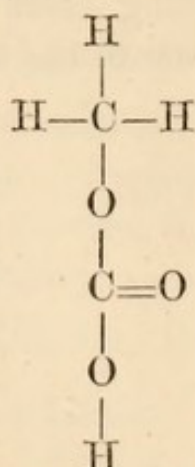
Carbomethylic acid.
