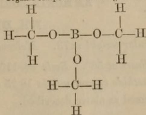
Methylic borate.
