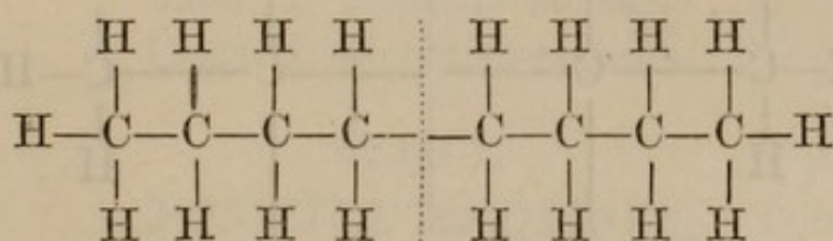
Normal butyl or propylated methyl. (Molecule.)
