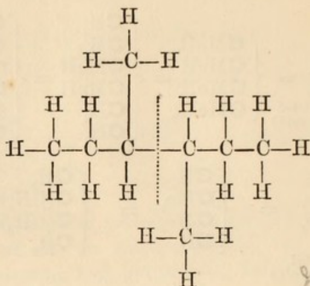
Methylo-ethylated methyl. (Molecule.)
