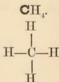
Marsh-gas.
