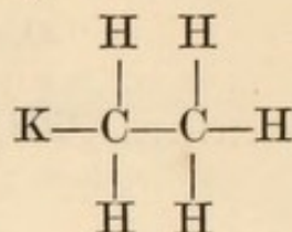
Potassic ethide.
