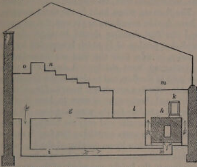
Fig. 138. Section of a greenhouse, with reserve flue and common flue.
