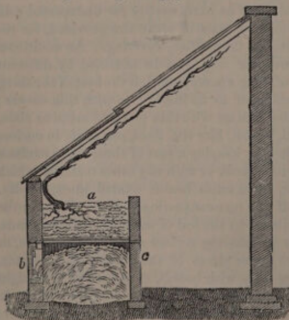
Fig. 136. Section of a vinery heated by dung.
