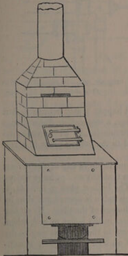
Fig. 149. Rogers's boiler set, with the chimney added.
