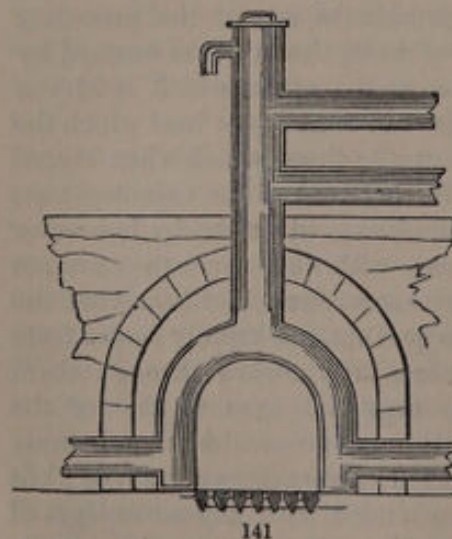
Fig. 141. Boiler and furnace for heating by hot water in rising and falling pipes.
