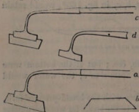
Fig. 162. The Leicestershire or shifting-blade draw hoe.
