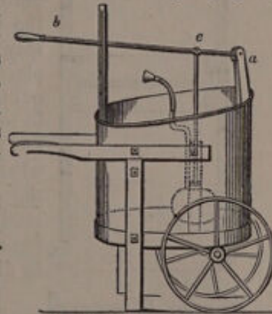
Fig. 83. Read's barrow-engine.
