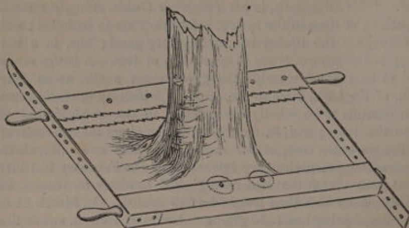
Fig. 262. Perspective view of the girdling machine.
