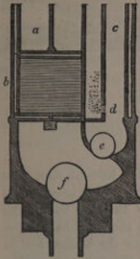
Fig. 82. Section of Read's pneumatic hand-engine.
