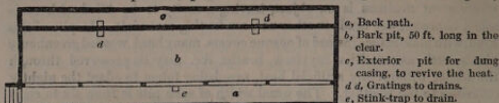
Fig. 157. Ground plan of a pit to be heated in Mr. Corbett's manner.
