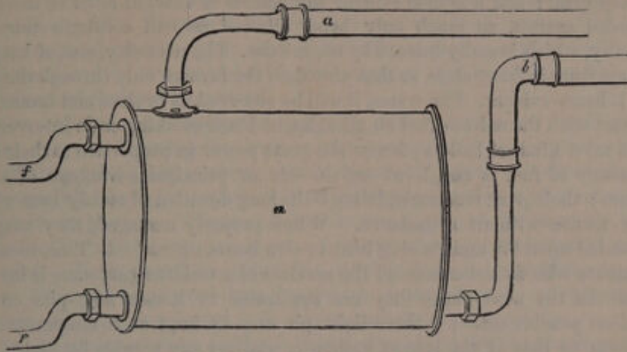
Fig. 152. Rogers's hot-water reservoir.
