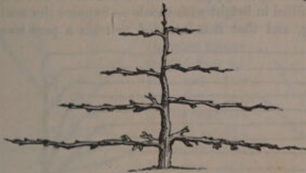
Fig. 309. Horizontal training, third stage.
