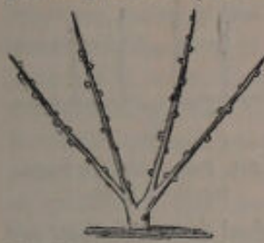
Fig. 316. Half-fan training, second stage.
