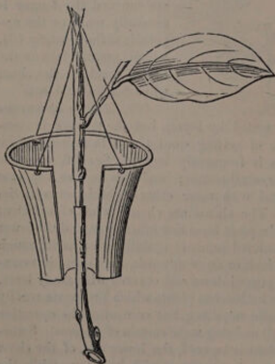
Fig. 189. A branch ringed and prepared to be rooted in a tin case without separating it from the tree.
