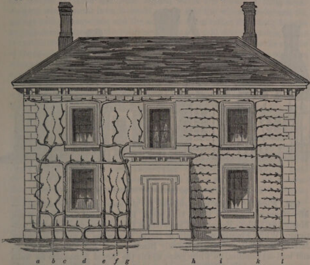
Fig. 354. The front of a plain house, covered with grape vines on the left side, and other fruit trees on the right side.
