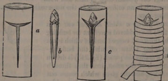
Fig. 248. Budding with a terminal eye.
