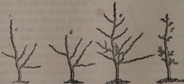
Fig. 276. Spurring-in, progressive stages.
