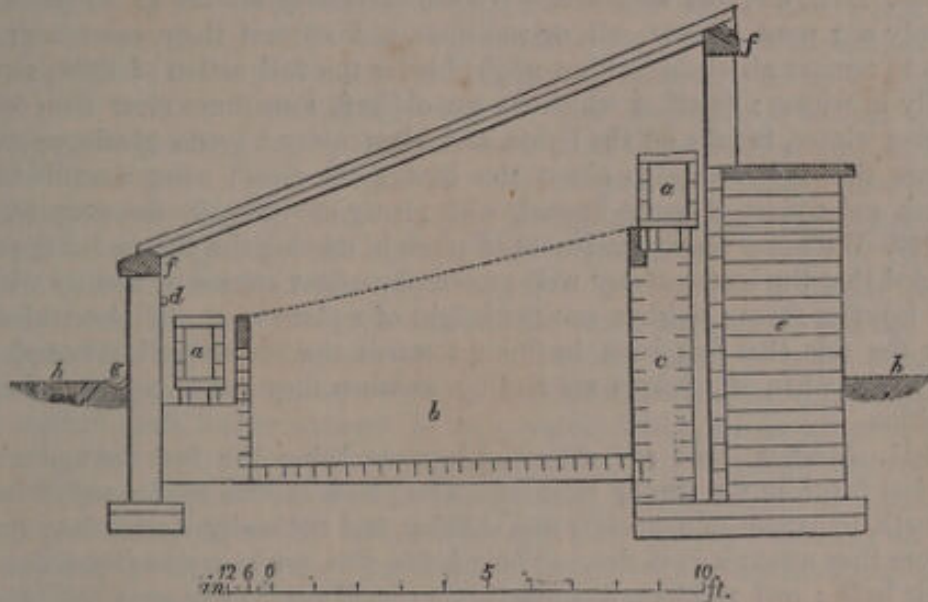
Fig. 335. Section of the pine pit at Oakhill.
