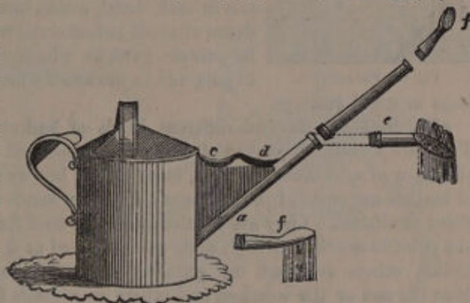
Fig. 63. Money's inverted-rose watering-pot.
