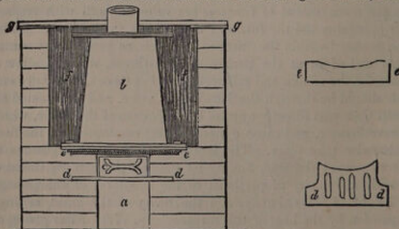
Fig. 148. Mode of setting Rogers's conical boiler.
