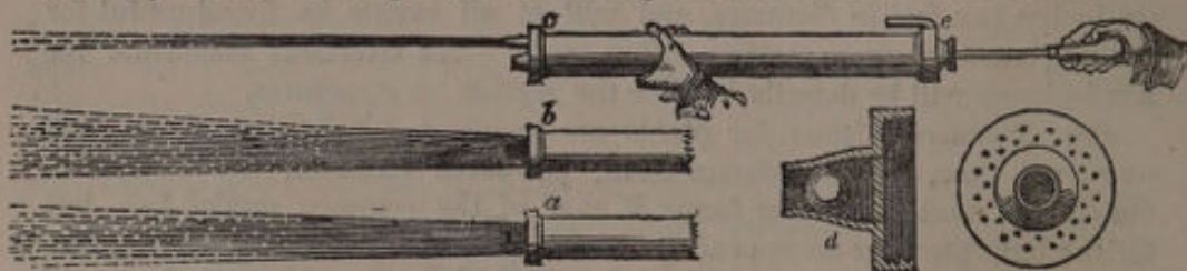
Fig. 80. Read's garden syringe.
