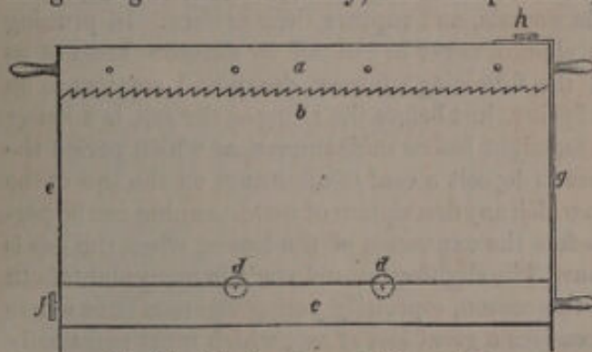
Fig. 261. Side view of the girdling machine.
