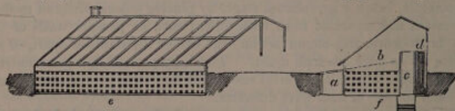
Fig. 135. Pinery heated by dung linings.
