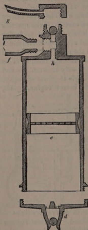
Fig. 85. Section of the canister of Read's fumigating bellows.
