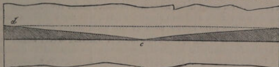
Fig. 155. Lap of glass panes puttied and painted.
