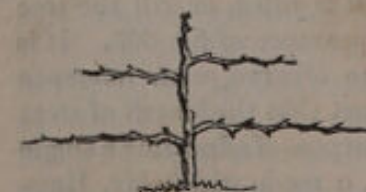
Fig. 308. Horizontal training, second stage.
