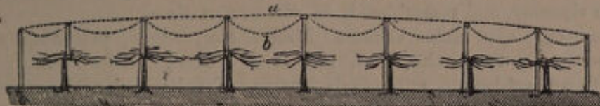
Fig. 372. Section through a Cherry Garden, showing the netting tightened by rain, ( a ) and slackened by drought ( b ).
