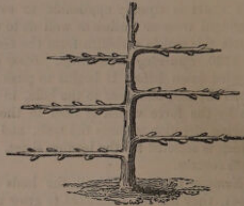
Fig. 360. Horizontal Training, first year.
