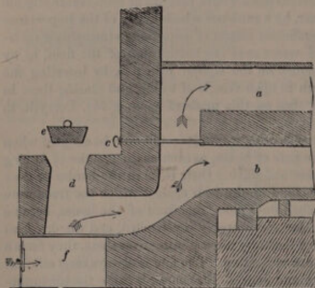
Fig. 137. Section of a furnace and double flue.
