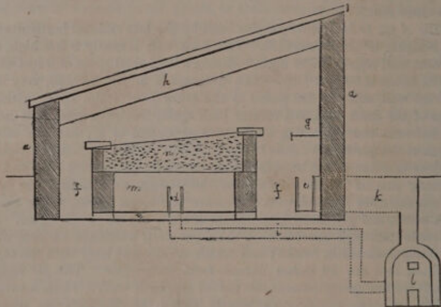
Fig. 356. Cucumber or Melon Pit, heated by hot water in open troughs. The scale \frac{1}{4} of an inch to a foot.
