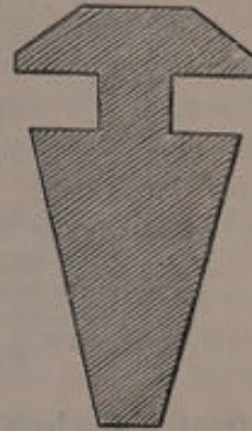
Fig. 131. Section of a wooden sash-bar, with grooves for the glass.
