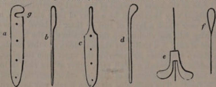
Fig. 328. Details of wire fastening mats on frames, one-sixth of the full size.
