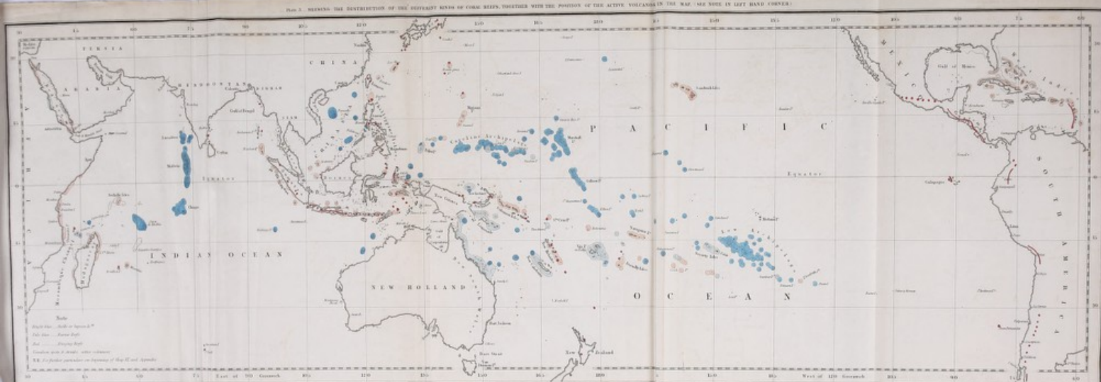
PLATE 2. SHOWING THE DISTRIBUTION OF THE DIFFERENT KINDS OF CORAL REEFS, TOGETHER WITH THE POSITION OF THE ACTIVE VOLCANOS IN THE MAP (SEE NOTE IN LEFT HAND CORNER).
