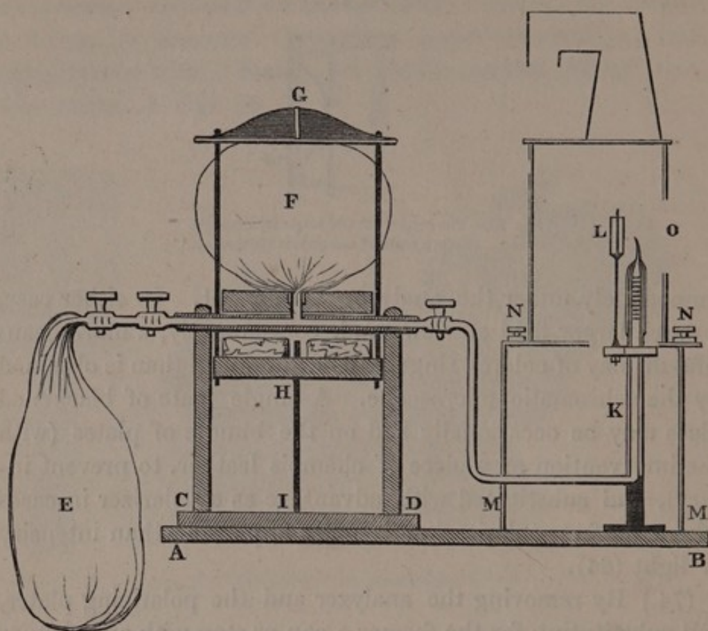
Fig. 22.—The hydro-oxygen apparatus on a scale of one inch to a foot.
