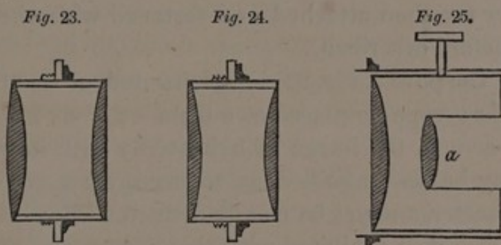
Fig. 23. —Condensers for the gas polariscope.
