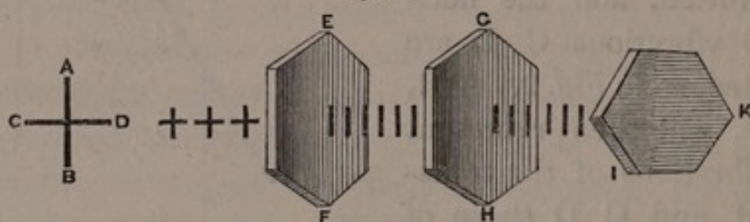
E F, G H, I K, plates of tourmaline.—The horizontal vibrations C D stopped by E F.—The perpendicular vibrations A B transmitted by E F and G H, but stopped by I K.
