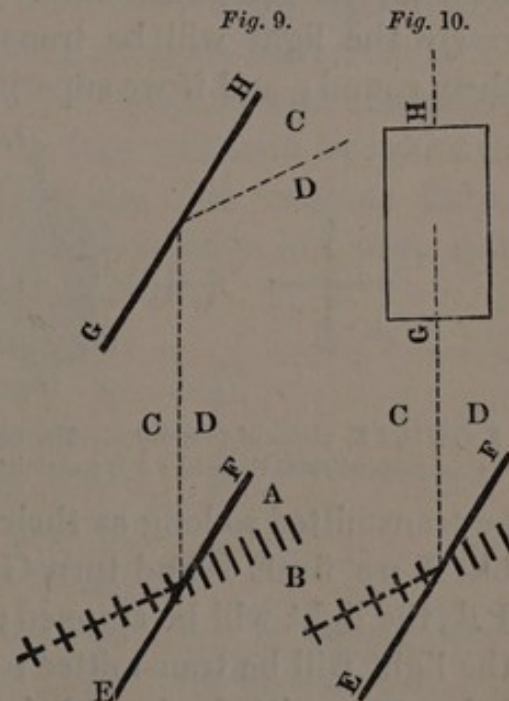
Fig. 9.—The perpendicular vibrations A B transmitted by E F.—The horizontal vibrations C D reflected first by E F, and again by G H.
