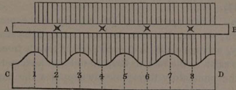
Fig. 3.—Intensity of waves doubled by the superposition and coincidence of two equal systems.
