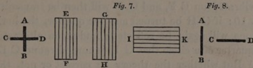
Fig. 7.—A B, C D, rectangular vibrations for common light.
