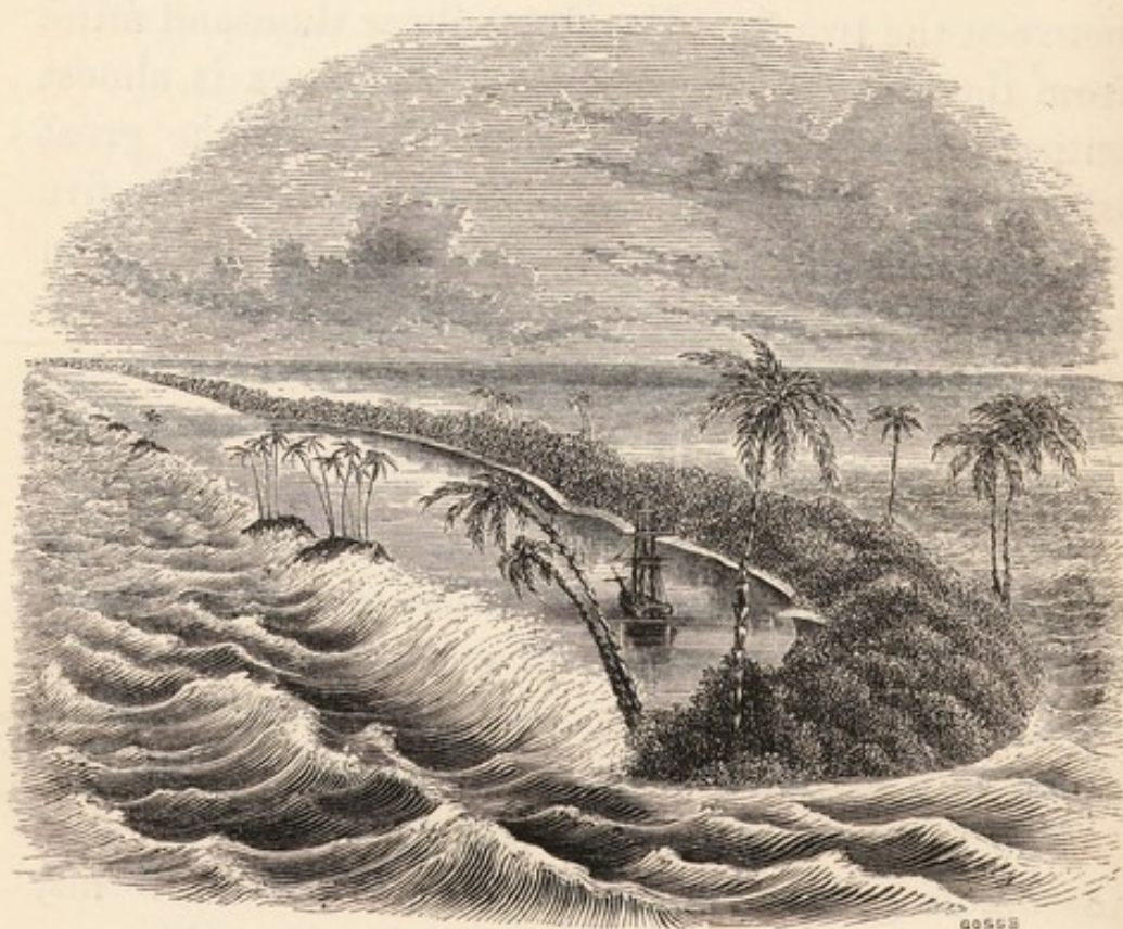
CORAL ISLAND.
