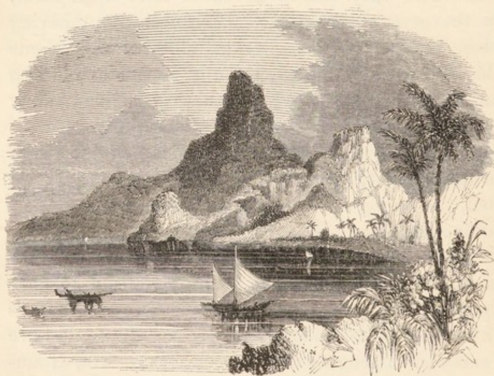
VOLCANIC ISLAND.
