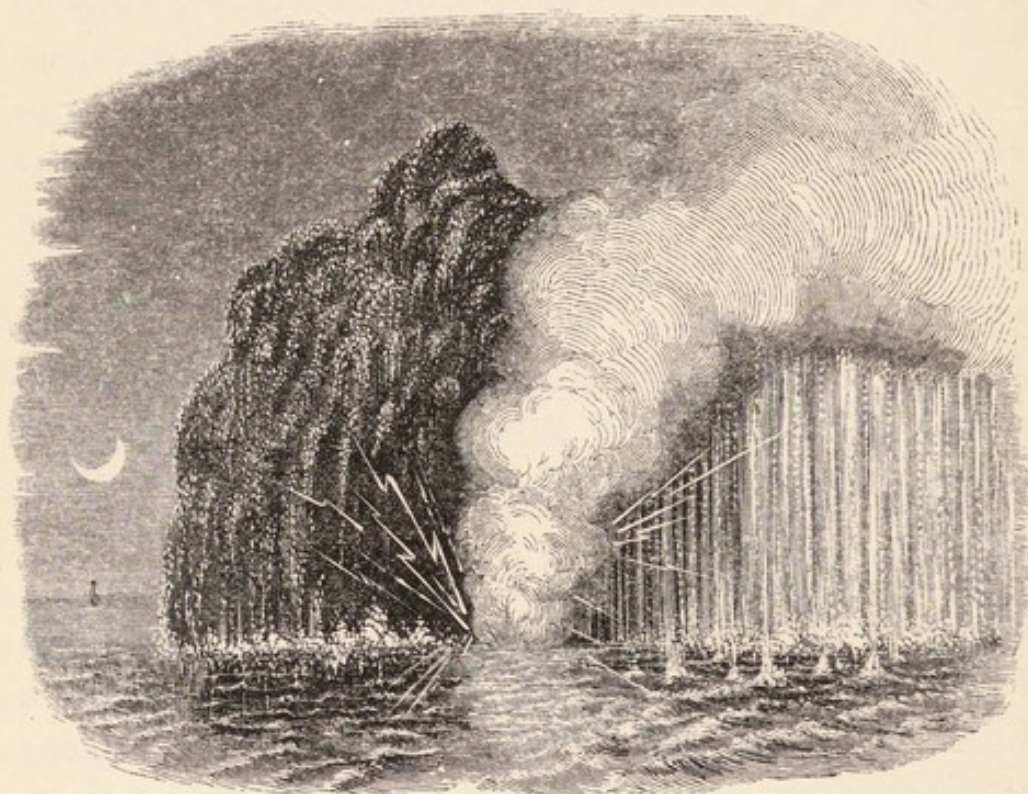
SUBMARINE VOLCANO.
