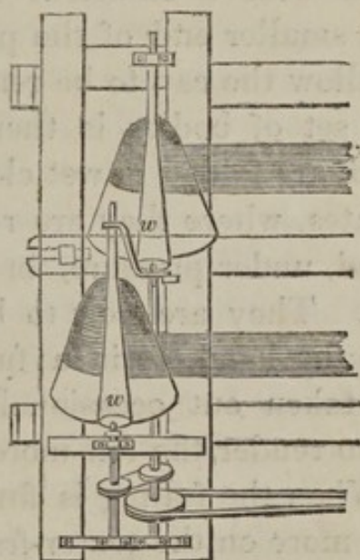
Fig. 34.—Williams's Hat Felter.
