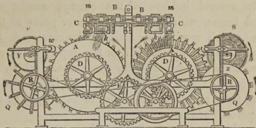
Fig. 39.—Section of Wordsworth's Flax-heckling Machine.
