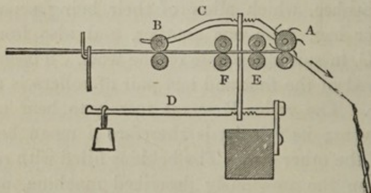
Fig. 29.—Worsted Throstle.
