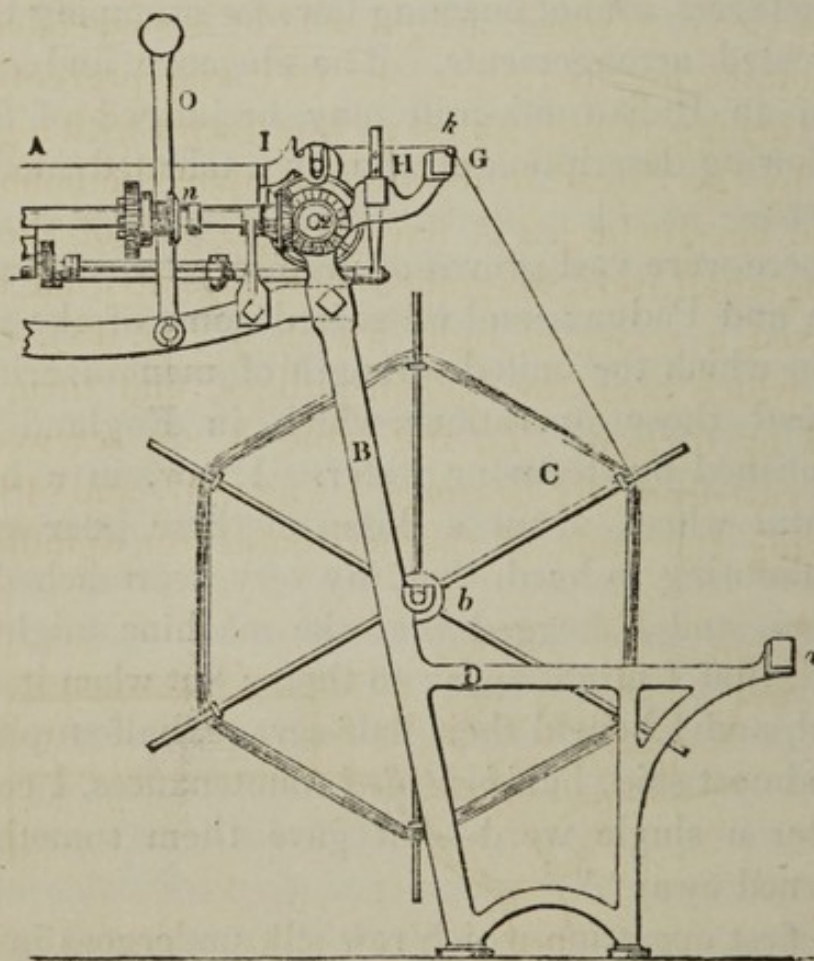
Fig. 47.—Silk Engine, or Swift.
