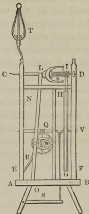
Fig. 44.—Self-acting Flax-wheel.
