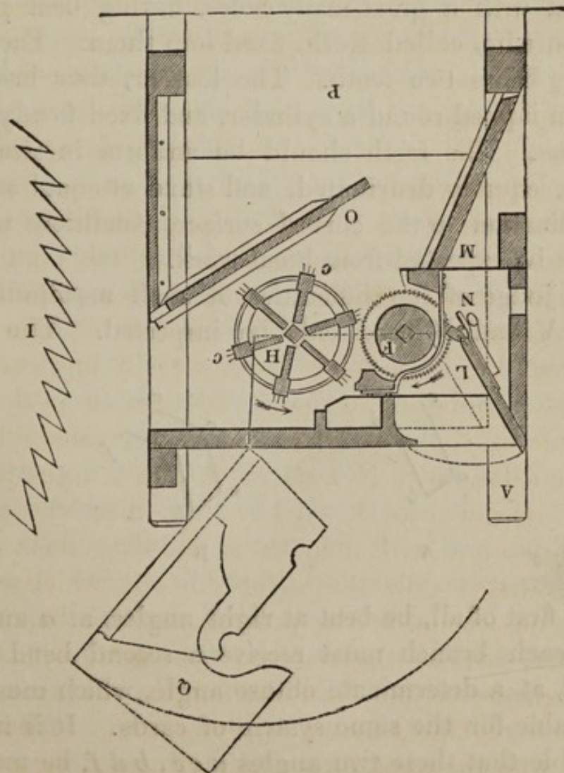
Fig. 17.—Whitney's Saw-gin.
