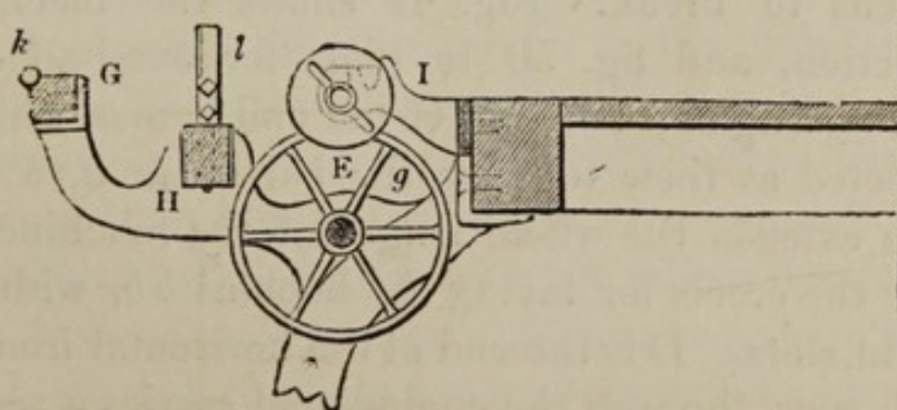
Fig. 48.—Bobbin Mechanism of the Silk Engine.
