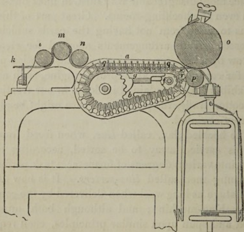
Fig. 40.—Wordsworth's Flax-roving Machine.
