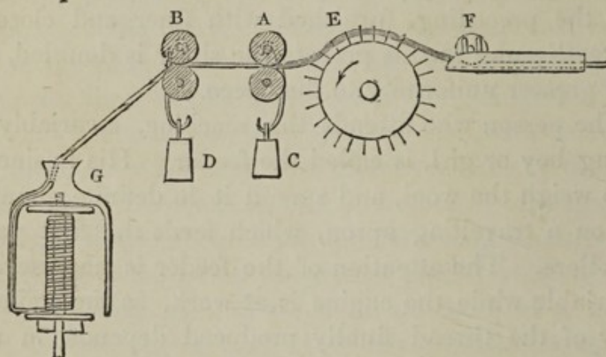
Fig. 27.—Worsted Roving.
