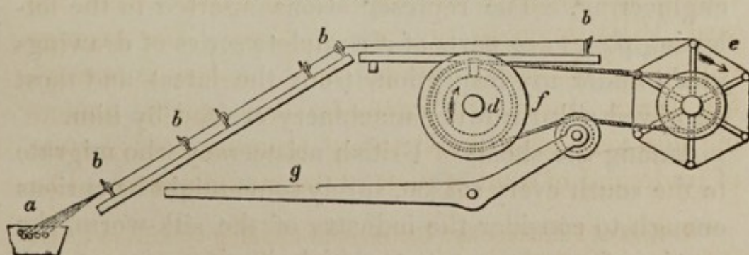
Fig. 46.—Cocoon Filature.—Section of Reel.
