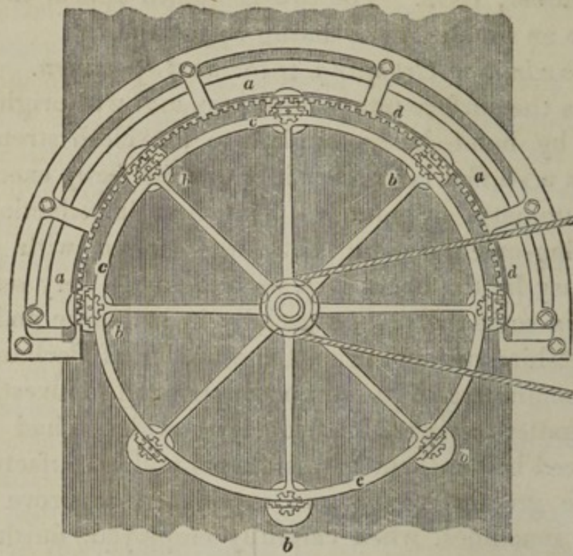
Fig. 37.—Oldland's Cloth-Shearing Machine.
