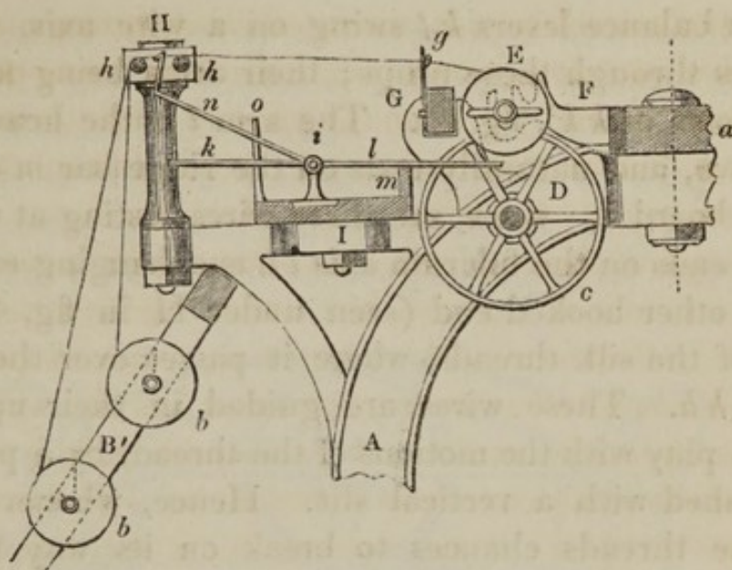
Fig. 49.—Mechanism of Silk Doubling-Mill.—Section.
