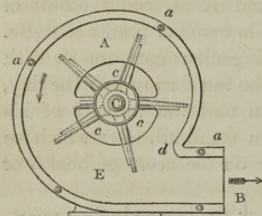
Fig. 56.—Side View of the Ventilating Fan.
