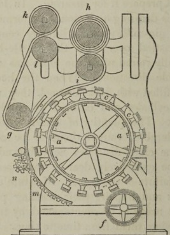
Fig. 35.—Atkinson's and Walker's Gig Mills united.
