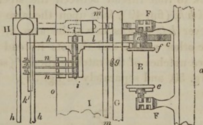
Fig. 50.—Mechanism of Silk Doubling-Mill.—Plan.
