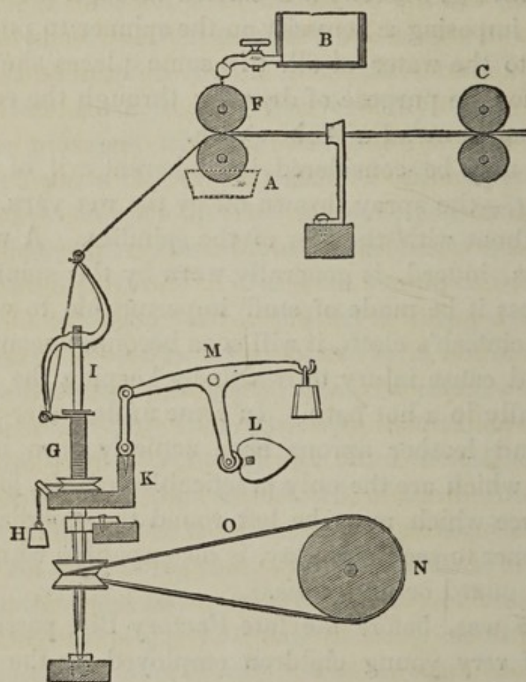
Fig. 43.—Wet Flax Spinning.
