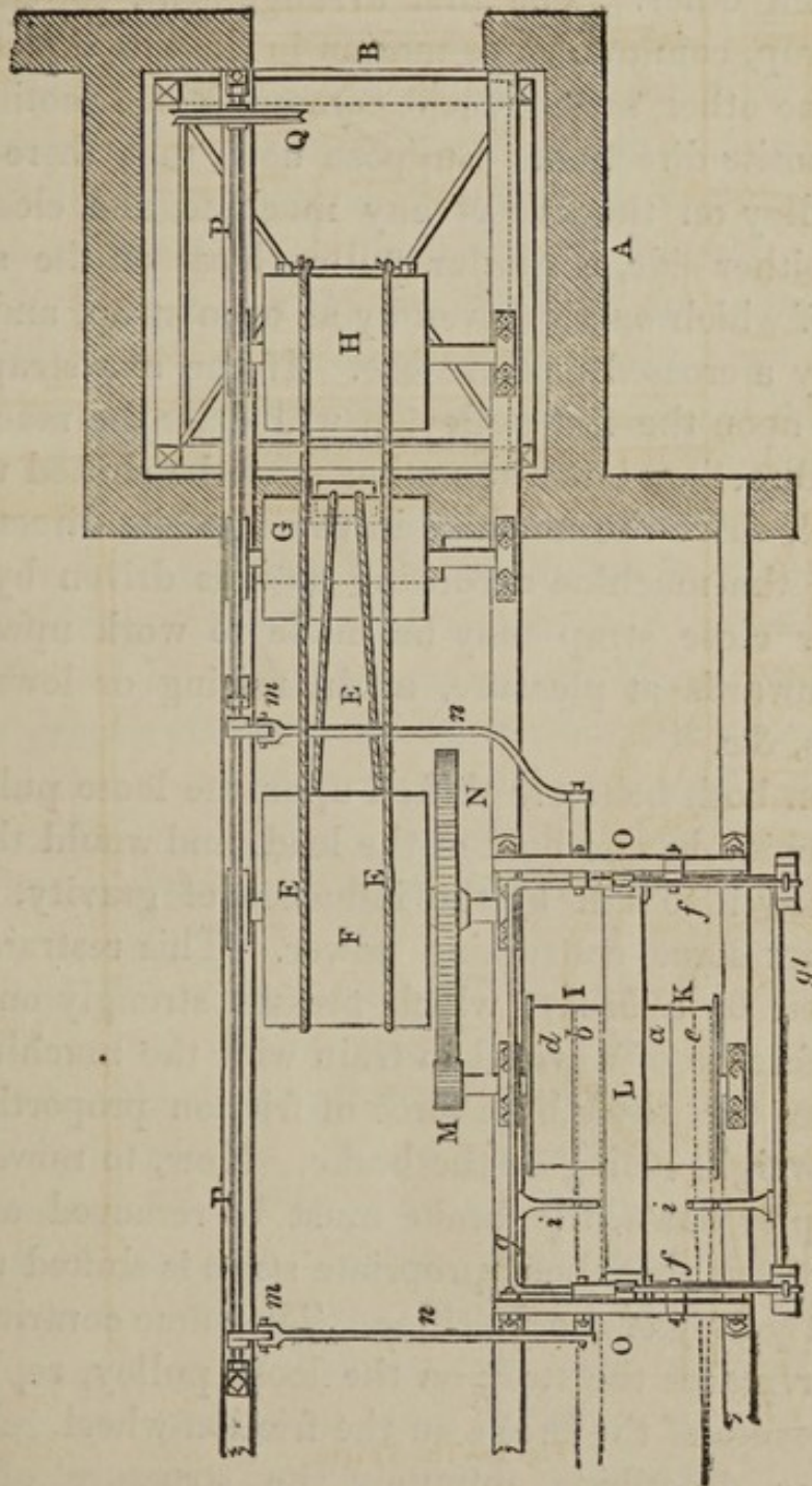
Horizontal Section, or Plan.
