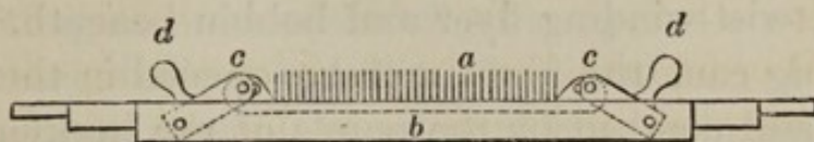
Fig. 41.—Wordsworth's Flax-gill.
