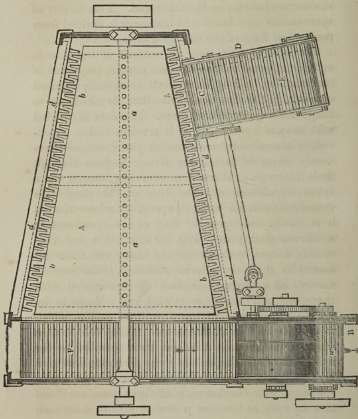
Fig. 30.—Lilly's Conical Willow.
