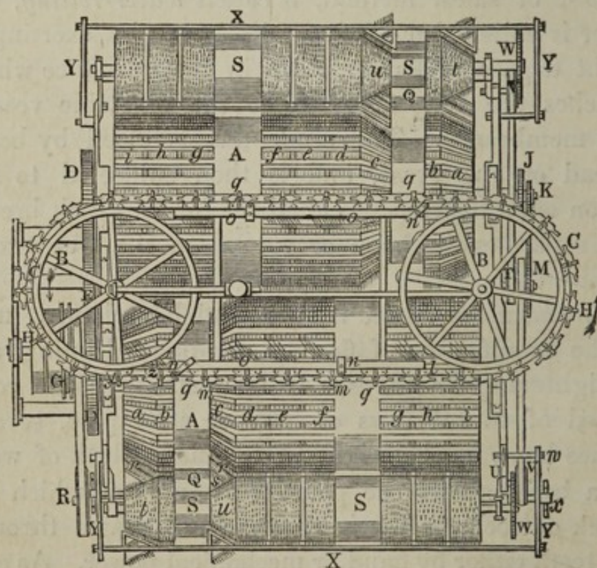
Fig. 38.—Plan of Wordsworth's Flax-heckling Machine.
