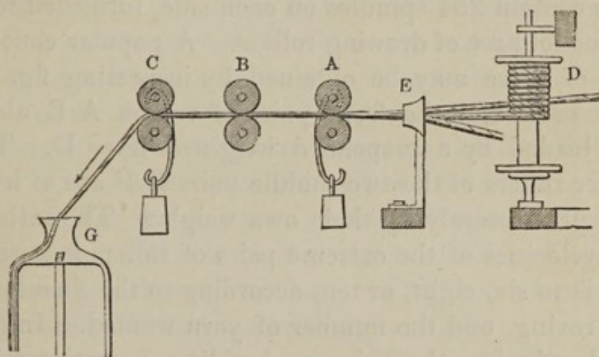
Fig. 28.—Worsted Spinning.
