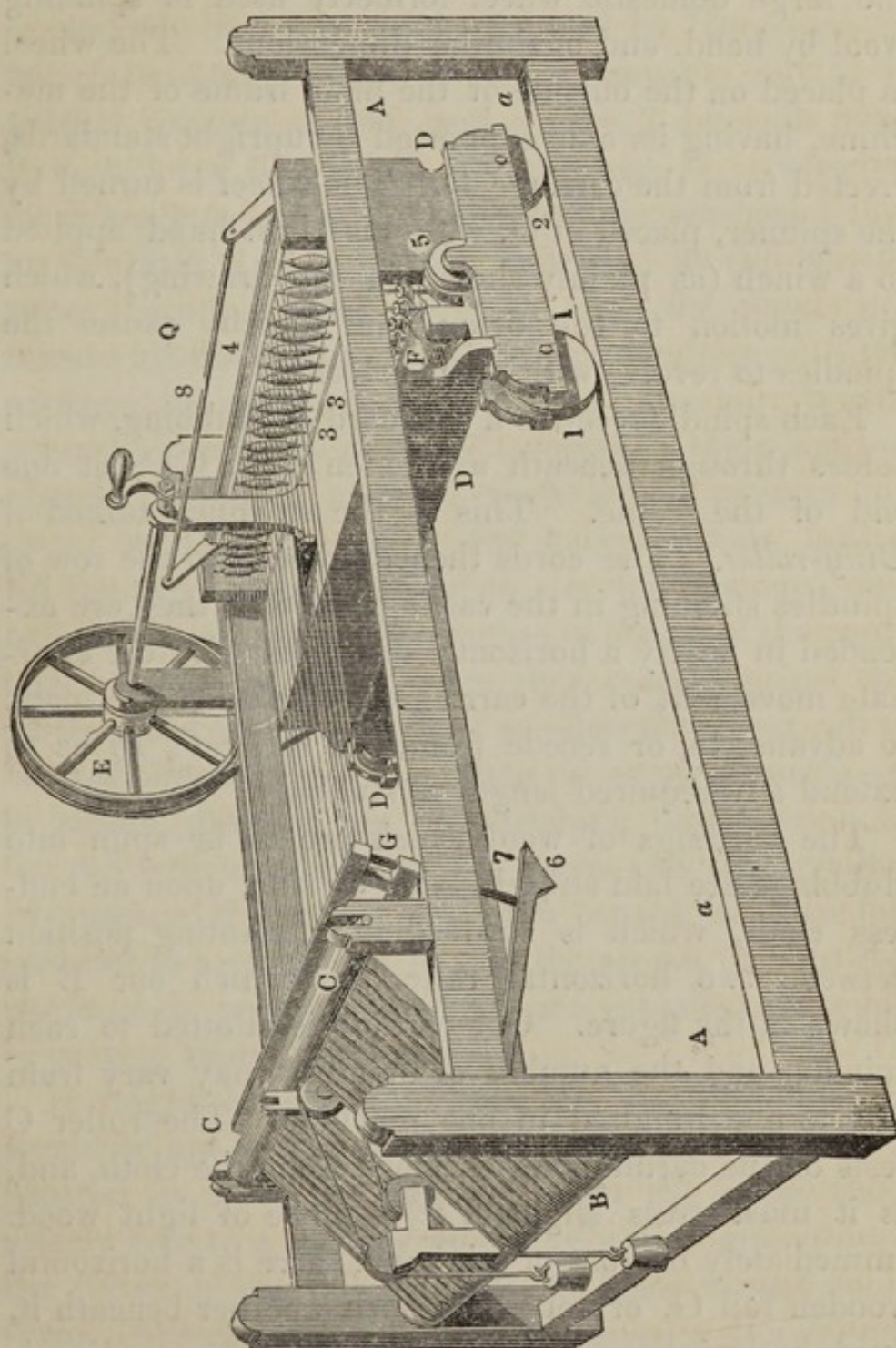
Fig. 31.—Slubbing Billy.
