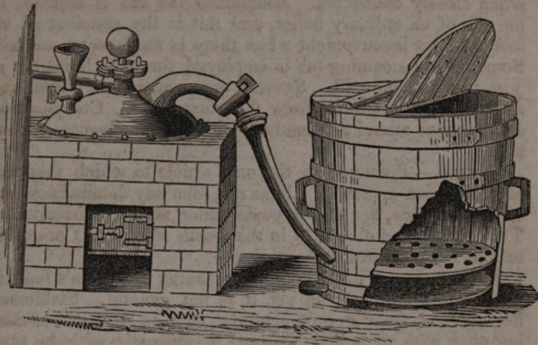
FIG. 17.—STEAMING APPARATUS.
