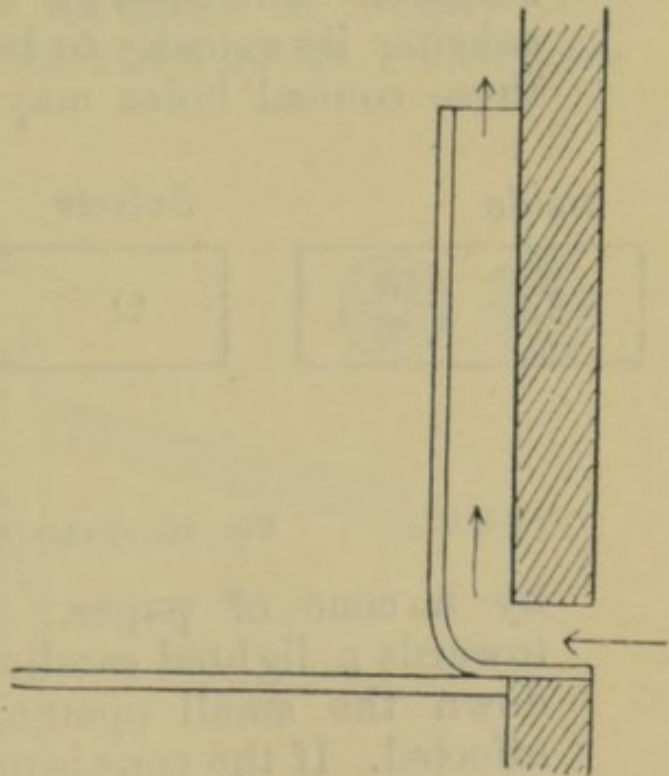
Fig. 40.—TOBIN'S TUBE.
