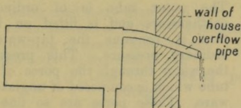
Fig. 97.—OVERFLOW PIPE AS IT SHOULD BE.
