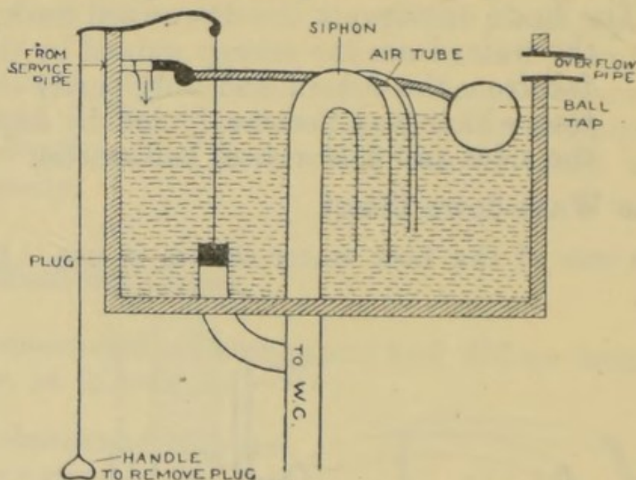
Fig. 108.—FLUSHING CISTERN OR WATER WASTE-PREVENTER.
