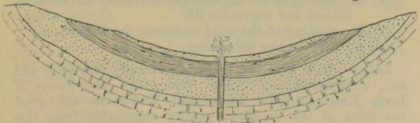
Fig. 94.—AN ARTESIAN WELL.
