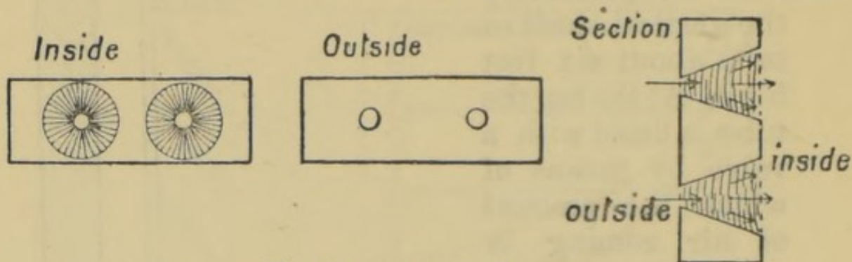
Fig. 42.—ELLISON'S BRICKS.
