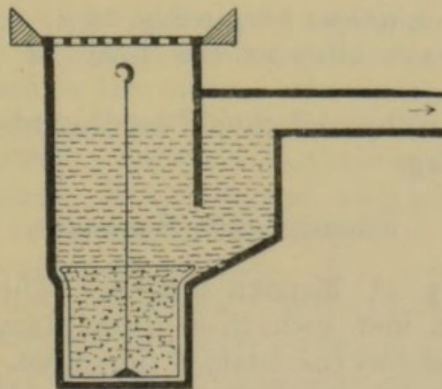
Fig. 113.—GULLY TRAP WITH MOVABLE BUCKET FOR SEDIMENT.
