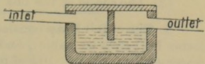
Fig. 110.—THE MID-FEATHER TRAP.
