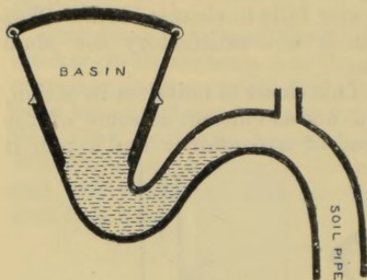
Fig. 105. —SHORT HOPPER CLOSET.
