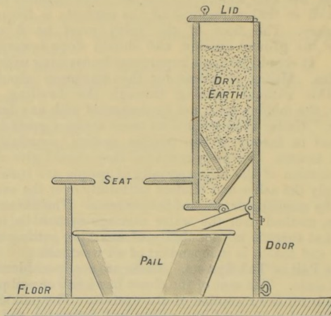
Fig. 114.—AUTOMATIC EARTH CLOSET.
