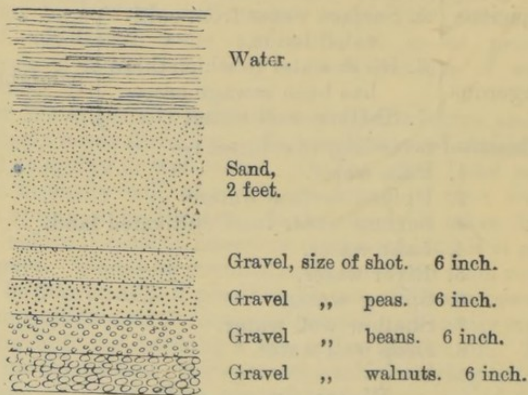
Fig. 95.—A FILTER BED (SECTION).
