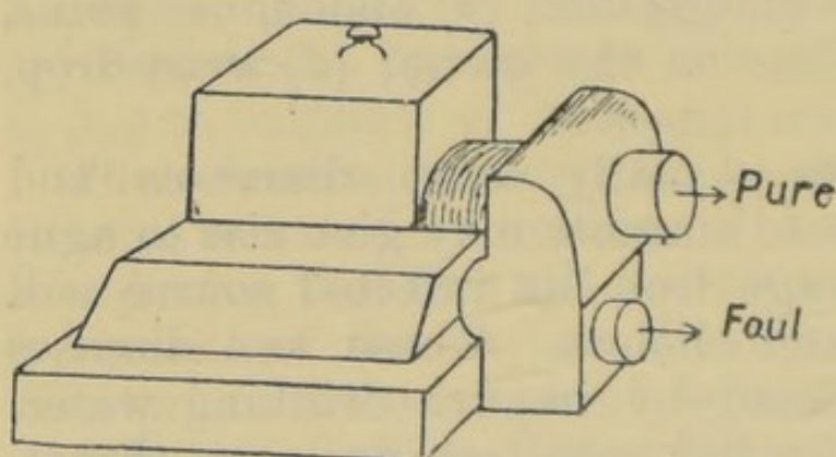
Fig. 88.—RAIN-WATER SEPARATOR.
