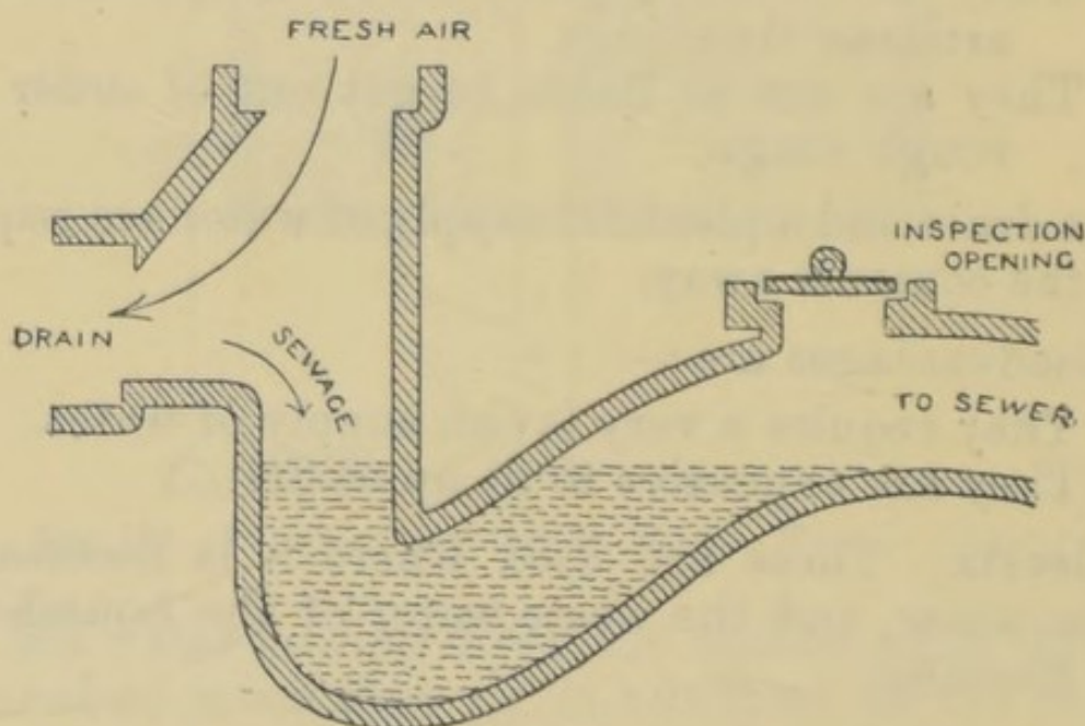
Fig. 109.—BUCHAN'S DISCONNECTING AND VENTILATING TRAP.
