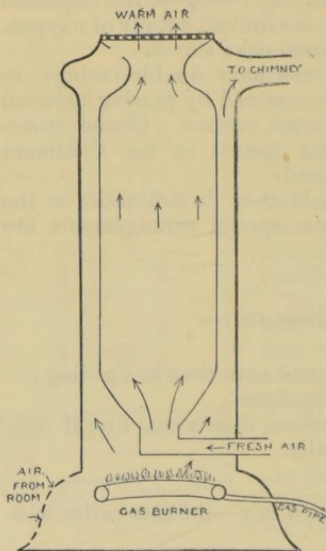
Fig. 100.—VENTILATING STOVE (Bond's).
