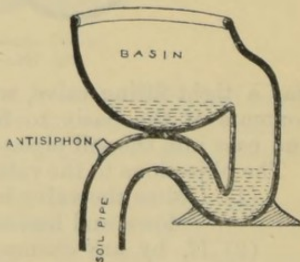
Fig. 106. —WASH-OUT CLOSET.
