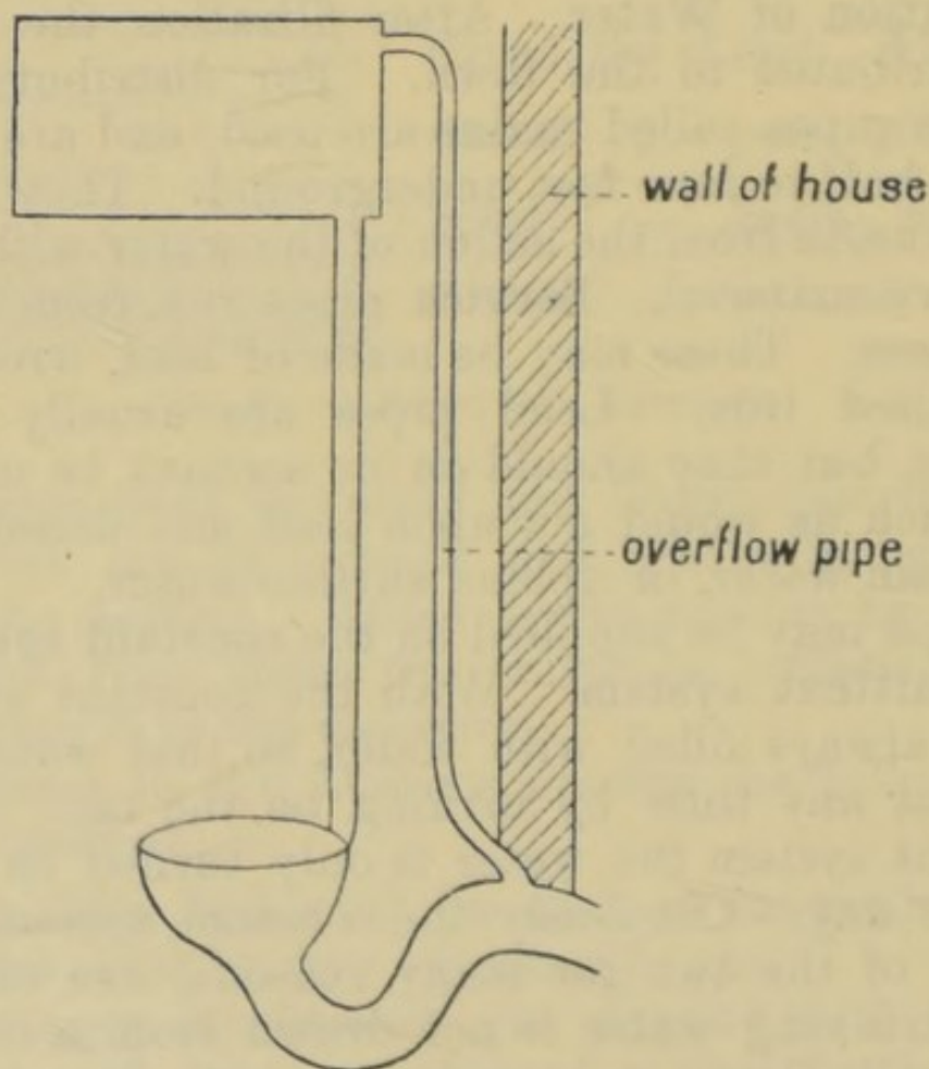
Fig. 96.—OVERFLOW PIPE OF CISTERN WRONG.
