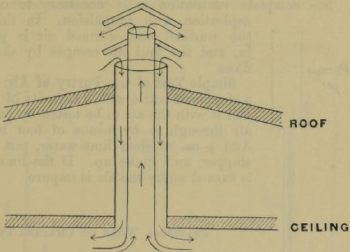
Fig. 44.—McKINNELL'S VENTILATOR.
