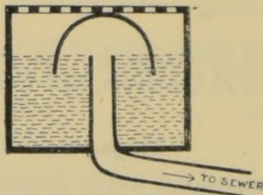
Fig. 111.—THE BELL TRAP.
