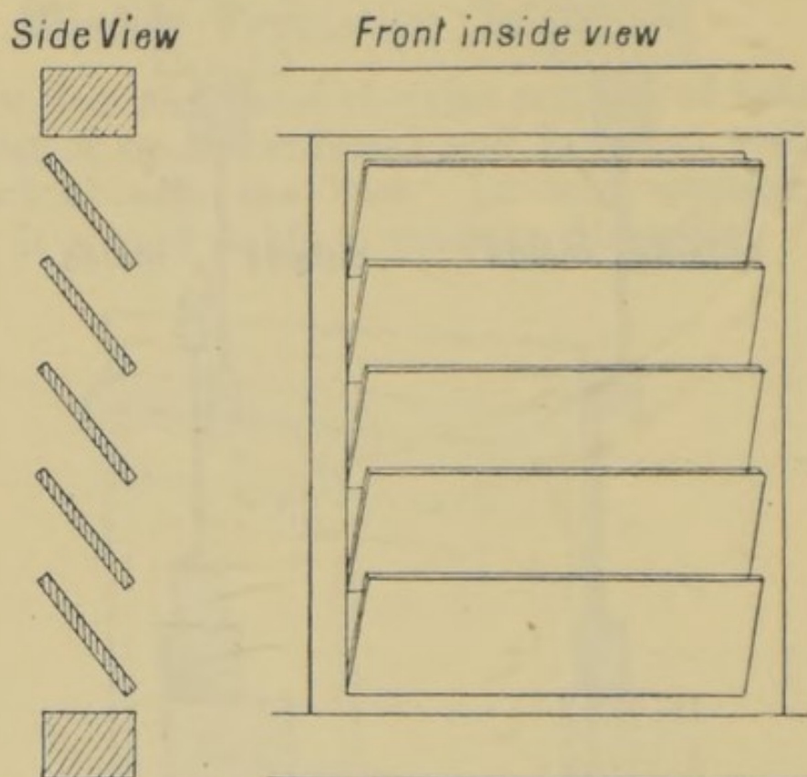
Fig. 38.—THE LOUVRE VENTILATOR.
