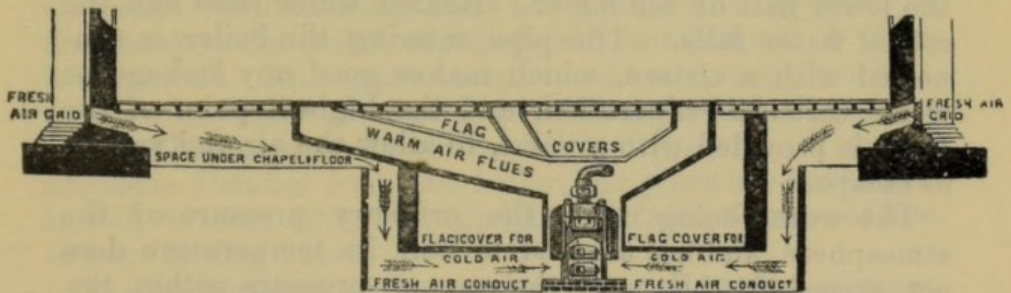
Fig. 101.—To WARM A CHURCH BY HOT AIR.
