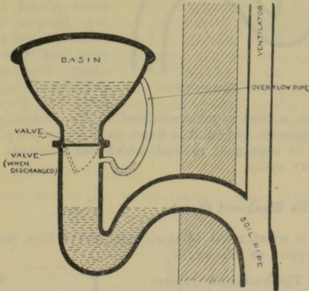
Fig. 104.—VALVE CLOSET
