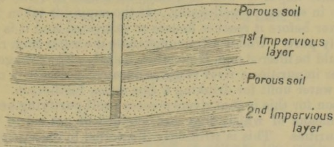
Fig. 93.—DEEP WELL.
