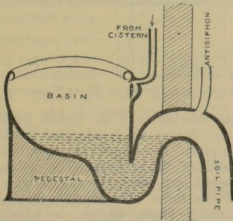
Fig. 107.—WASH-DOWN CLOSET.
