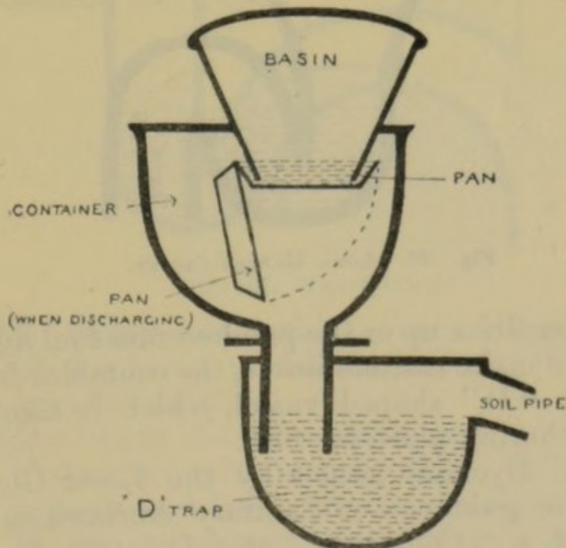
Fig. 102.—PAN CLOSET.
