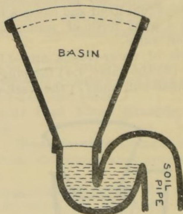
Fig. 103.—LONG HOPPER CLOSET.
