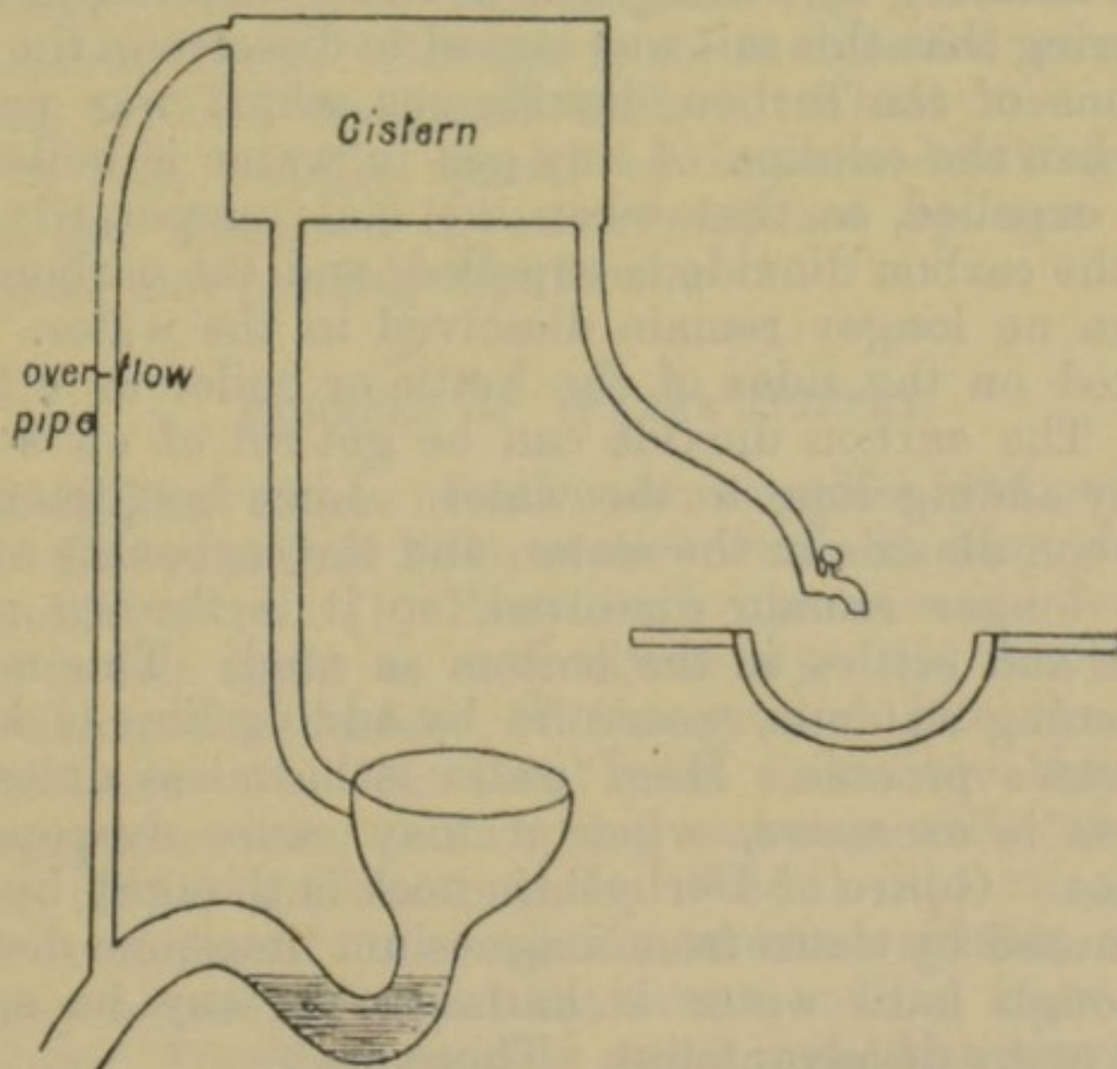
Fig. 87.—CISTERN WITH INSANITARY ARRANGEMENTS.
