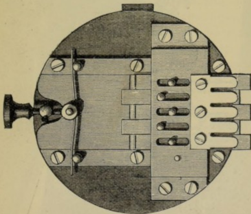
FIG. 33.—Slit allowing five photographs to be taken on the same plate by using successively different portions. Two portions of the slit are shown covered.
