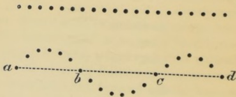
FIG. 11.—Wave Systems.
