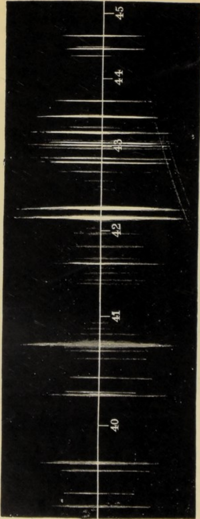
FIG. 17.—Long and short lines.
