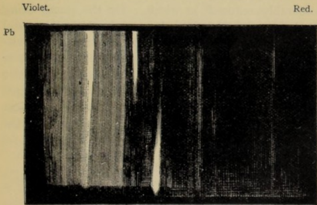
FIG. 45.—Spectrum of Cadmium and Lead.
