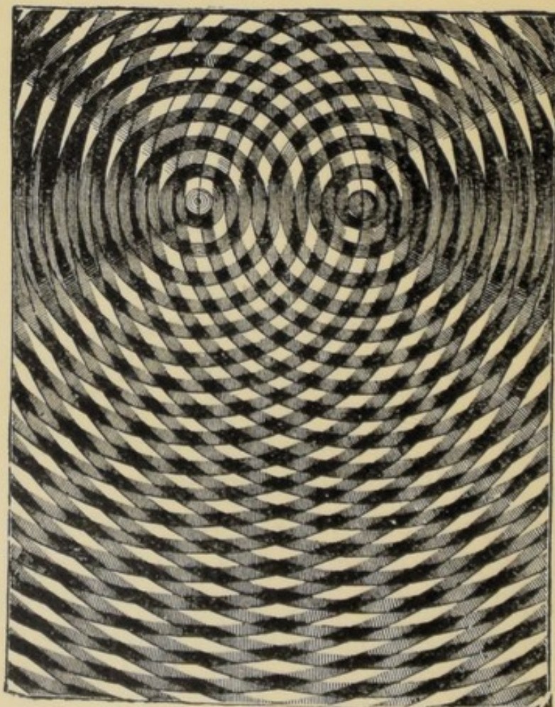
FIG. 1.— Superposition of two wave-systems.
