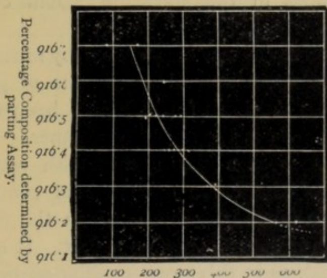
FIG. 51.—Curve B. Gold and Copper Alloys.
