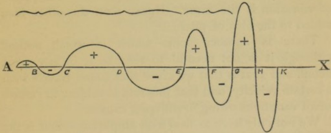
FIG. 10.—Sound waves of different lengths and amplitudes.
