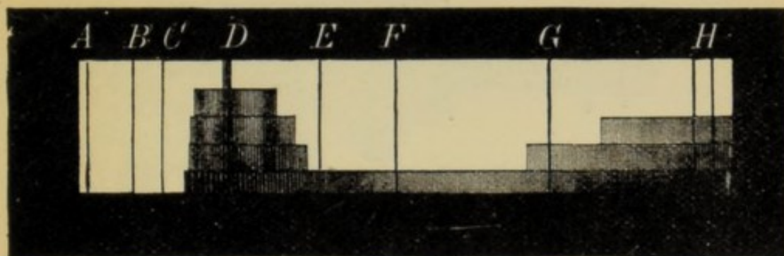
FIG. 24.—Absorption of different thicknesses of the colouring matter of litmus.
