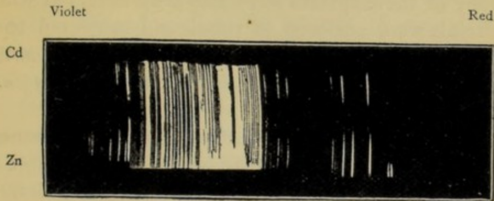
FIG. 44.—Copy of a photograph of the spectrum of the spark between poles of zinc and cadmium, showing the separation of the three spectra.
