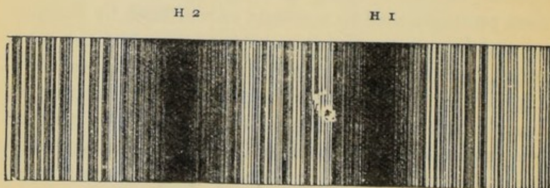
FIG. 29.—The H-lines in the blue end of the solar spectrum, from a photograph by the author.
