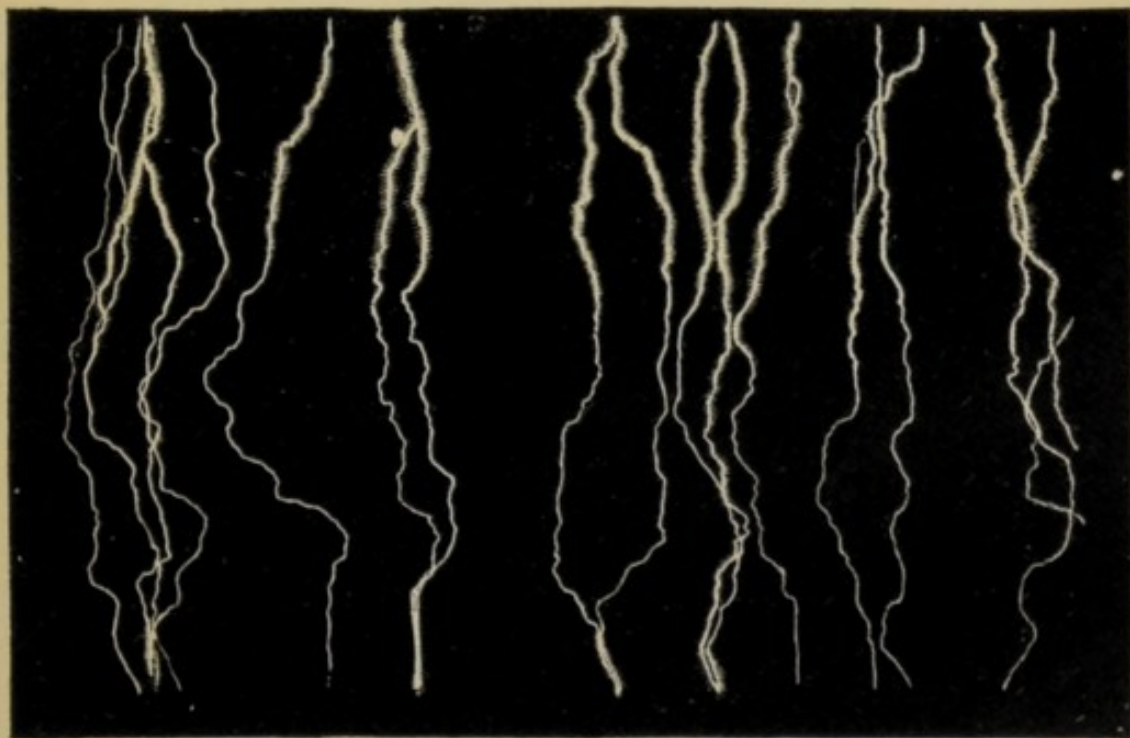
FIG. 40.—Copy of Professor Tait's photograph of the spark in air.
