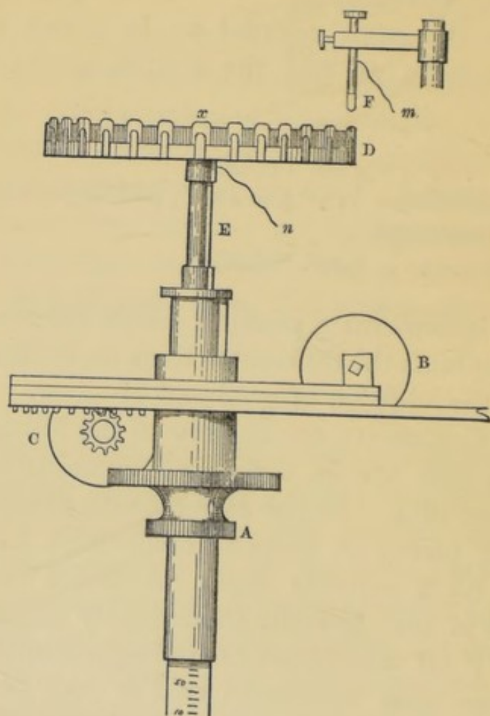
FIG. 48.—SPECIMEN HOLDER. A. Elevating Screw.—B. Rotating Screw.—C. Screw giving side motion.—D. Wheel holding specimens.—F. Upper fixed pole.— m n . Wires to coil.
