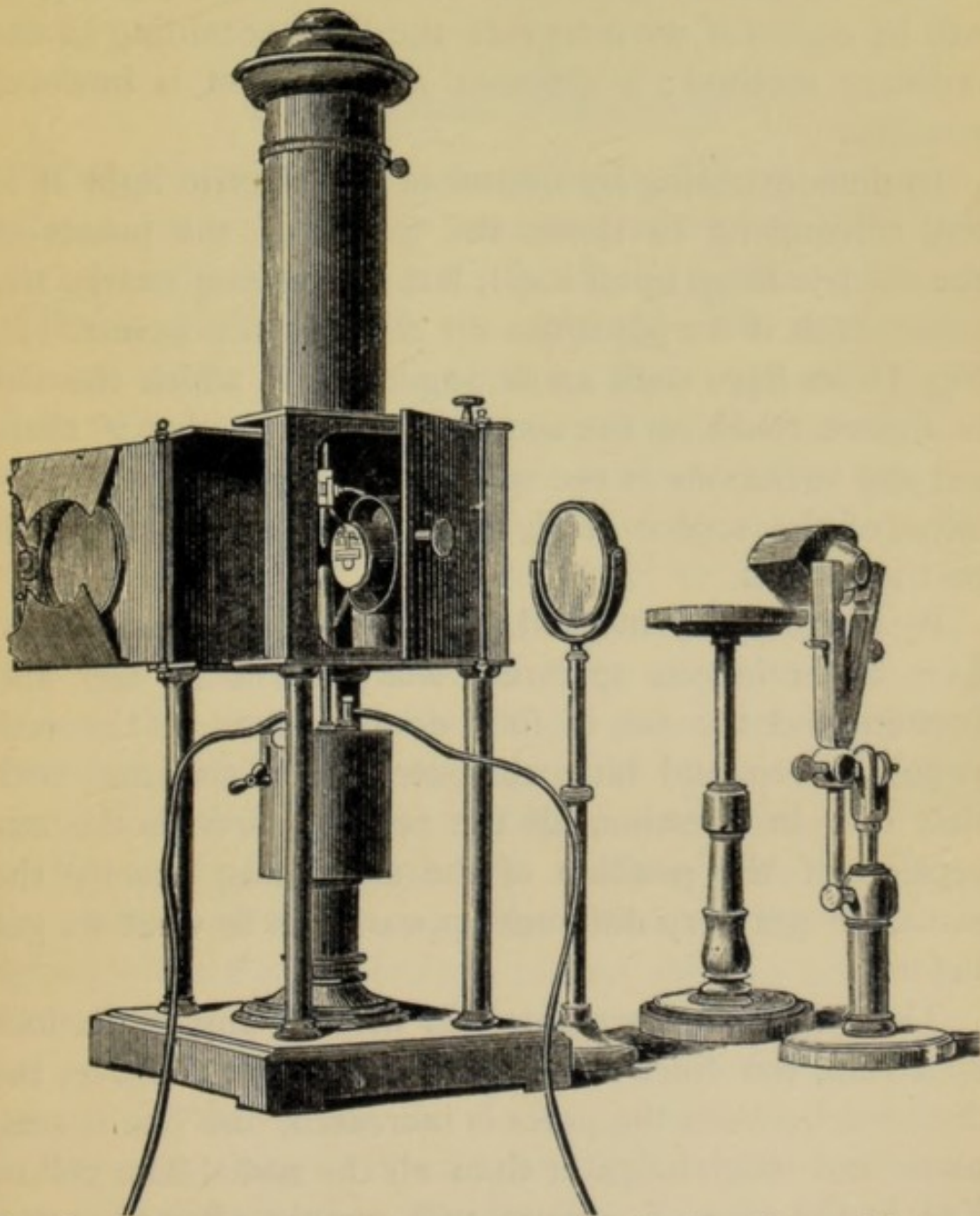
FIG. 18. - Arrangement of electric lamp for demonstrating the existence of long and short lines
