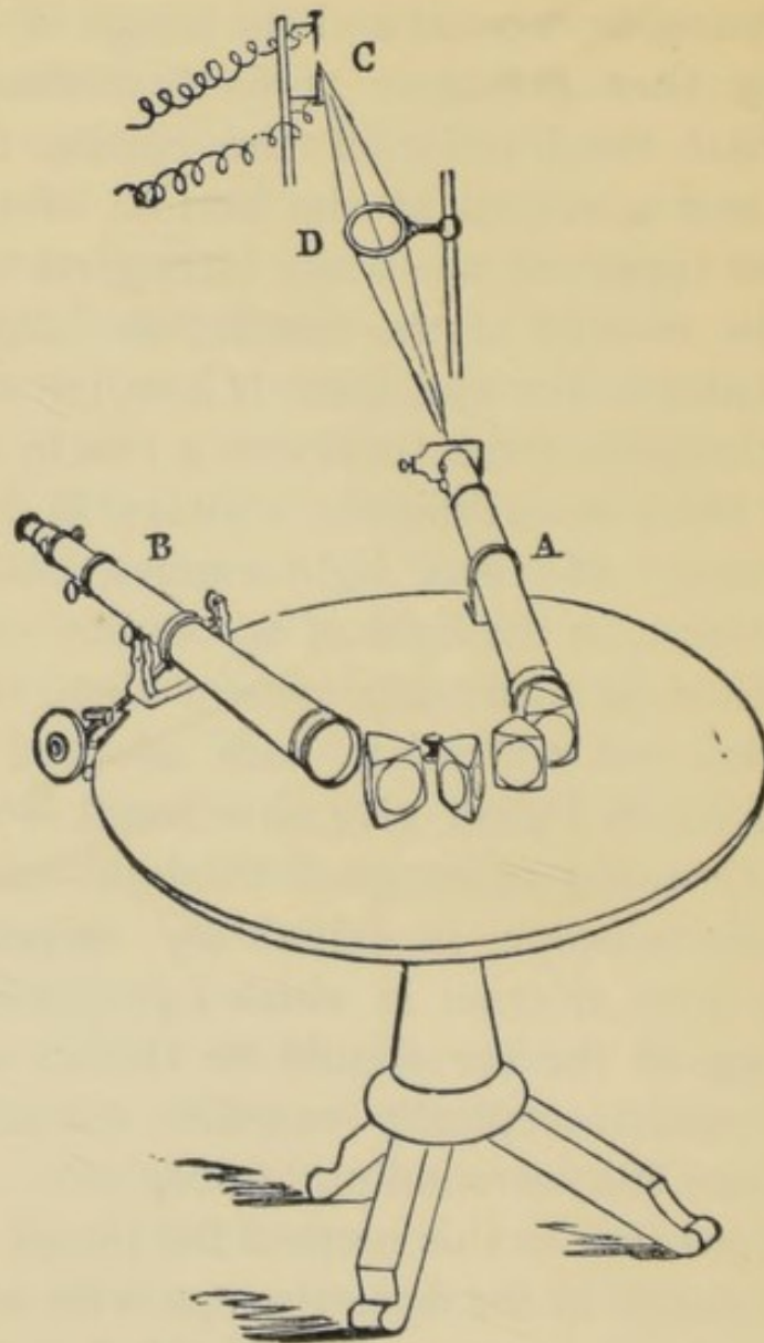
FIG. 14.—The analysing spectroscope
