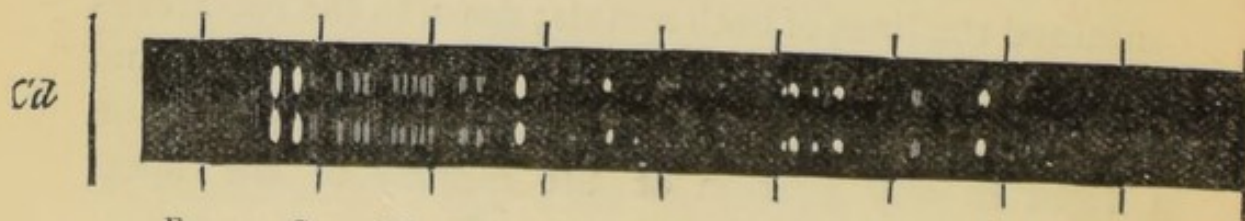
FIG. 43.—Copy of Dr. Miller's Spectrum of Cadmium, showing the "dots."
