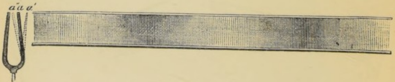
FIG. 5.—Propagation of sound waves along a cylinder.
