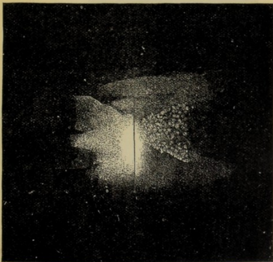
FIG. 16.—Image of horizontal arc of sodium vapour thrown on a vertical slit (from a photograph).
