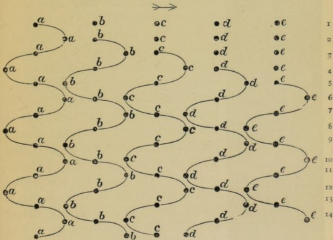
FIG. 6.—Sound Waves. Particles of air, a , b , c , d , e , are in position 1 at rest. The remaining positions show how they are situated at successive instants, when a continuous series of impulses reaches them from the left. In position 2, e.g. , only one particle has begun its oscillation. In position 3, only two, while in position 6, all are in motion.
