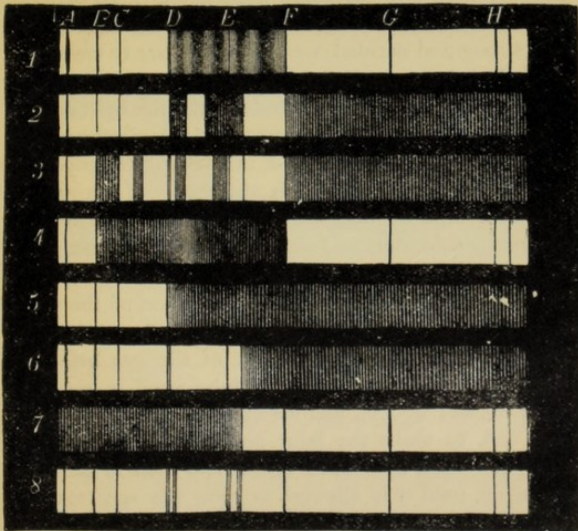
FIG. 23.—Diagram illustrating the various kinds of absorption, and the characteristic absorption of some bodies. 7, Absorption of the red end of the spectrum; 5 & 6, absorption of the blue end; 1, special absorption of permanganate of potash; 2, ditto of blood; 3, ditto of chlorophyll; 4, ditto of cobalt glass (the characteristic structure is not given); 8, ditto of didymium glass.
