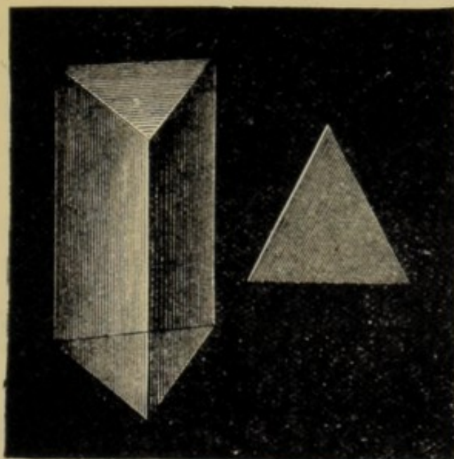
FIG. 12.—The prism.
