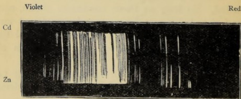
FIG. 15.—Copy of a photograph of the spectrum of the spark between poles of zinc and cadmium, showing the separation of the three spectra.
