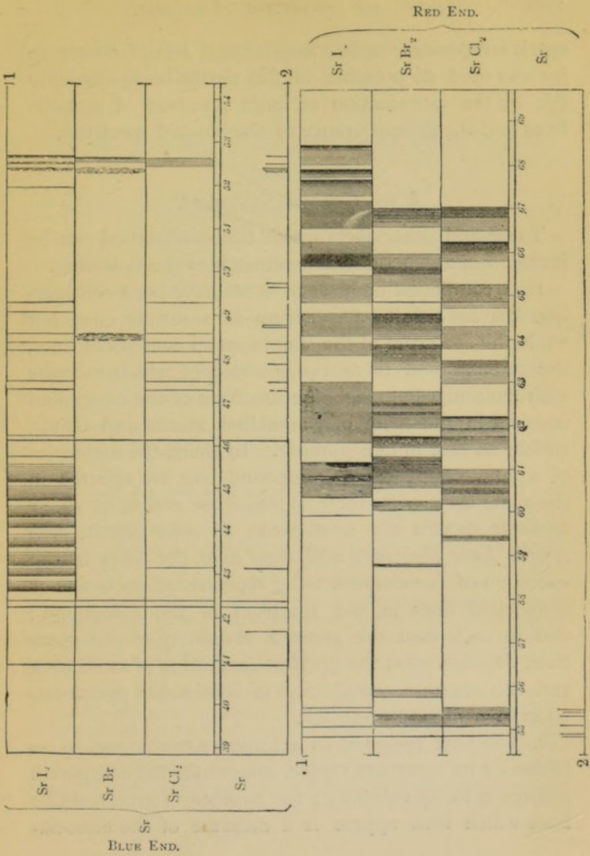
FIG. 46. Spectra of the Salts of Strontium.
