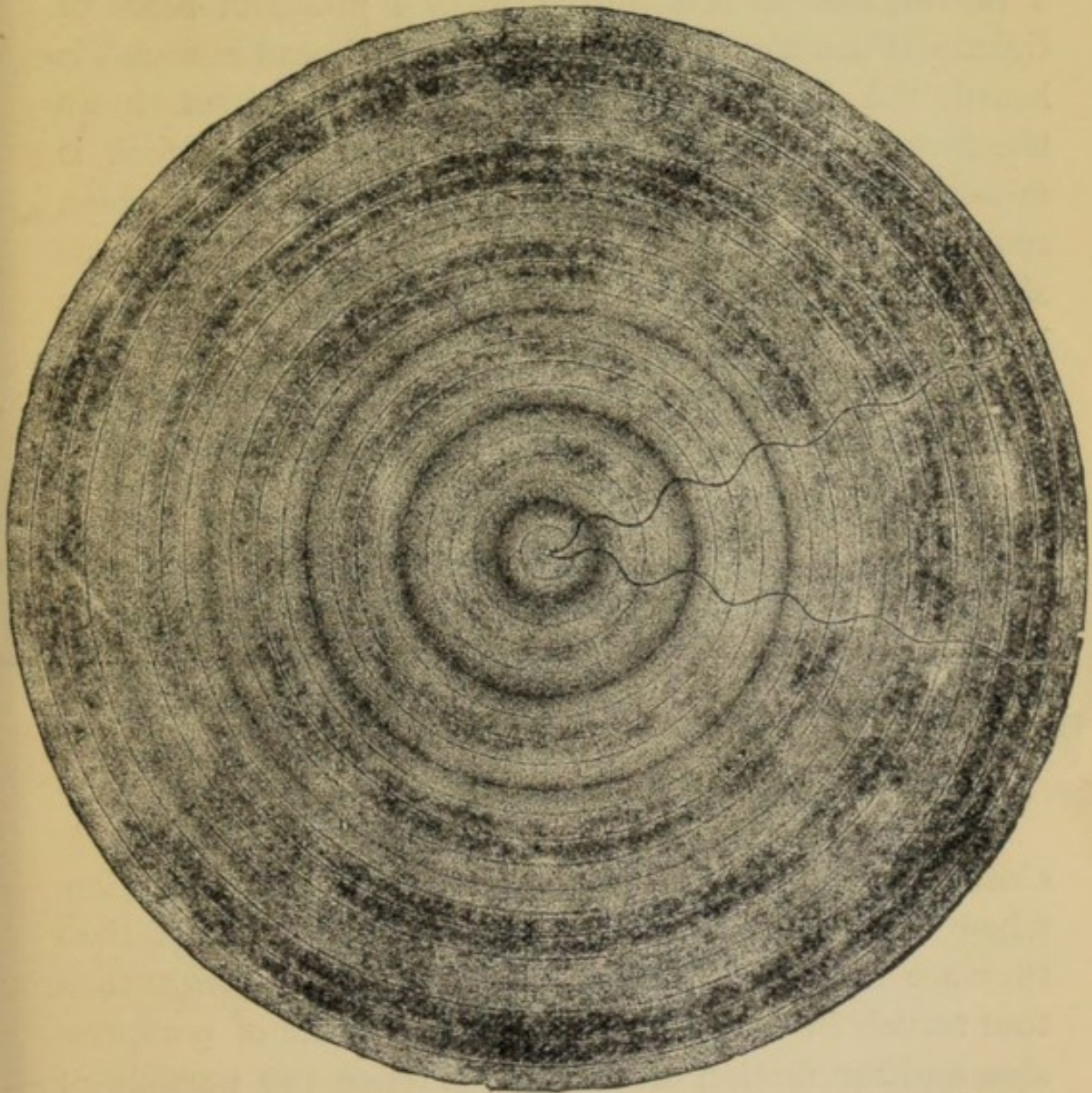
FIG. 4.—Shells of compressed and rarefied air produced by a source of sound.
