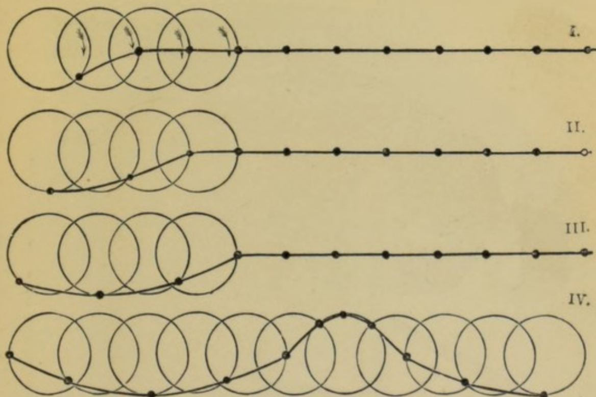
FIG. 2.—Showing the formation of waves by the circular motion of each particle of water in a vertical plane. Eight positions in each revolution are shown.
