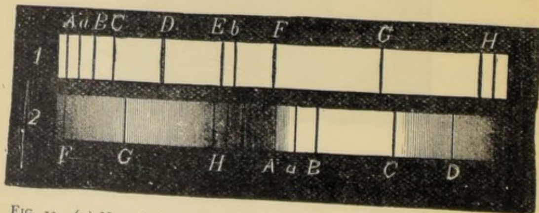
FIG. 13.—(1) Normal dispersion of glass.—(2) Abnormal dispersion of Fuchsine. A a B C, Red.—D, Yellow.—E F, Green.—G, Blue.—H, Violet.
