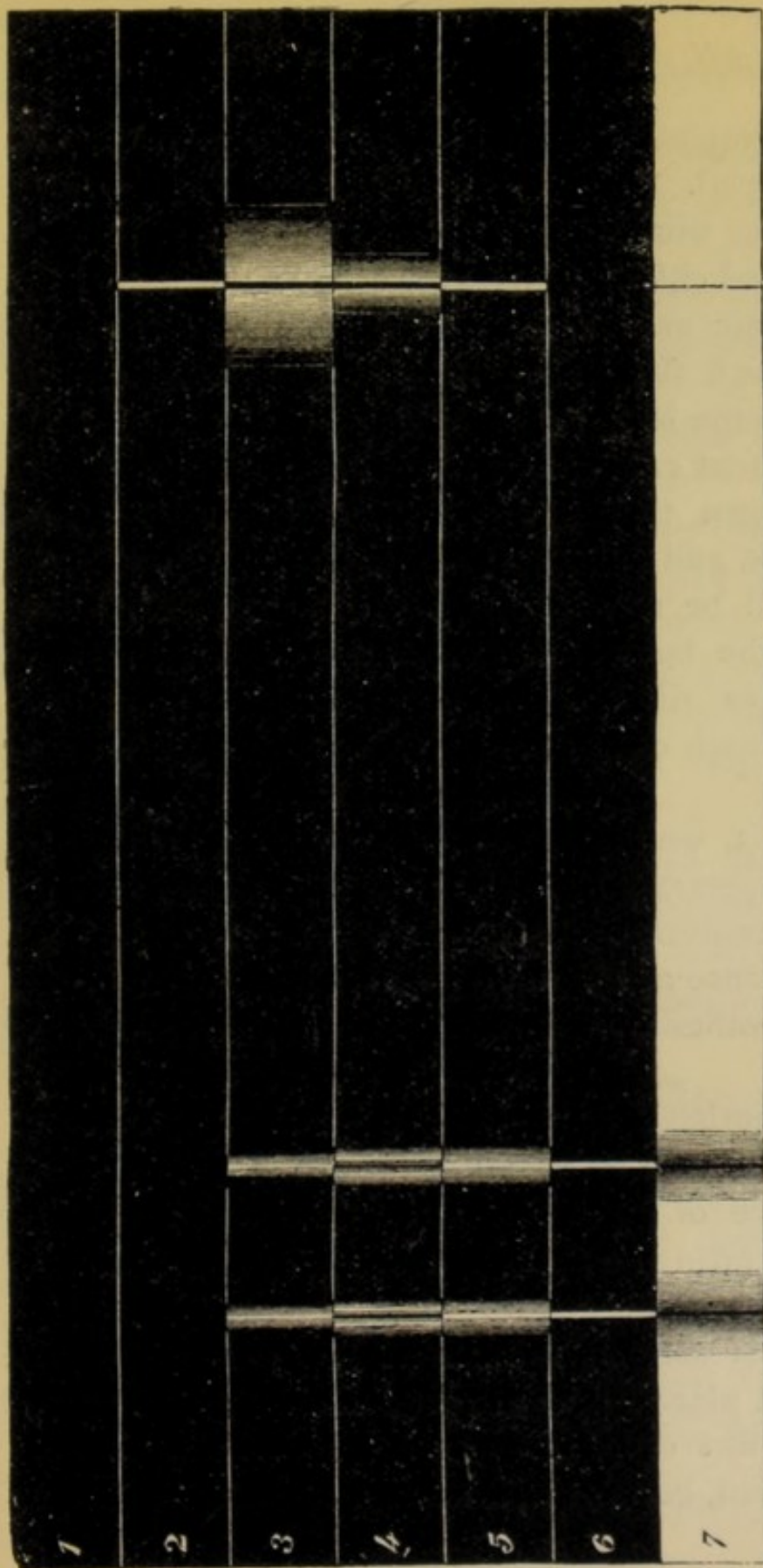
FIG. 47. The blue end of the spectrum of calcium under different conditions.
