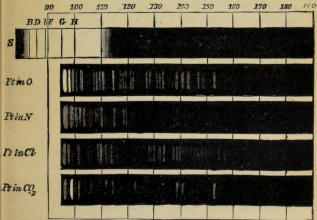
FIG. 32*.—Copies of Dr. Miller's maps of the ultra-violet spectrum of platinum in various gases showing the length of the solar and ultra-violet spectrum.
