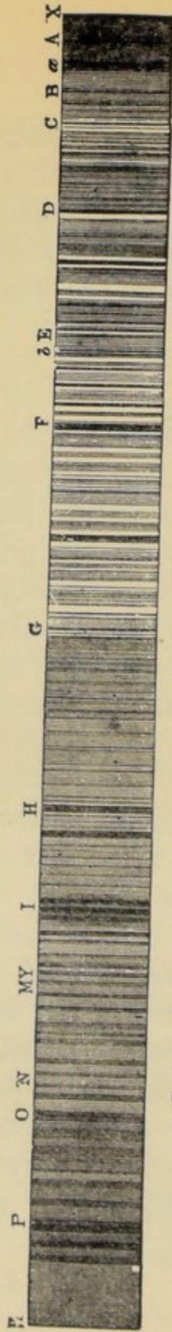
FIG. 27.—Reduced copy of Becquerel's photograph of the complete solar spectrum taken in 1842.
