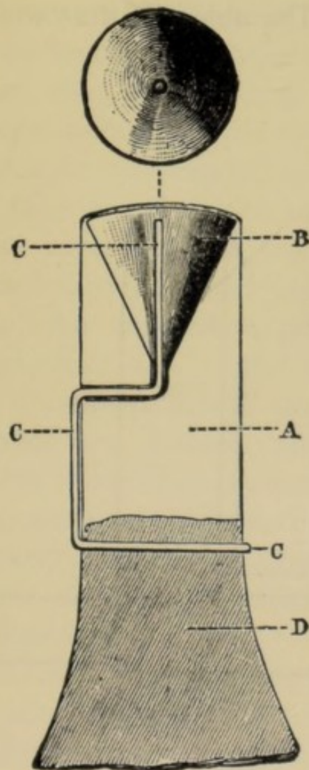
FIG. 19.—Plan and section of cup used with salts. A, aluminum wire; B, cup-shaped cavity drilled in it; C, platinum wire; D, flattened and split portion of the aluminium wire.
