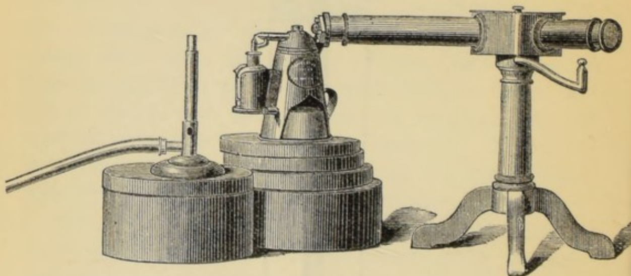
FIG. 22.—Examination of the spectra of solution by blowing the solute into the Bunsen flame by means of a "spray inhaler."
