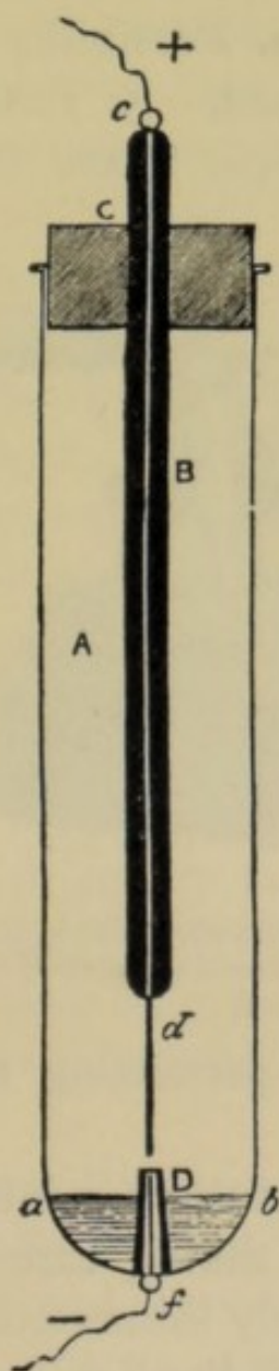
FIG. 21.—A, tube, 11 mm. high, into which the liquid to be analysed is poured; B, capillary tube in which is fixed the platinum wire c d , which forms the upper electrode; C, cork stopper closing the tube A—it supports B, and permits its being moved with little friction; D, small capillary tube, slightly conical, covering the lower electrode f ; d , upper electrode; f , lower electrode; a b , level of liquid.
