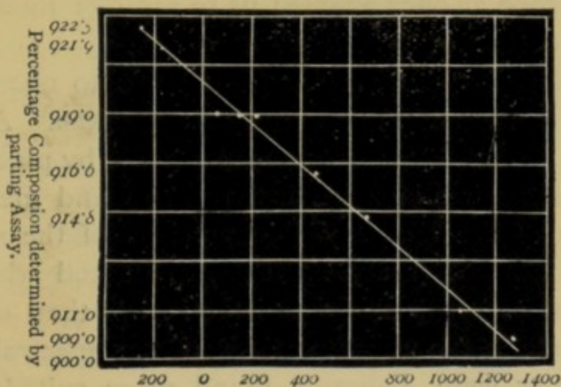
FIG. 50.—Curve A. Gold and Copper Alloys.
