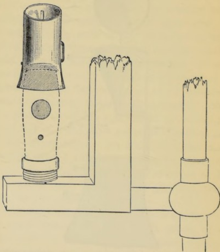
FIG. 20.—Aluminium cup placed in the spark-stand as in use.
