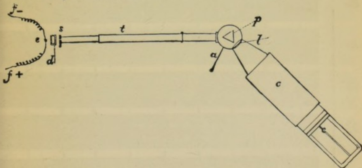
FIG. 30.—Dr. Miller's arrangements,— s , slit; l , quartz lens; c , camera; p , quartz prism; t , collimator; e , spark.
