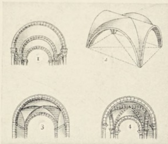
FIG. 161.—TYPES OF VAULTS.
