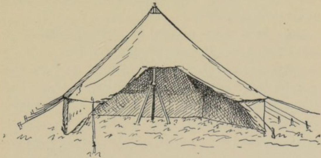
Fig. 29.—Pyramidal tent, with tripod support (United States Army standard model for fixed camps).
