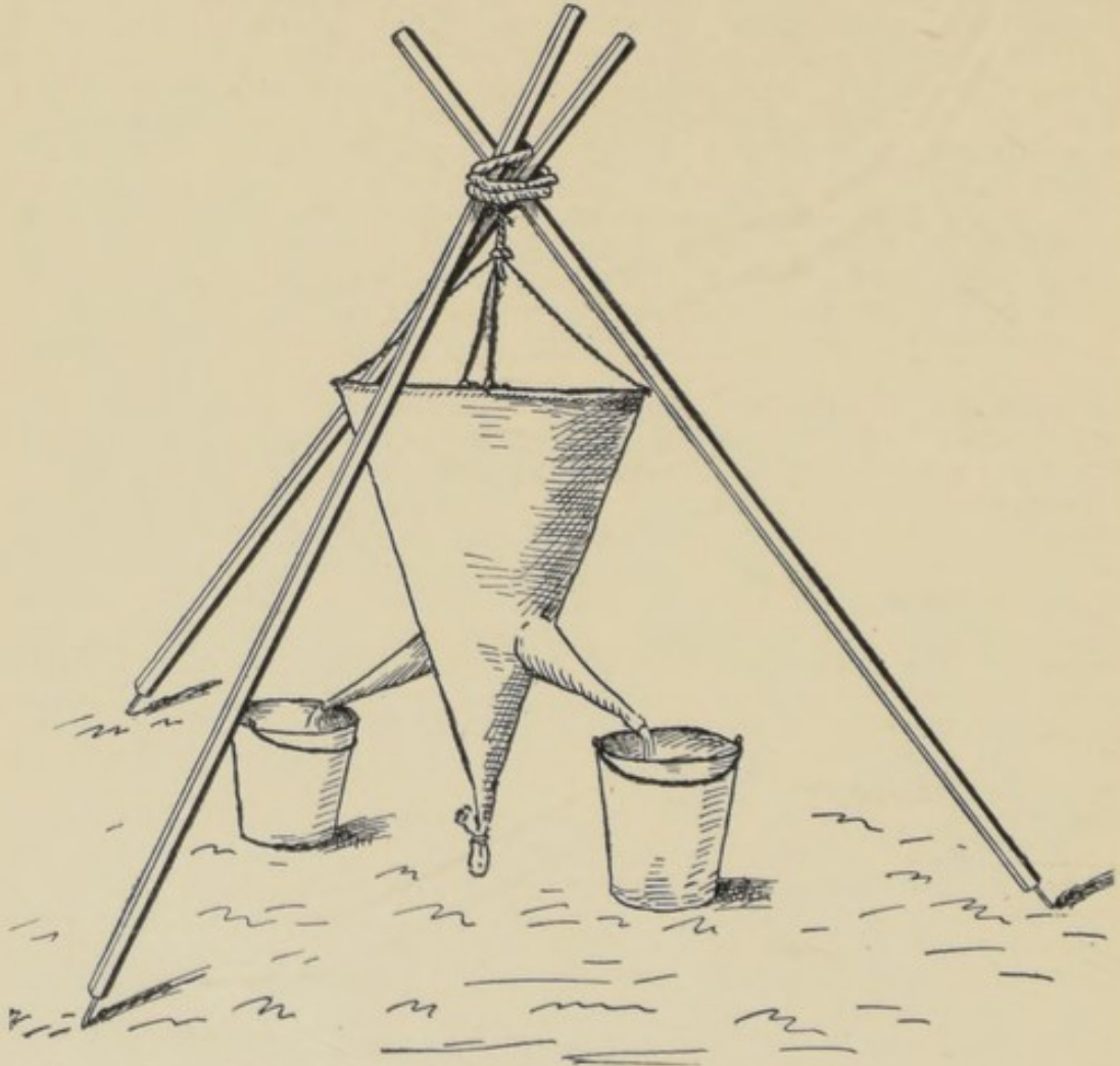
Fig. 16.—Ishiji filter (Japanese model).
