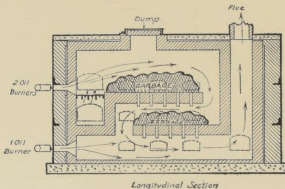
Fig. 37.—Morse-Boulger destructor, longitudinal section.
