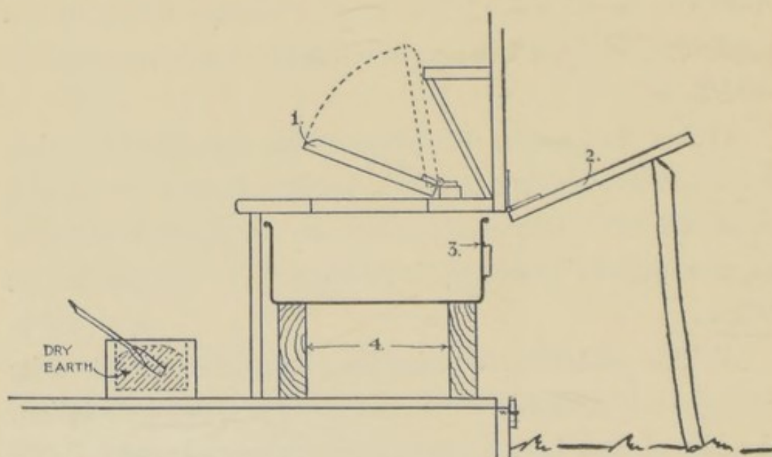
Fig. 34.—Dry earth closet: 1, Self-closing seat cover; 2, fly-tight trap-door; 3, pan; 4, supports for pan.
