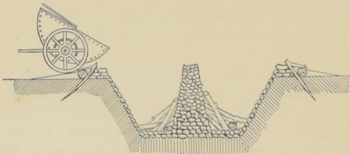
Fig. 46.—Circular pit (rock pile) crematory (after Wilson).
