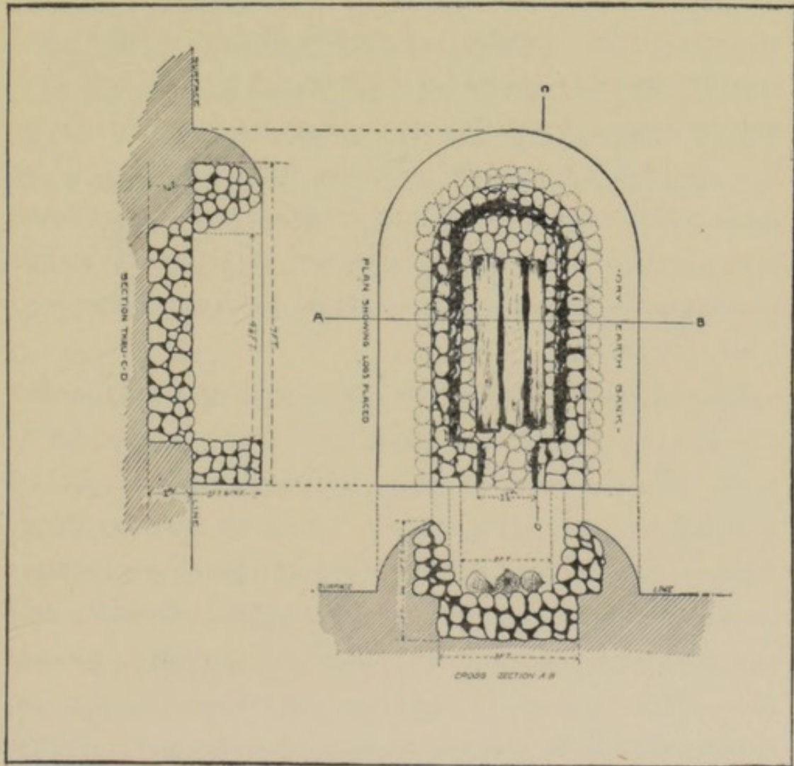
Fig. 45.—Company mess incinerator (Straub).
