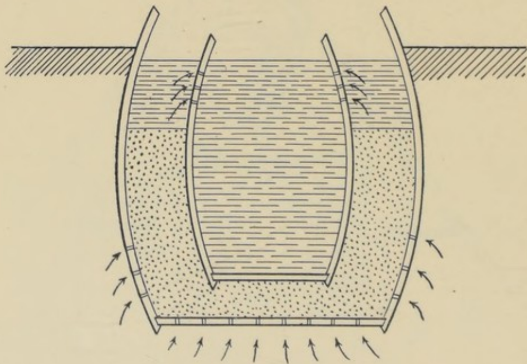
Fig. 18.—Barrel filter sunk in spring.
