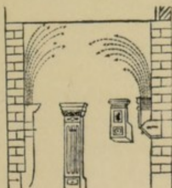
TOBIN'S TUBE INLETS.
