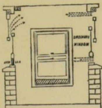
HINCKES-BIRD'S WINDOW INLET.
