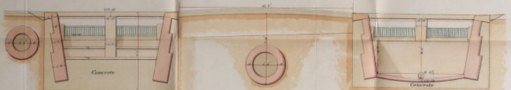
SECTION C. C.
