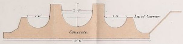
CROSS SECTION OF MAIN DELIVERING CONDUIT & CARRIERS.
