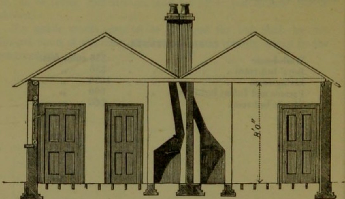
Plate II. Section.
