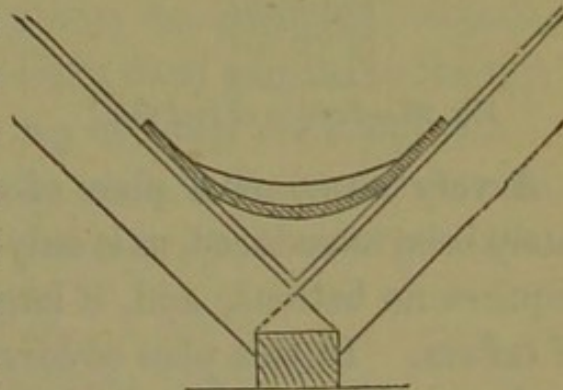
Fig. 28.—Section of valley tile.
