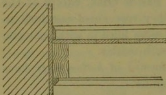
Fig. 25.—Section.
