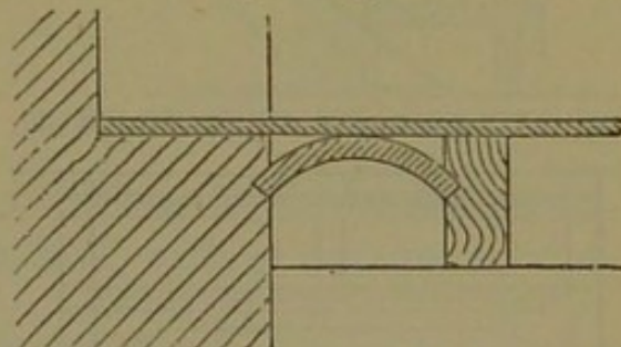
Fig. 23.—Section of tile trimmer.
