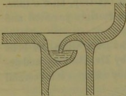
Fig. 7.—Section of bell-trap.
