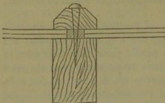
Fig. 31.—Section of slate roof.
