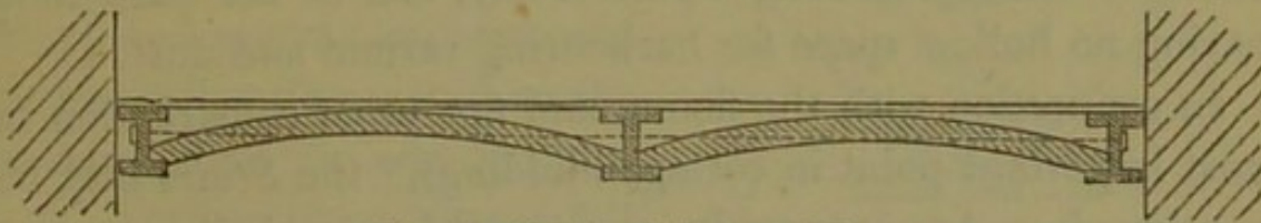
Fig. 22.—Section of fire-proof floor.
