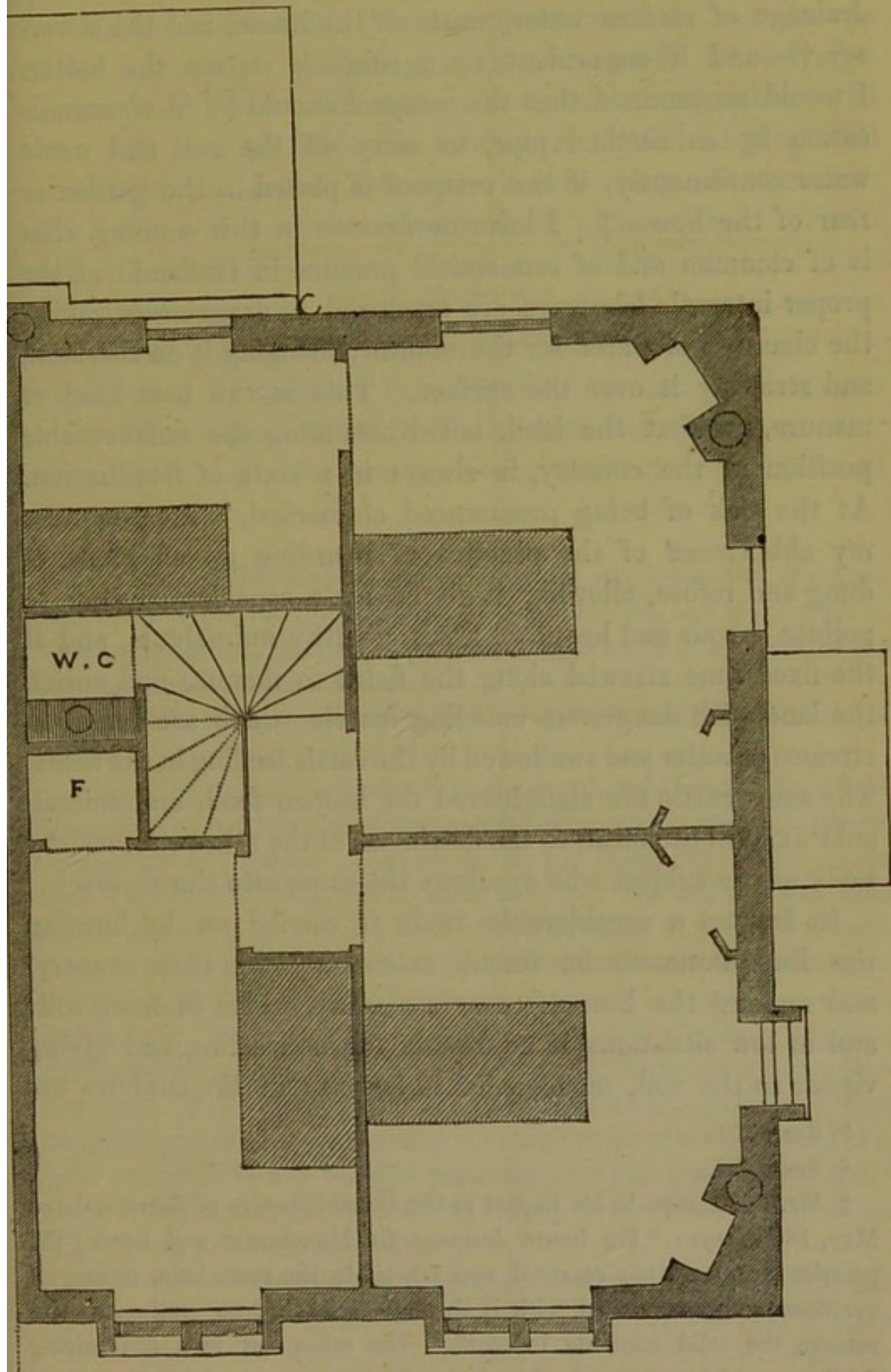
Plate IV. Chamber Floor. w. c. Water-closet.
