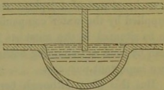
Fig. 2.—Section of drain-trap.
