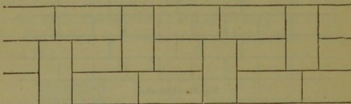
Fig. 16.—Hollow brick wall, 14 inches thick.
