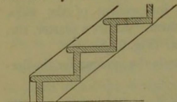
Fig. 26.—Section of stairs formed of tile.
