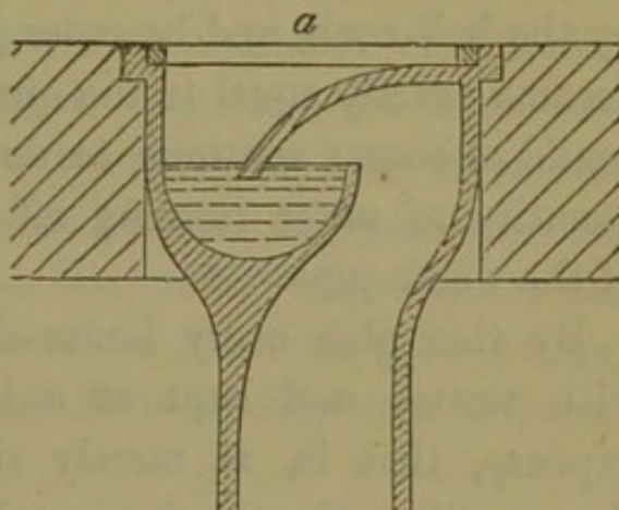
Fig. 4.—Section of drain-trap.
