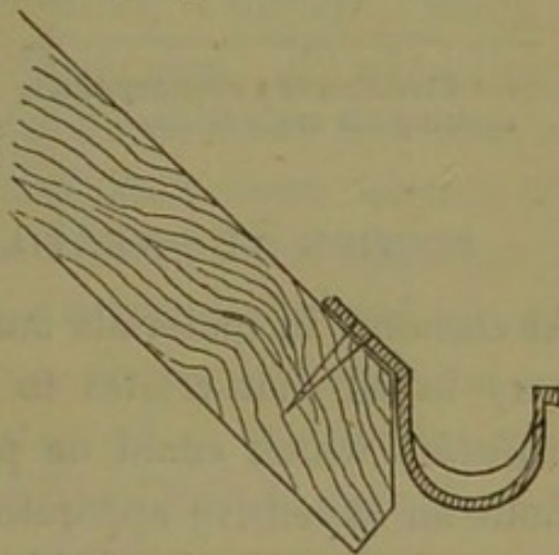
Fig. 33.—Section of tile eaves-gutter.
