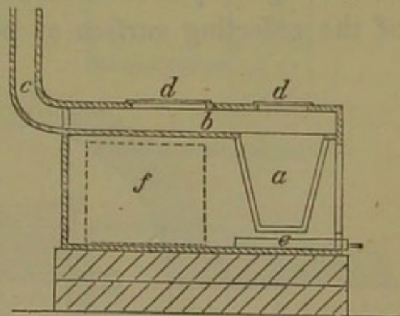
Fig. 38.—Section of cottage cooking-stove.
