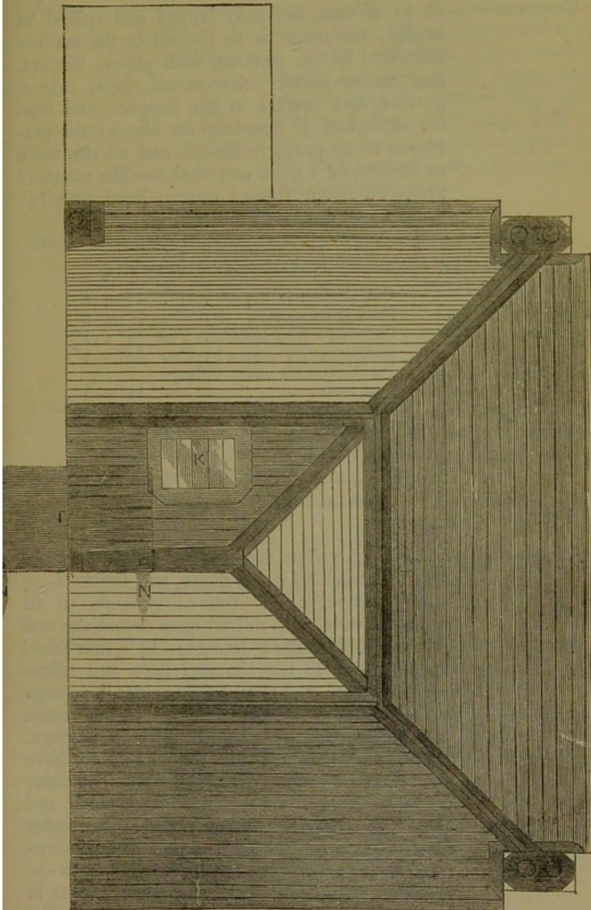
Plate X. Plan of Roofs.
