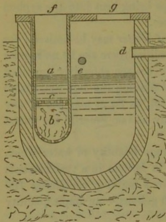
Fig. 8.— Section of rain-water filter.
