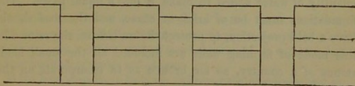
Fig. 14.—Loudon's hollow brick wall, 11 inches thick.
