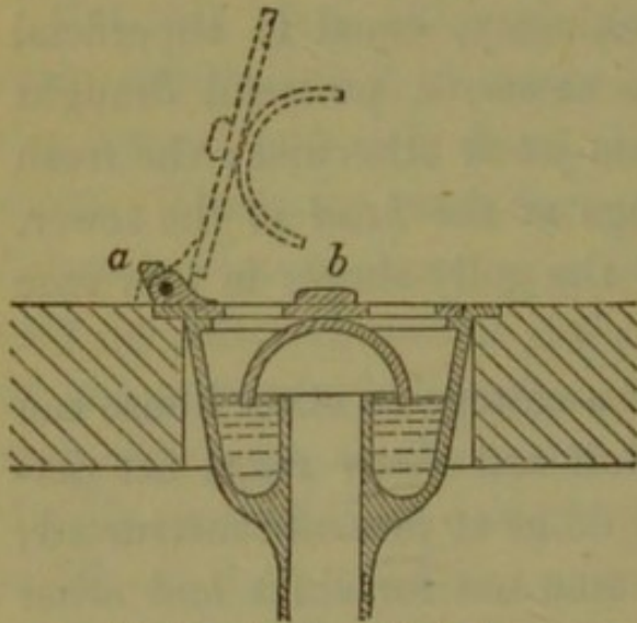
Fig. 6.—Section of bell-trap.
