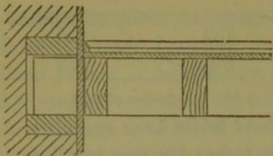
Fig. 24.—Section of girder floor.
