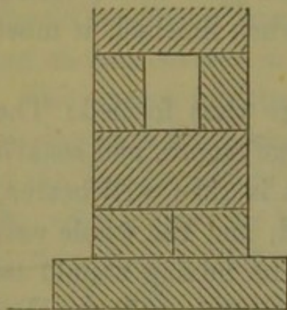
Fig. 9.—Section of Silverlock's hollow wall, 9 inches thick.
