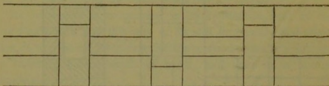
Fig. 15.—Hollow brick wall, 12 inches thick.
