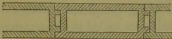
Fig. 17.—Plan of hollow brick partition.
