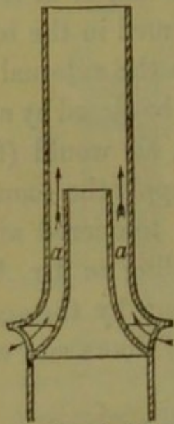
Fig. 35.—Section of chimney-funnel.
