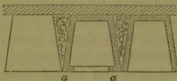
Fig. 19.—Section of a plaster floor.
