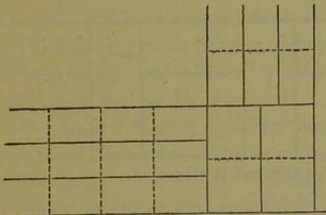
Fig. 11.—Plan of Dearn's hollow brick wall, 9 inches thick.
