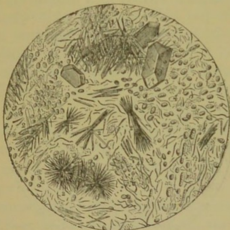
Fig. 54.—Wines affected by pousse . Deposit seen under the microscope : 1, ordinary alcoholic wine-ferment ; 2, acicular crystals of potassium bitartrate ; 3, crystals of normal calcium tartrate ; 4, Vibrio , or microbe which produces the disease.
