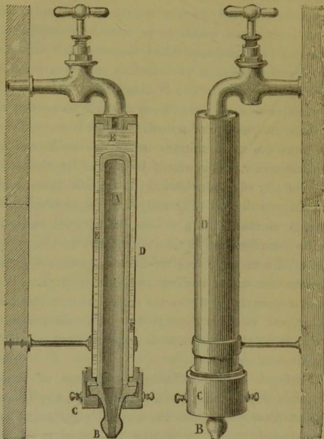
Fig. 101.—Section and elevation of Chamberland's filter.
