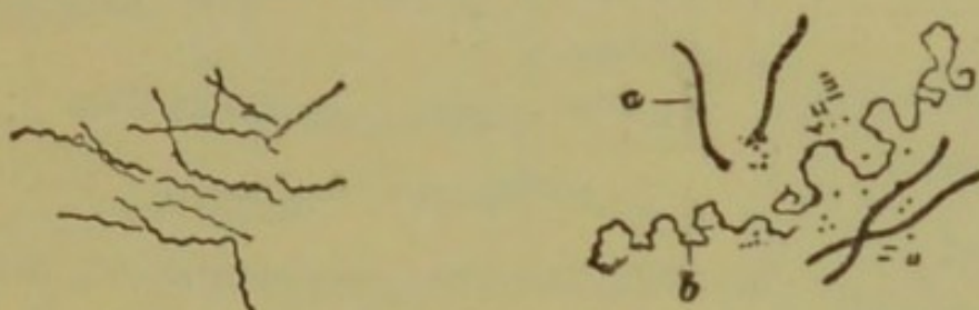
Figs. 77, 78.— Spirochæte buccalis , and S. plicatilis , b (mixed with Vibrio rugula , a ), microbes in mouth of a healthy man.
