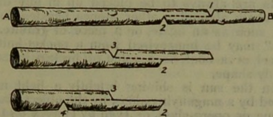
Fig. 94.—To cut up logs.
