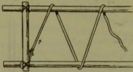
Fig. 26.—Unsatisfactory method of lashing rope for stretcher bed. Showing string and rope forming corner lashings.
