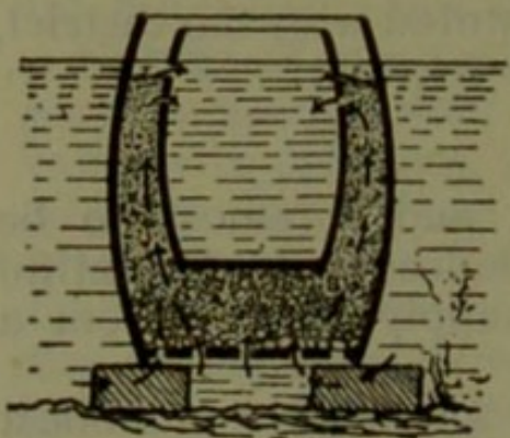
Fig. 71.—Barrel standing in a river bed.
