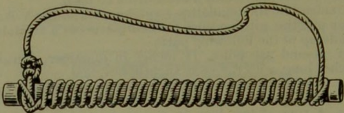
Fig. 24.—Improved transverse bar, showing method of twisting rope round the bar and making loop.
