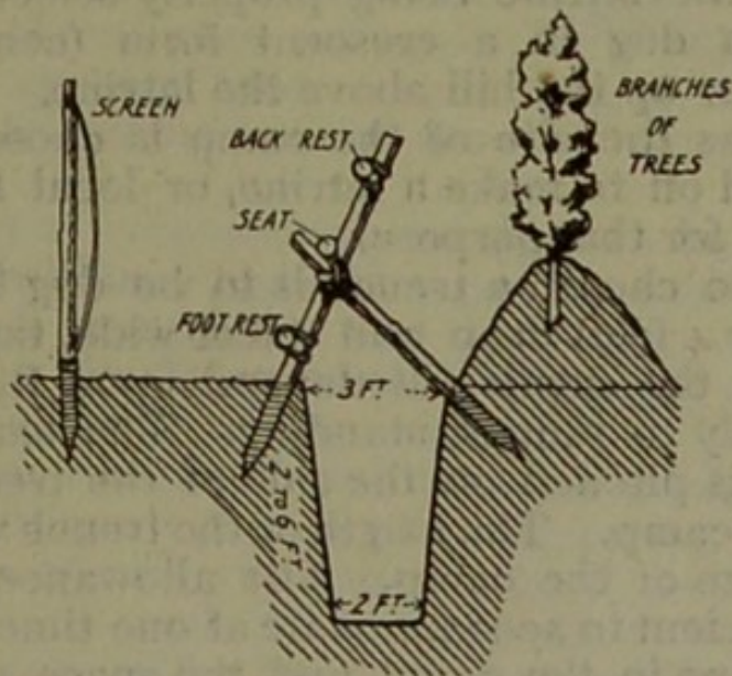
Fig. 80.—Front and section views of camp latrine. The dotted lines on poles indicate a screen.
