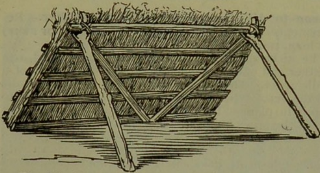
Fig. 98.—Lean-to hurdle-and-straw head shelter.
