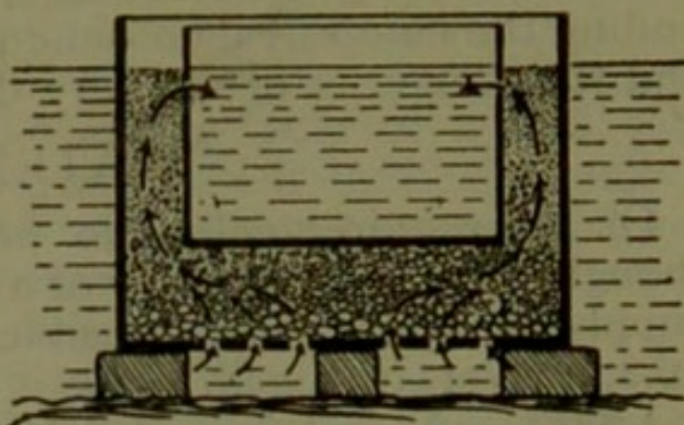
Fig. 72.—Boxes, one large and one smaller, with sand between, used in place of barrels.
