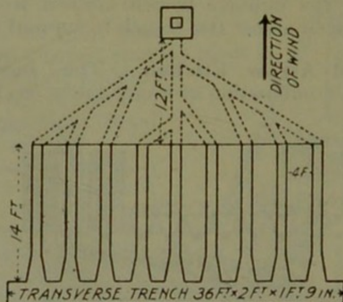
Fig. 90.—Gridiron kitchen on large scale.
