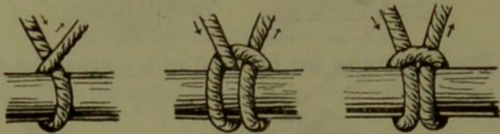
Fig. 33.—Different methods of fixing rope over poles, showing “simple turn,” “clove hitch,” and “double turn.”
