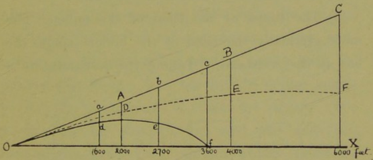
FIG. 1.—Trajectory in vacuo (dotted) and in air.
