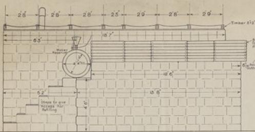
Rear View showing Both Room.
