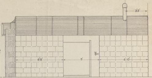
Front View looking S.W.
