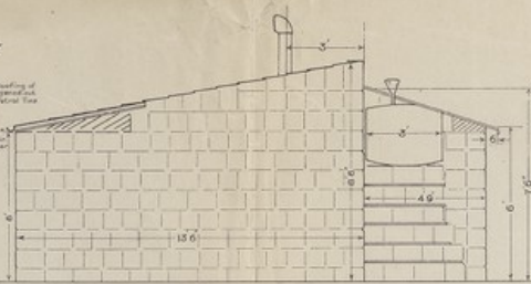
Side Elevation looking S.E.
