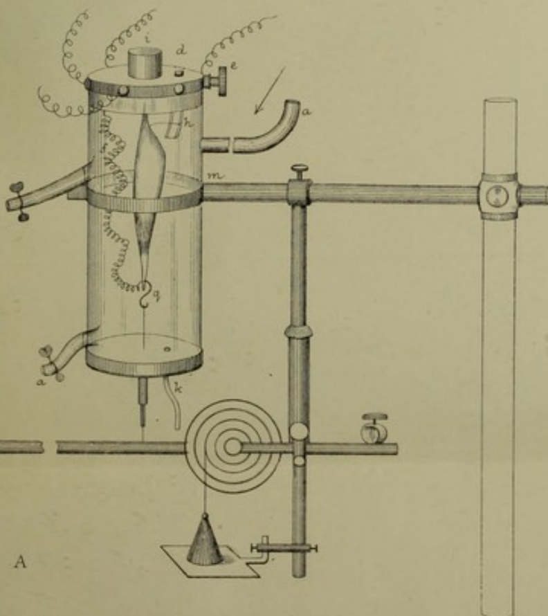
Drawing of closed Muscle Chamber. with Lever in connection. For explanation of Figures, see text
