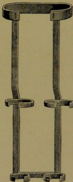
Fig. 33.—THE DOUBLE HIP SPLINT (RIDLON).
