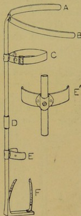
Fig. 24.—DIAGRAM OF CHEAP GAS-PIPE HIP SPLINT.
