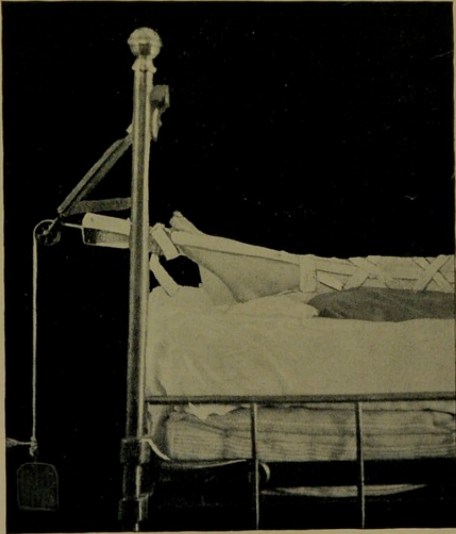
Fig. 15.—WEIGHT AND PULLEY APPARATUS FOR BED TRACTION.
