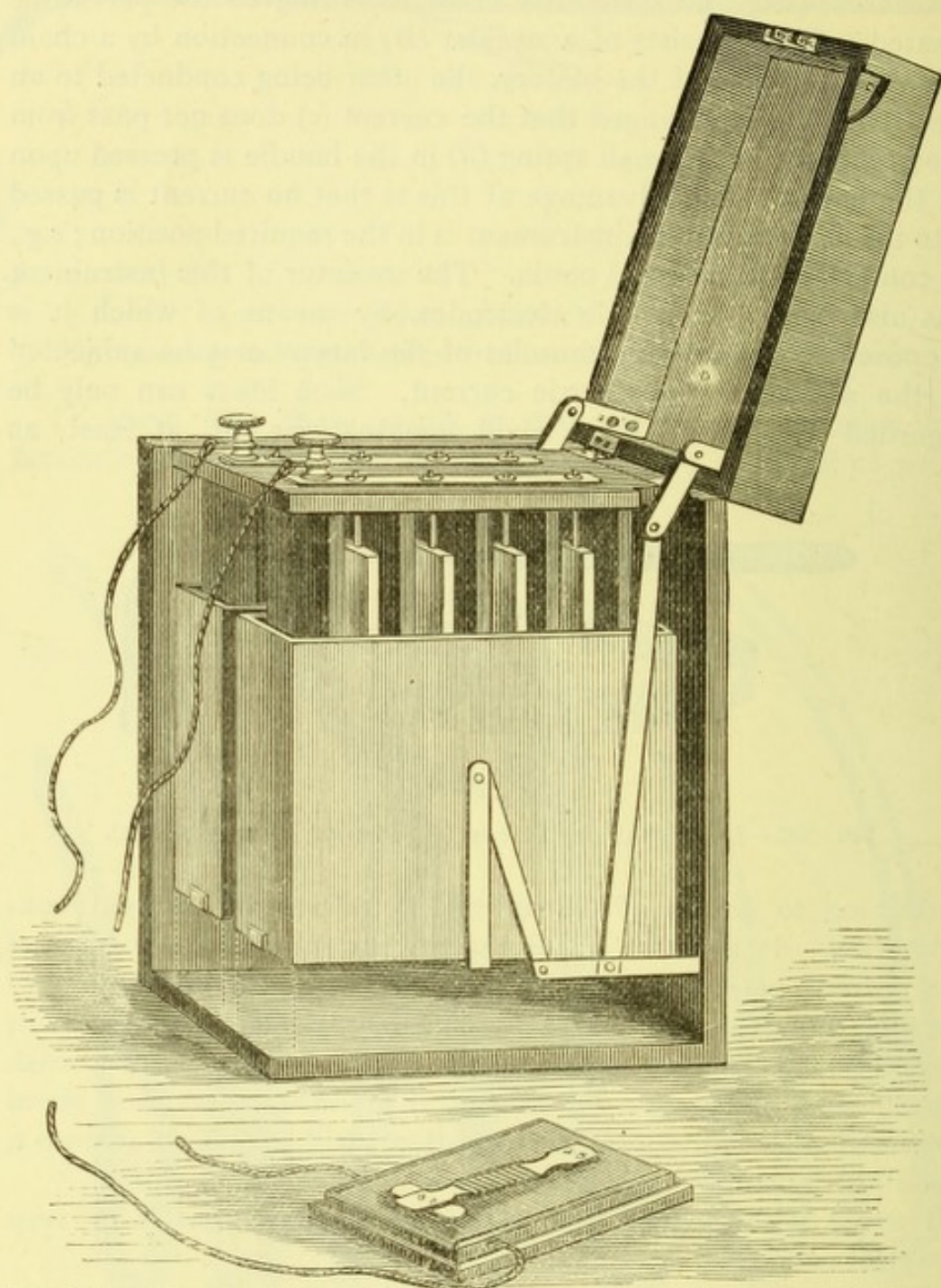
FIG. XCI.—AUTHOR'S GALVANO-CAUSTIC BATTERY, WITH FOOT-PIECE (MAYER).
