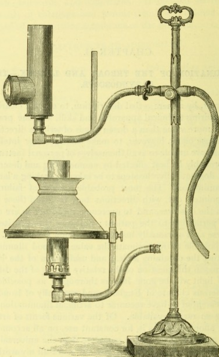
FIG. XIX.—A CONVENIENT STANDARD GAS LAMP, WITH ARGAND BURNER, WHICH CAN BE ATTACHED TO ANY GAS-JET, AND CAN BE USED FOR VARIOUS PURPOSES.
