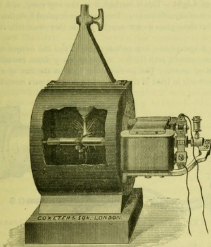
FIG. XXI.—COXETER'S WATER-WHEEL MOTOR.
