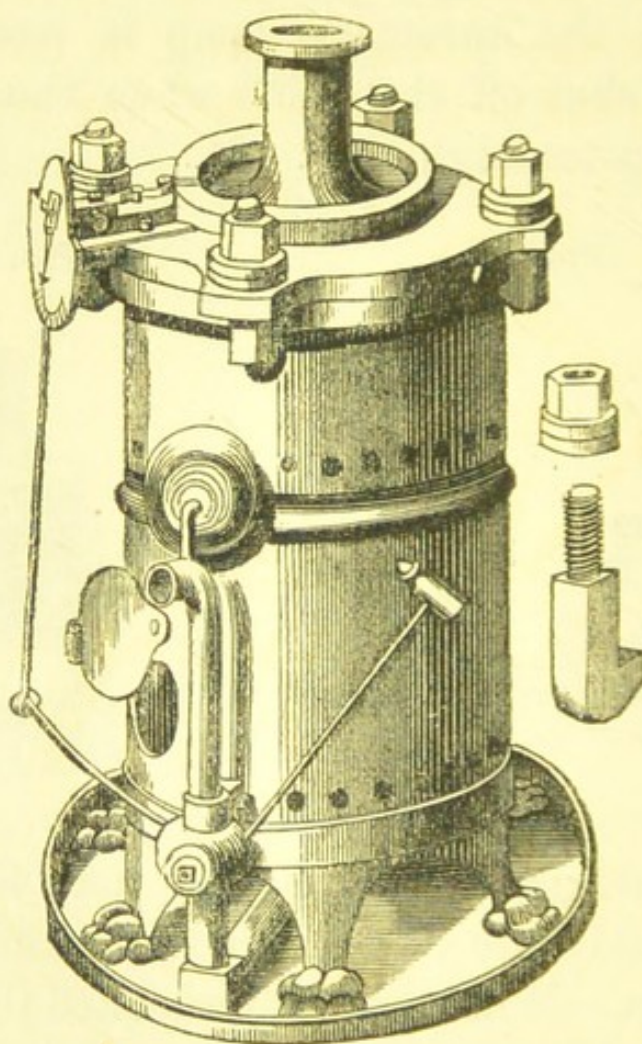
Vulcanizer.
