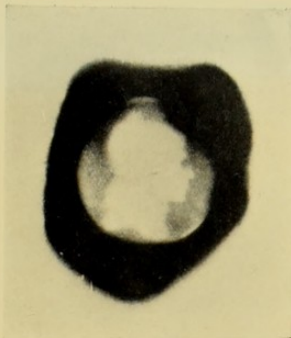
FIG. 1. Becquerel's Uranium Picture.
