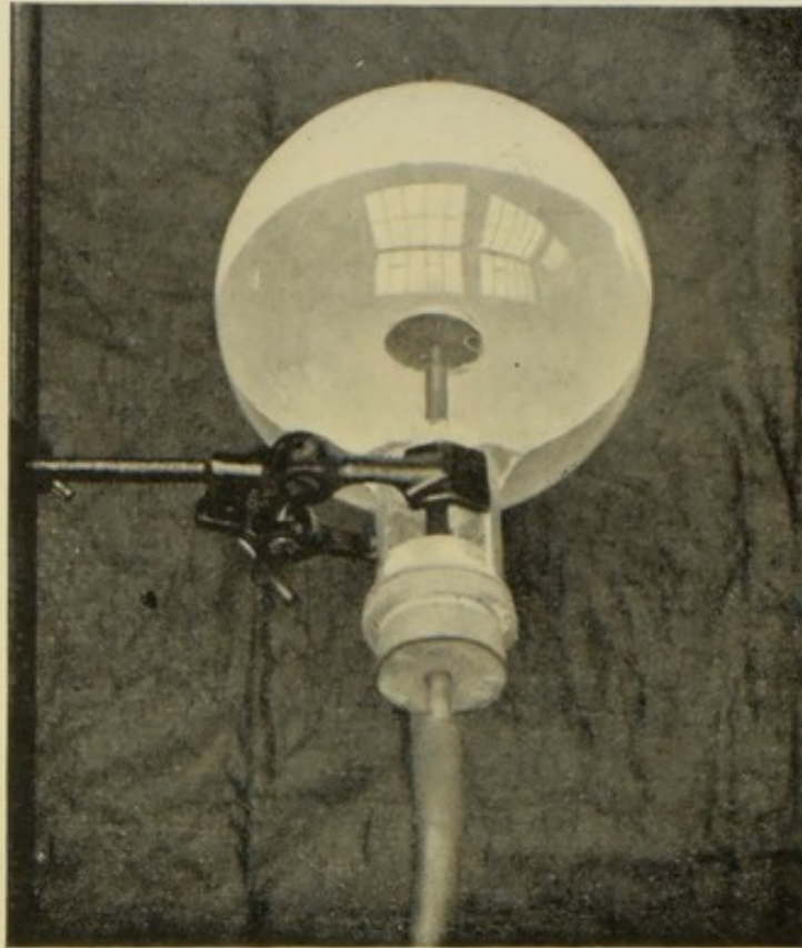
FIG. 9. Apparatus to show Absorption of \alpha -Rays by Air.
