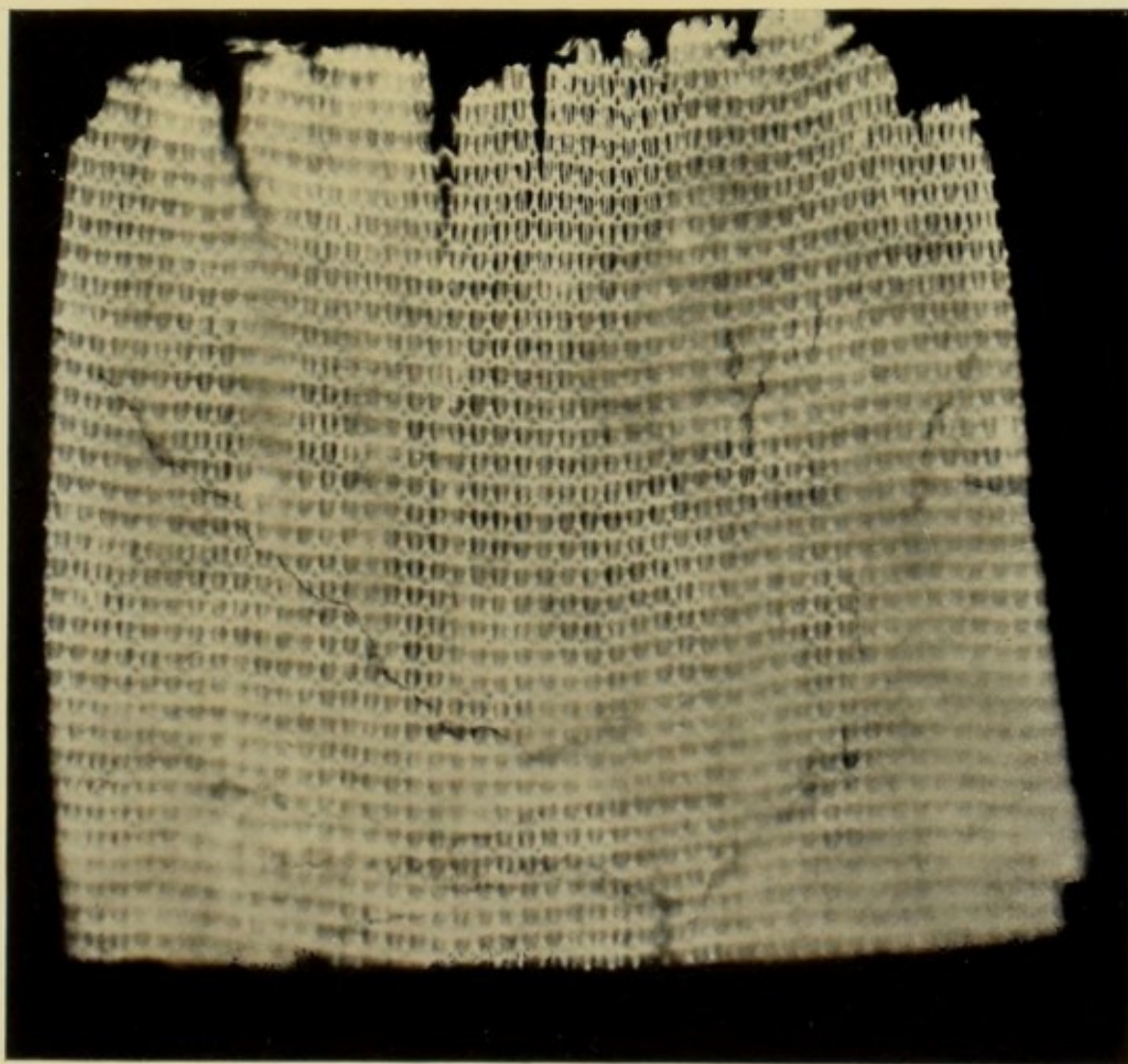
FIG. 2. Welsbach Mantle imprinted by its own rays.
