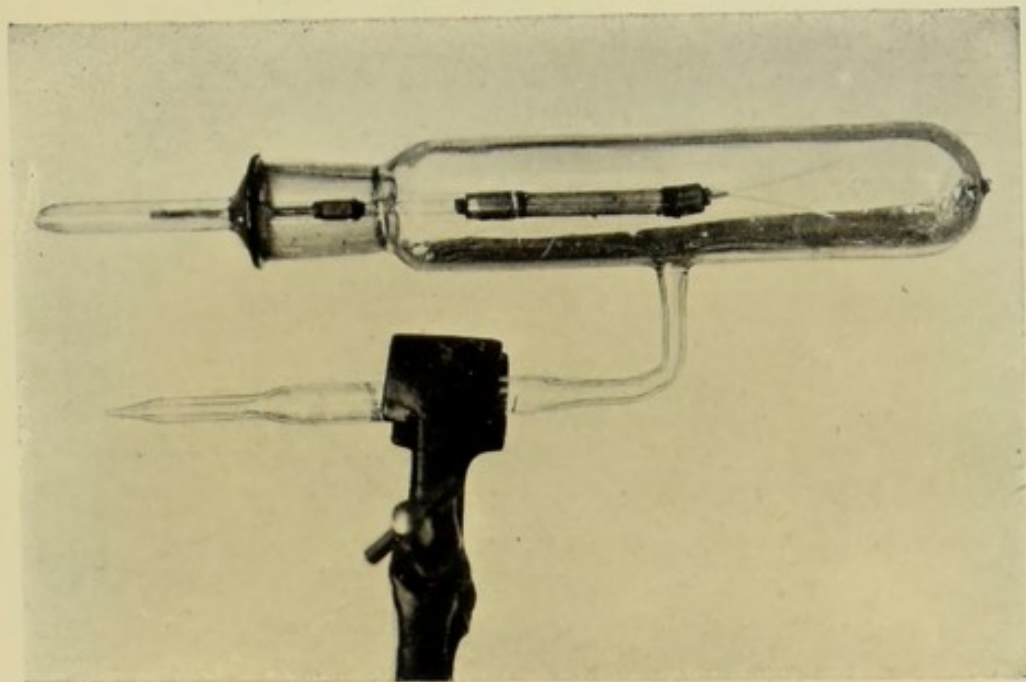
FIG. 16. Professor Strutt's "Radium Clock."
