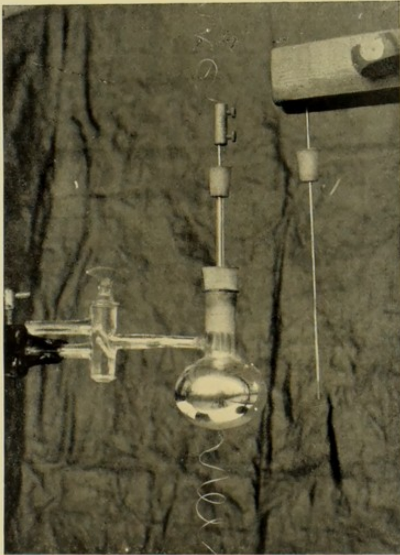
FIG. 29. Apparatus for obtaining the Active Deposit of Radium.
