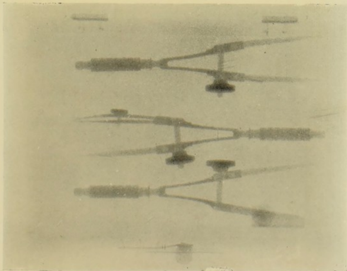
FIG. 7. Closed Box of Compasses taken with the \gamma -Rays of Radium.
