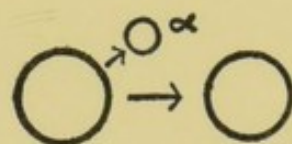
Radium. Emanation.
