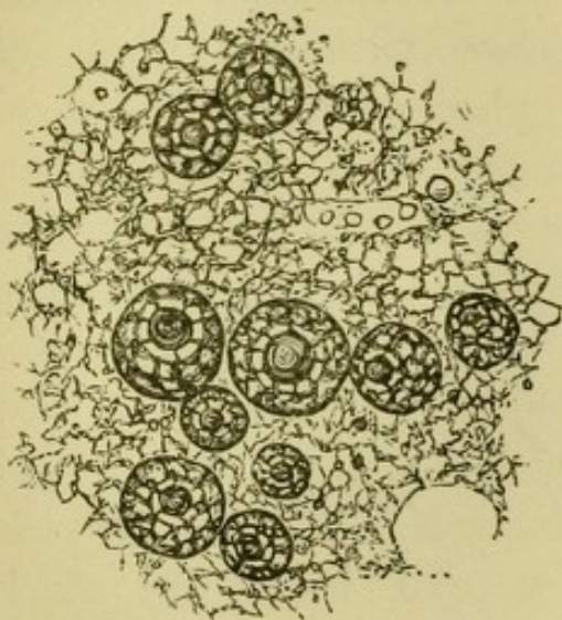
FIG. 113.— Badhamia utricularis ; portion of plasmodium, showing a number of spherical nuclei, in each of which the fibrillar network and the nucleolus is seen. Magnified 1200. (From Lister's Monograph of the Mycetozoa.)
