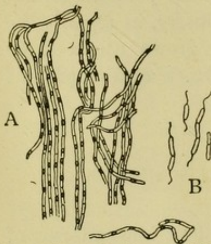
FIG. 109.— Bacillus subtilis . A, cells cohering in filaments; the dark bodies are spores. B, swarming ciliated cells produced on germination of the spores. Magnified 800. (After Strasburger.)
