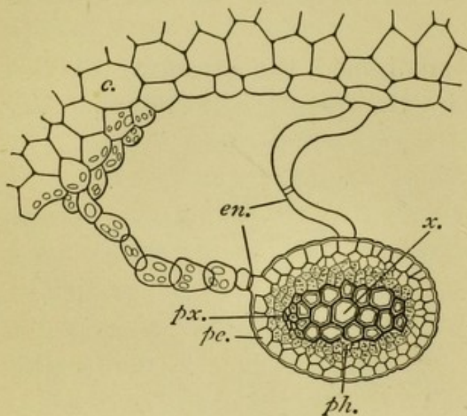
FIG. 8. — Selaginella Kraussiana ; part of transverse section of stem showing one stele. x , the wood; px , protoxylem; ph , phloëm; pc , pericycle; en , endodermal cells forming the whole or part of trabeculæ; c , inner layers of cortex. Magnified about 100 diameters. (After Harvey Gibson.)
