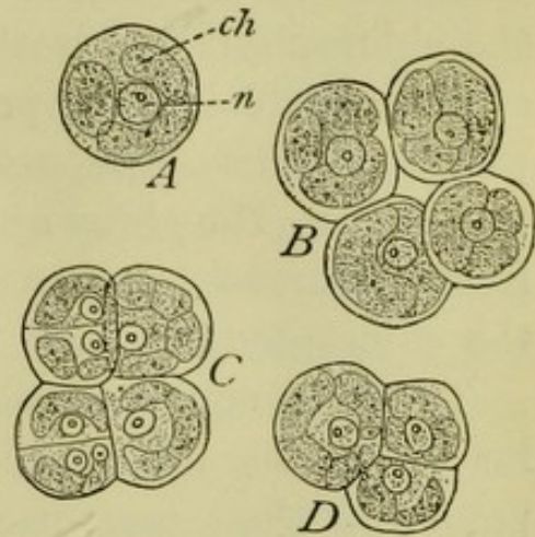
FIG. 77.— Pleurococcus vulgaris . A , single cell; n , nucleus; ch , chloroplastids. B , four cells separating after division. C , group of cells remaining in contact. The two to the left have just divided afresh. D , tetrahedral group. Magnified 540. (After Strasburger.)
