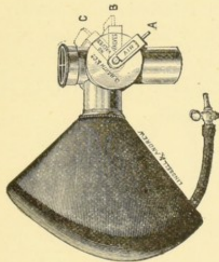
FIG. 12.—Barth's improved face-piece and three-way tube.
