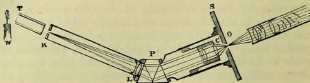
Fig. 69.—Sectional view of the Browning Spectroscope.
