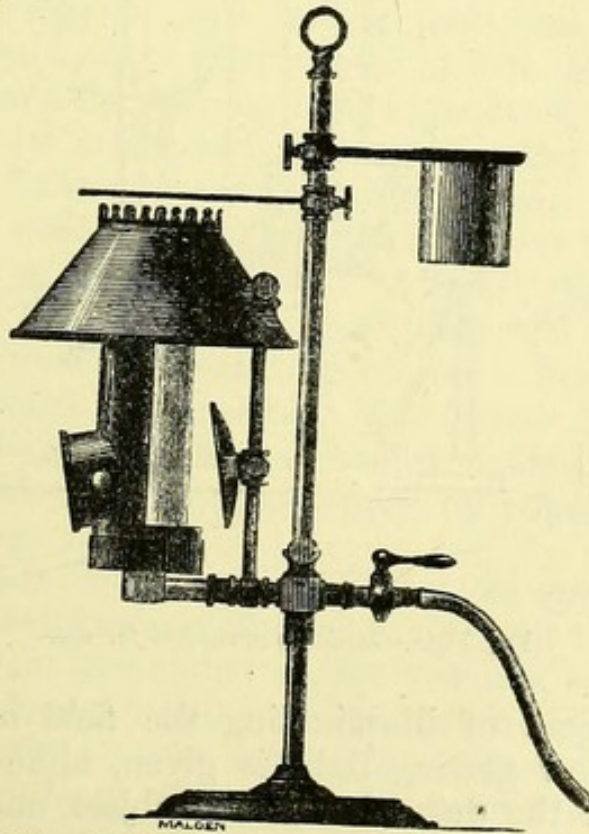
Fig. 109.— Highley's Gas-lamp, with Steam-bath attached.
