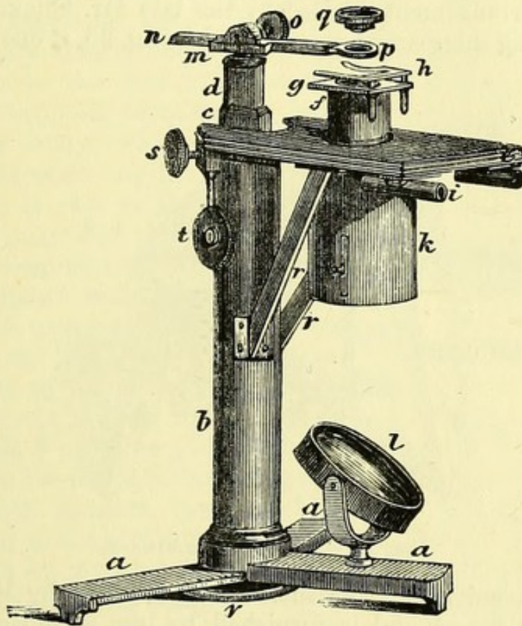
Fig. 24.— Valentine's Microscope.
