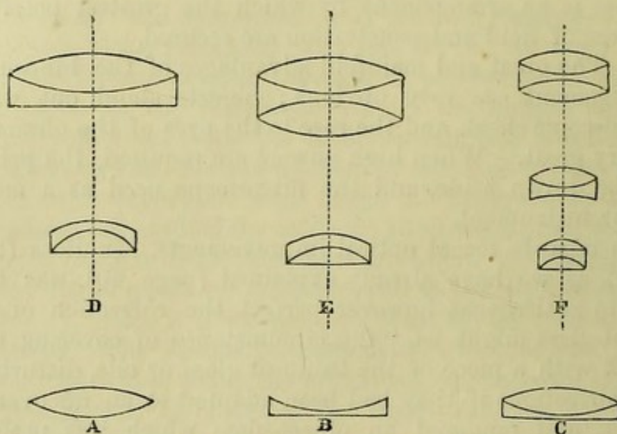
Fig. 38.—Forms of Object-glasses.
