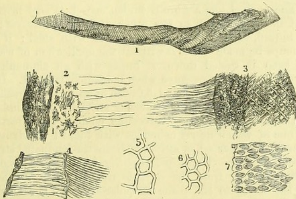
Fig. 342. — Tooth Structure.
