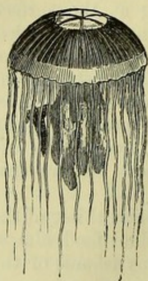
Fig. 238.—Jelly-fish.
