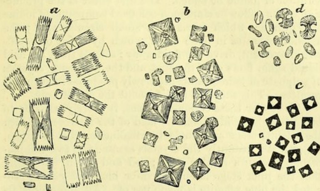
Fig. 91.— Urinary Salts.
