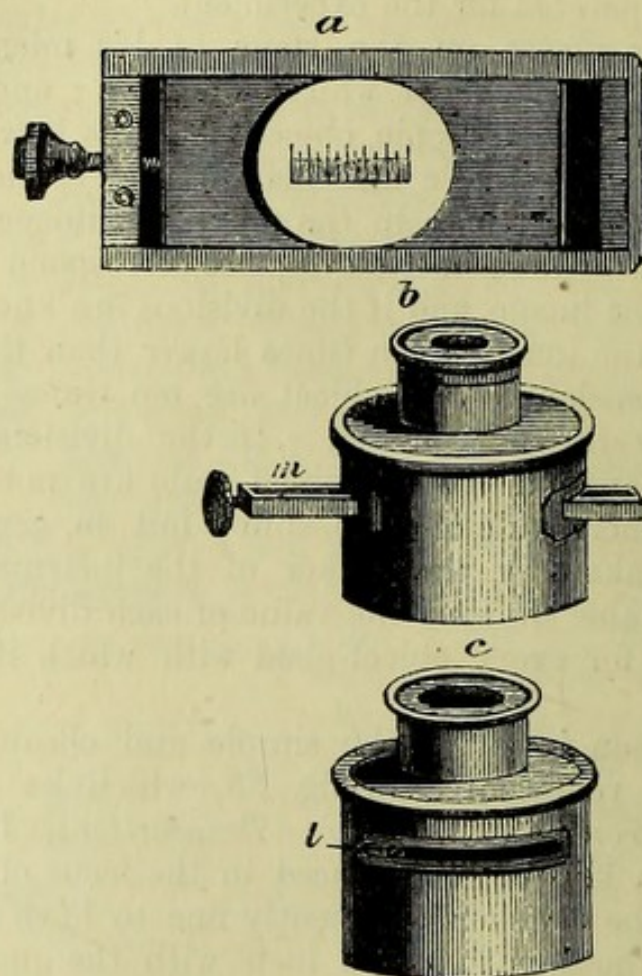
Fig. 35.—Mr. Jackson's Micrometer eye-piece.
