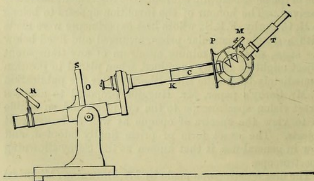
Fig. 70.—The Browning Huggins' Micro-spectroscope.
