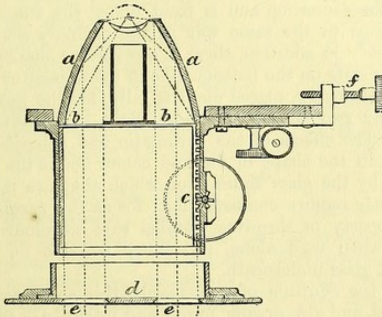
Fig. 104.—Wenham's Parabolic Reflector.
