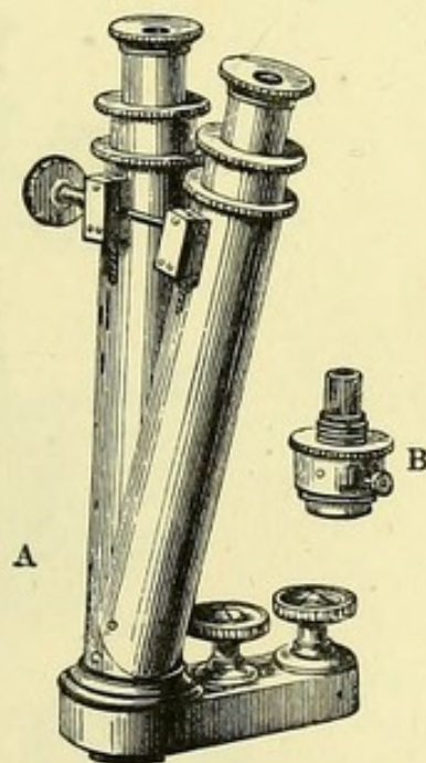
Fig. 45.—Baker's arrangement of Wenham's Binocular.
