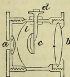
Fig. 2. Lieberkuhn's Micro- scope.
