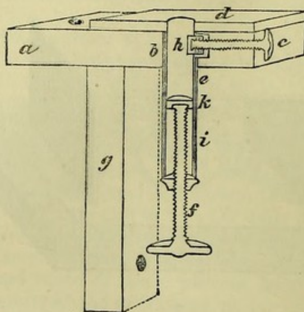
Fig. 133.— Topping's Section Cutting Machine.
