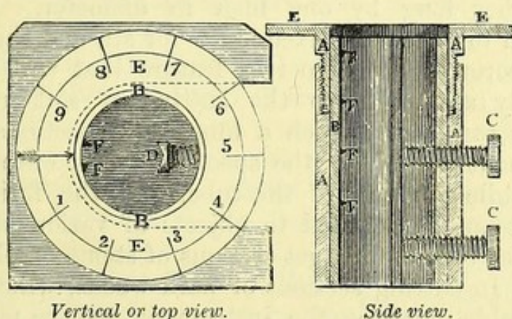
Fig. 131.—Smith's Section Instrument.
