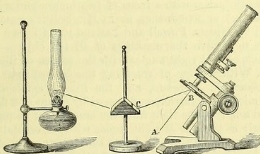
Fig. 102 — Sollitt's Single-Prism Illumination.
