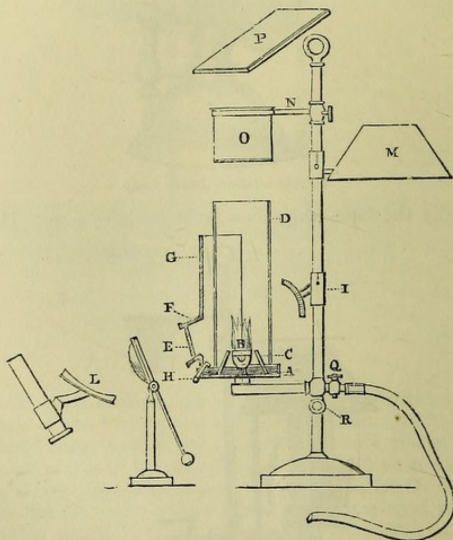
Fig. 110.—Gas-lamp arranged for use.
