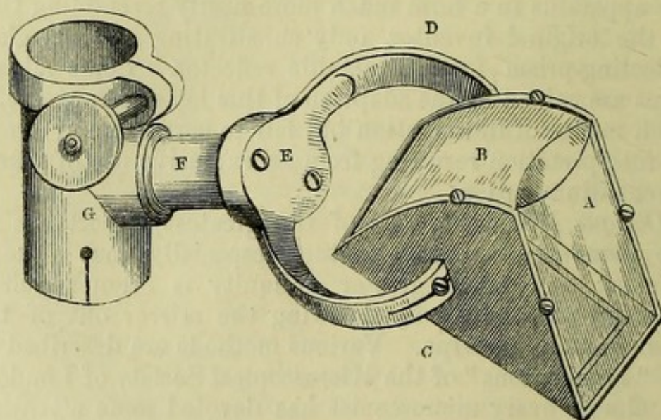
Fig. 101.— Abraham's Achromatic Lenticular Prism. Half-size.
