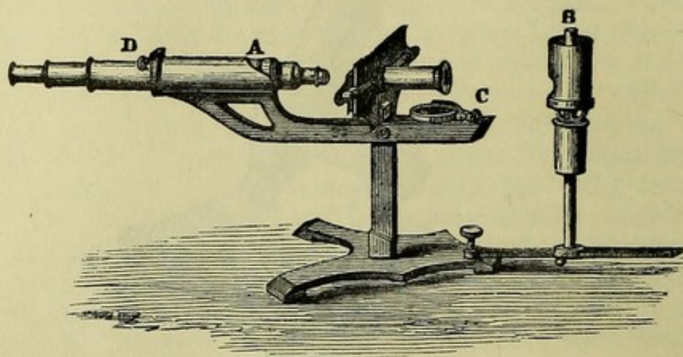
Fig. 58.— Murray and Heath's Class Microscope.
