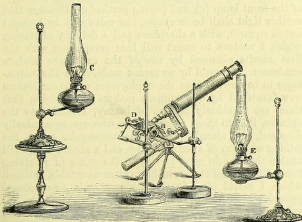
Fig. 103.—Mr. Newton Tomkins' Double Prism Illumination.
