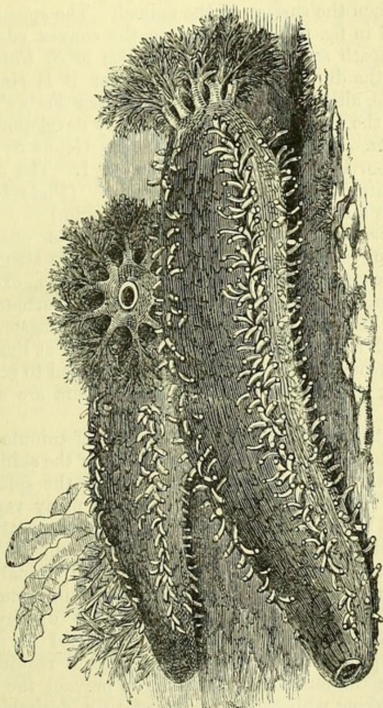
Fig. 242.— Holothuridea , Sea-cucumbers.
