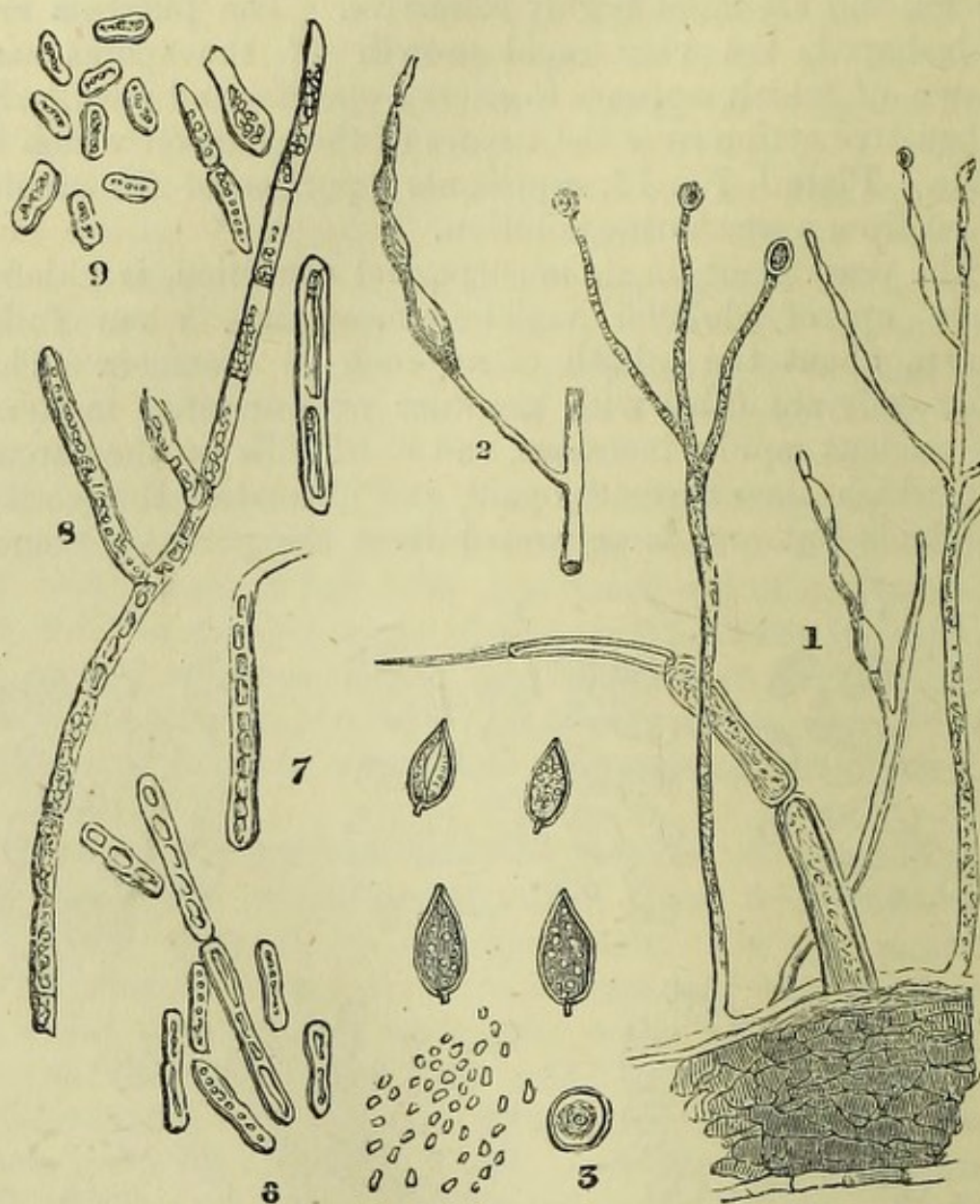
Fig. 160.—Fungoid growths.
