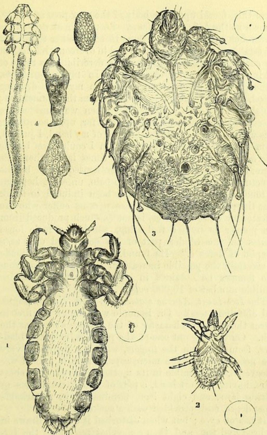
Fig. 290.—Parasites. Acarina .
