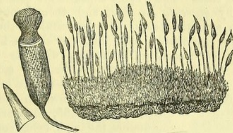
Fig. 163.—Screw Moss.
