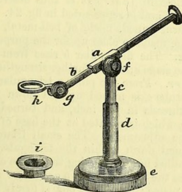
Fig. 23.—Ross's Simple Microscope.
