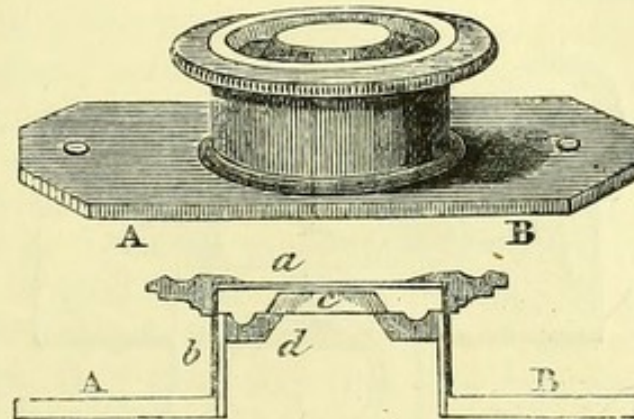
Fig. 121.—Varley's Animalcule-cage.
