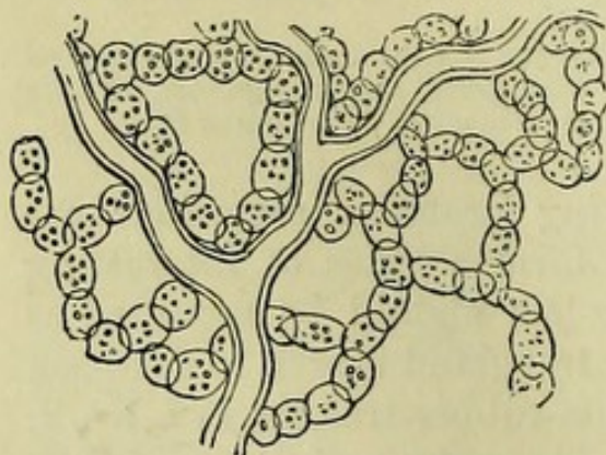
Fig. 178. —Lactiferous tissue.
