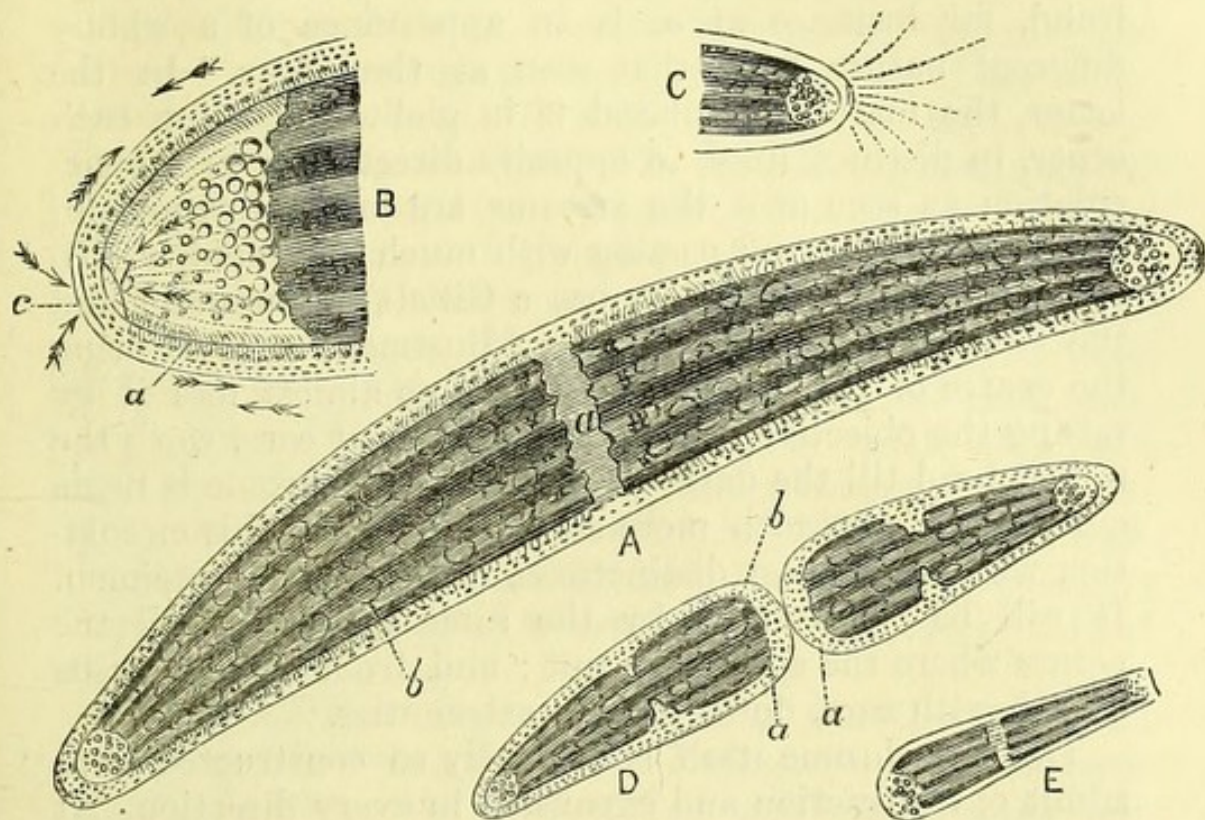
Fig. 156 — Closteria Lunula .
