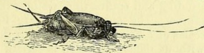
Fig. 285.—The Cricket.
