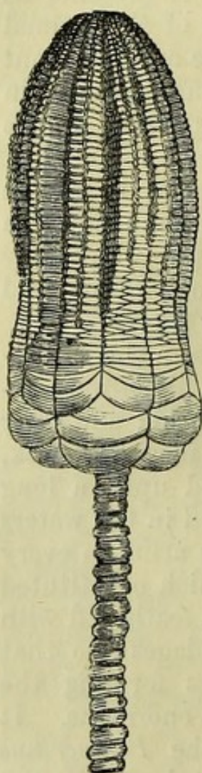
Fig. 241.— Encrinurus , Sea-lily.
