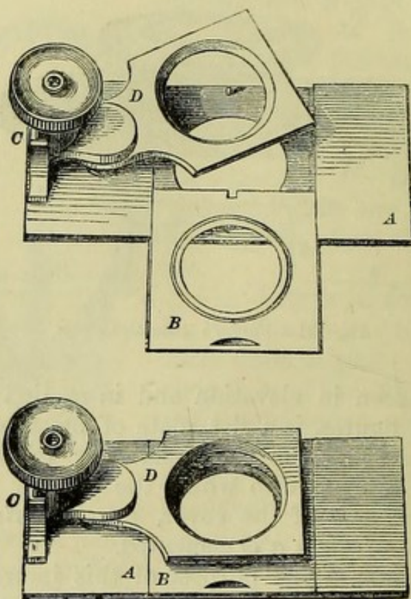
Fig. 122.—Ross's Compressorium.
