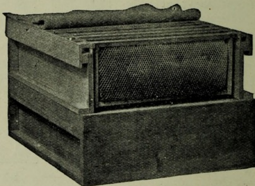
Fig. 41.—Surplus-boxes of Shallow Frames.
