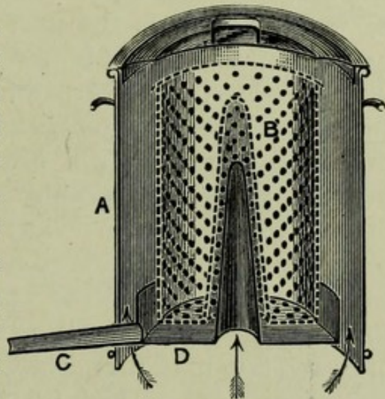
Fig. 63.—Gerster's Wax-extractor.
