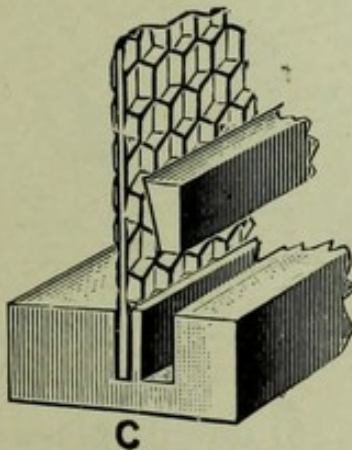
Fig. 51.—Wedge-piece for Securing Foundation.
