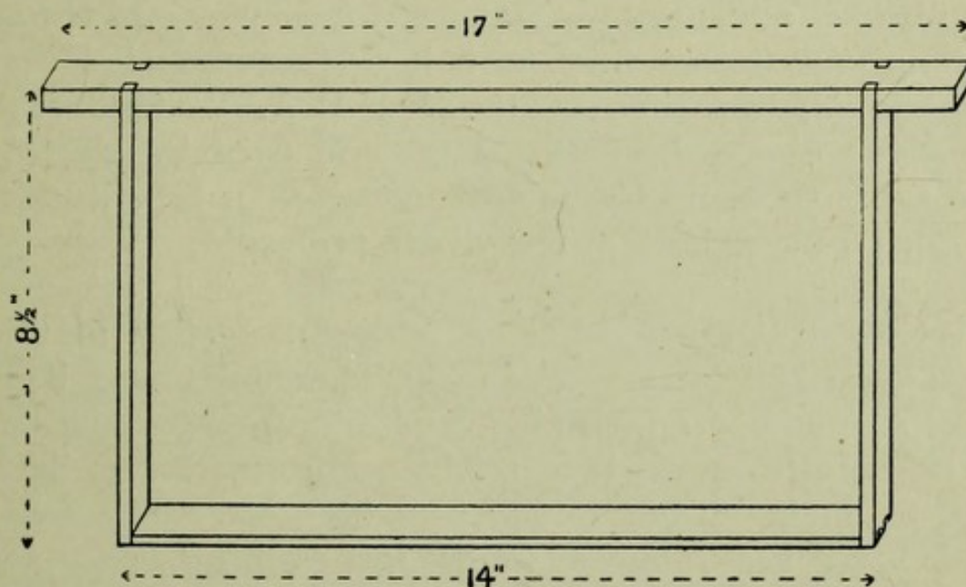
Fig. 21.—British Bee-keepers' Association Standard Frame.
