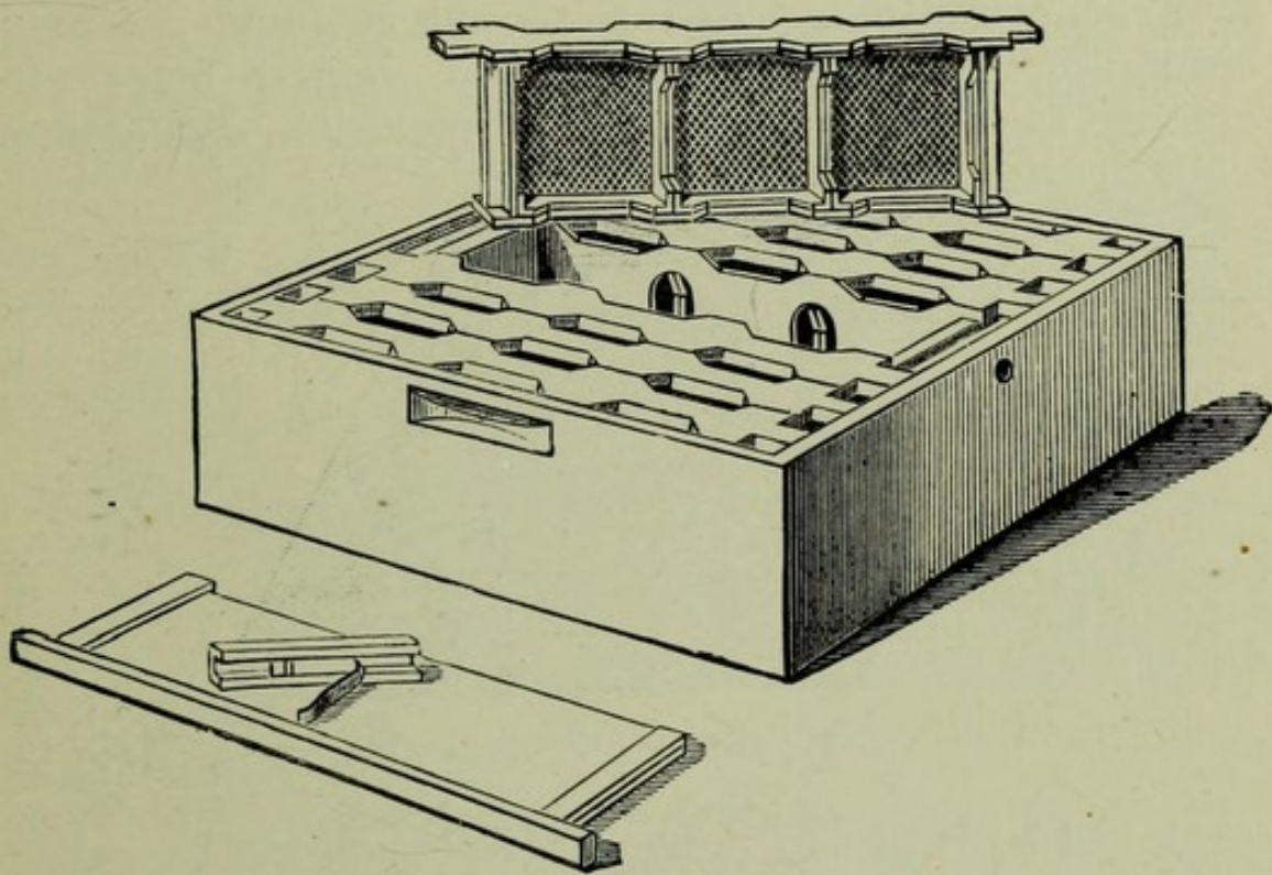
Fig. 35.—“W.B.C.” Section-rack.
