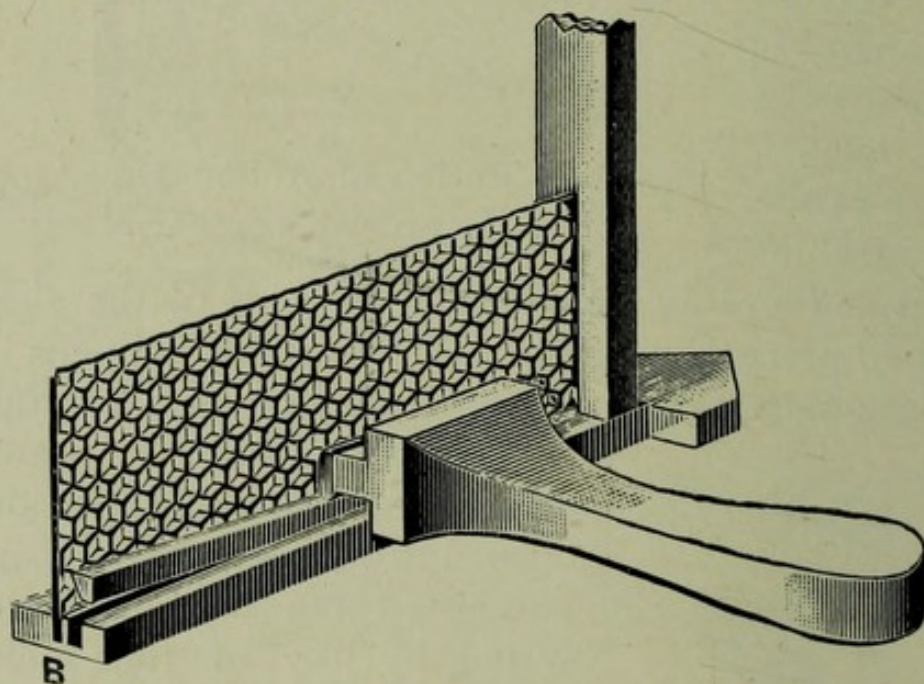
Fig. 52.—Lever for Forcing Wedge Home.
