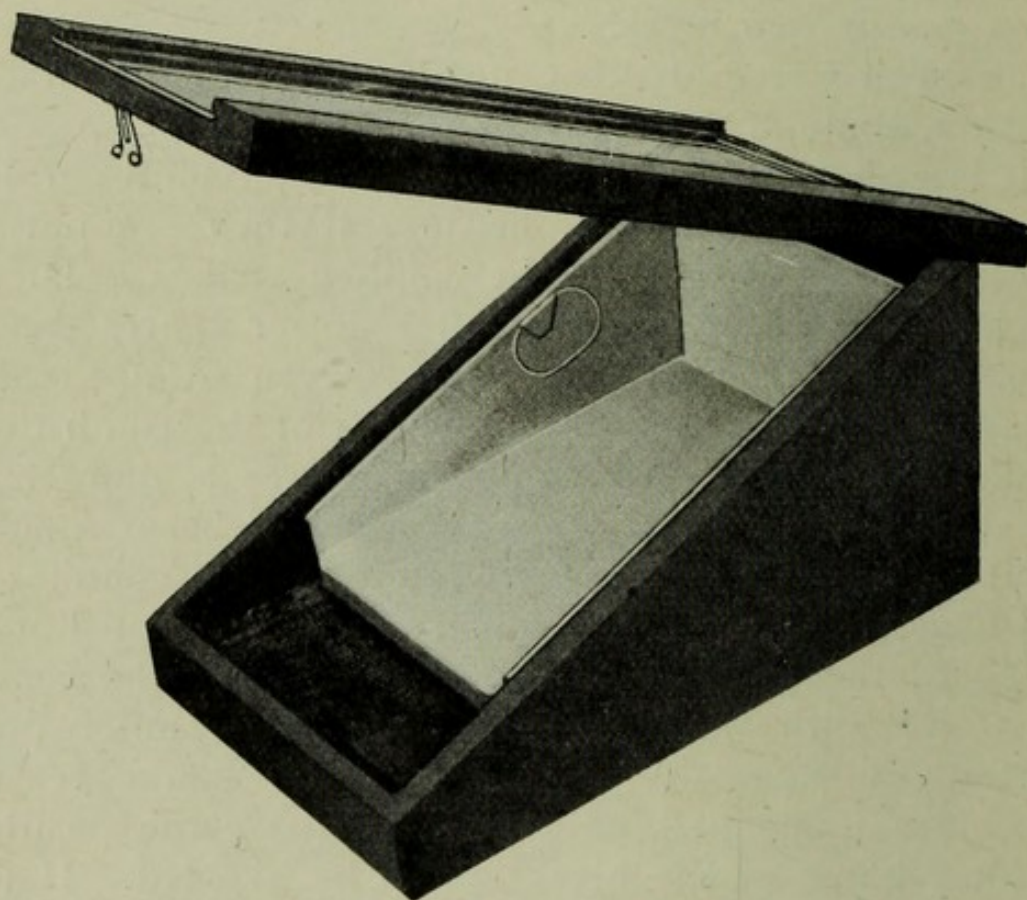
Fig. 62.—Solar Wax-extractor.
