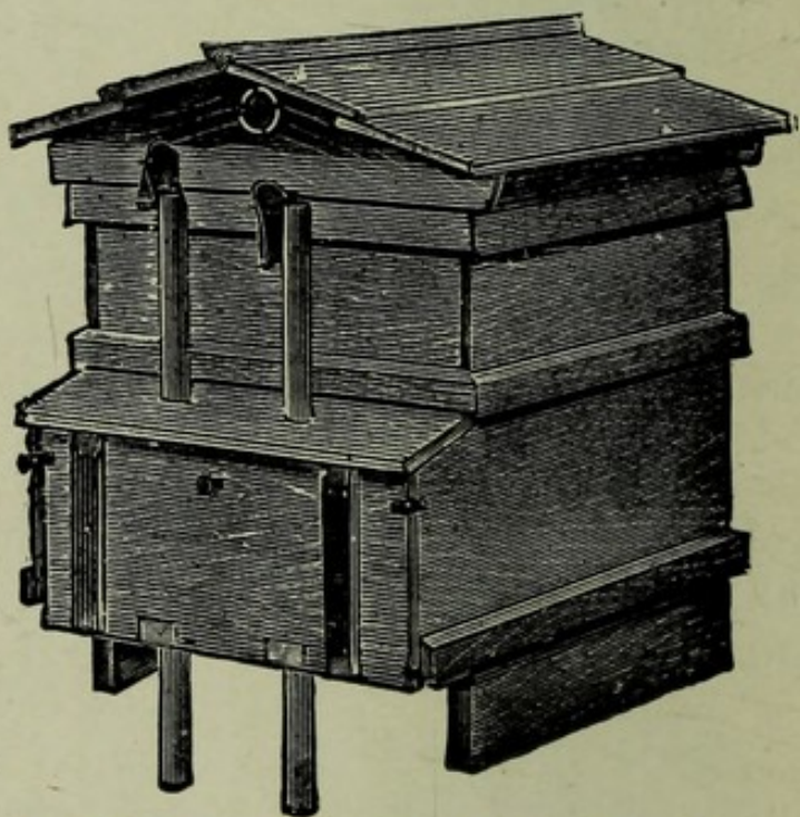
Fig. 29.—Claustral Hive, with Ventilating Chimneys, alighting-board closed.
