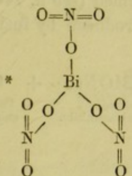
Bismuthous nitrate.
