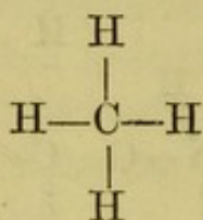
Marsh-gas.
