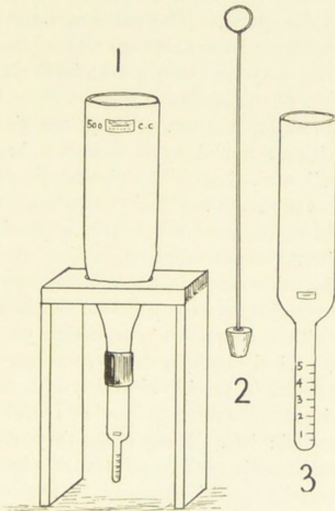
FIG. 48.—Apparatus for estimation of sediment in milk.
