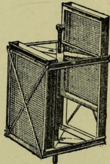
Fig. 56.—Revolving Cage of “Cowan” Extractor.
