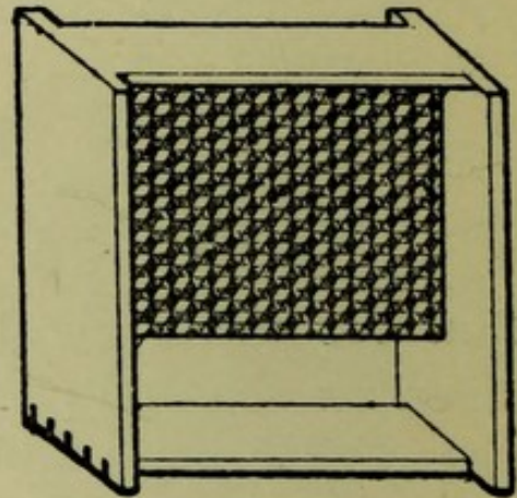
Fig. 48.—Section with Foundation fixed.
