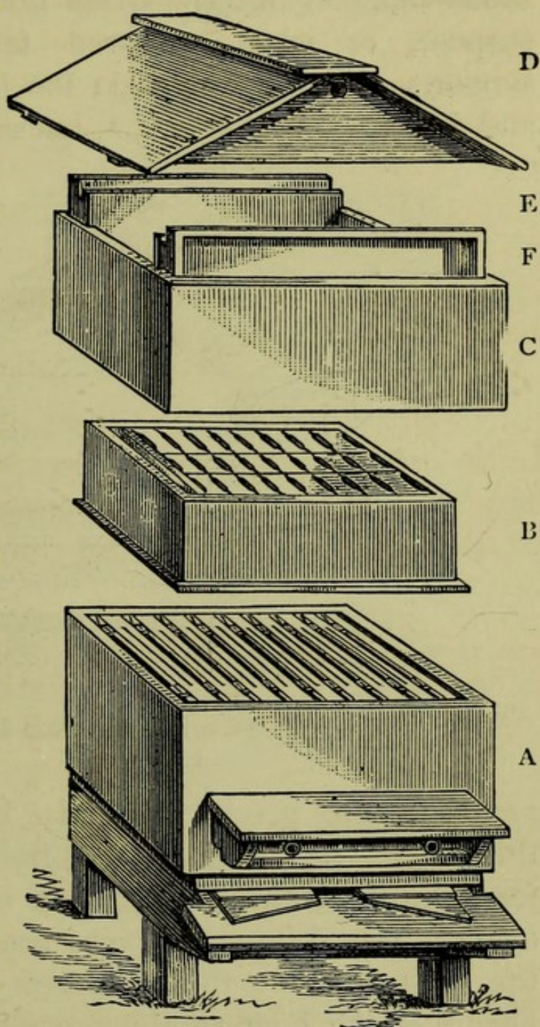
Fig. 17.—Neighbour's Sandringham Hive.
