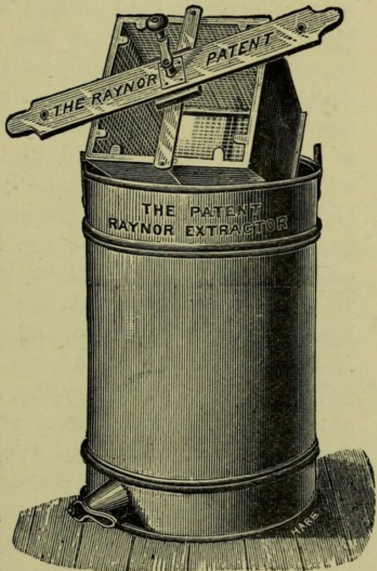
Fig. 58.—Meadows' "Raynor" Extractor.
