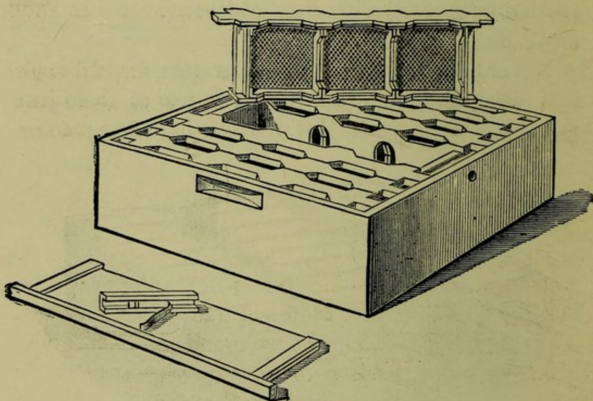
Fig. 30.—"W. B. C." Section-rack.
