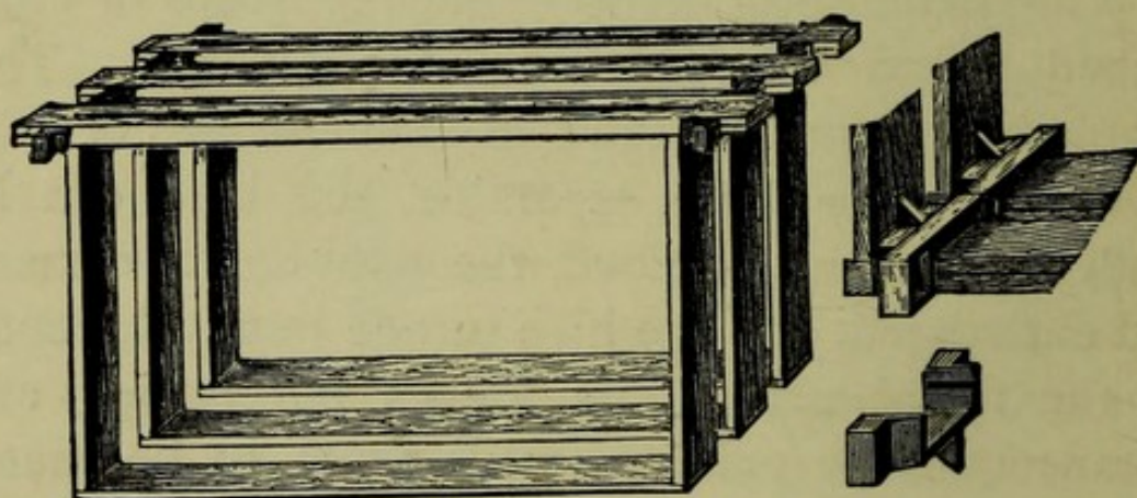
Fig. 16.—Frames and Metal Ends.
